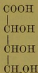
Erythroglicic acid.
