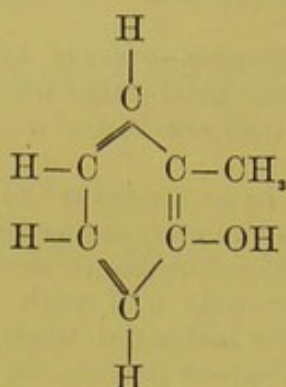
Benzyl phenol.
