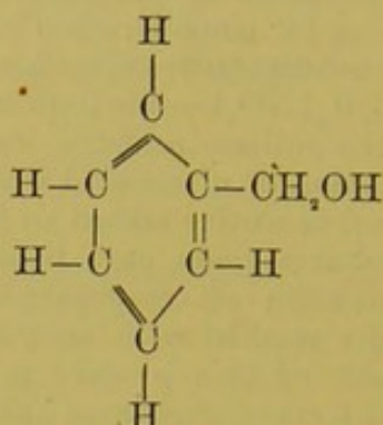
Benzyl alcohol.
