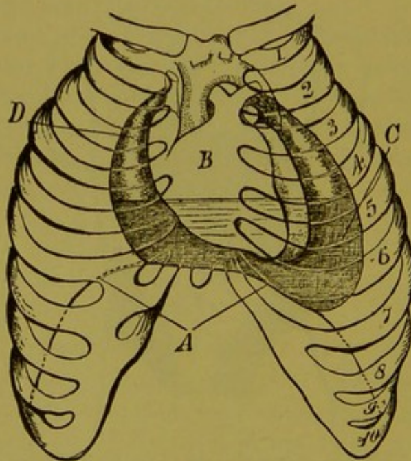
FIG. 78.—Hydropericardium.
