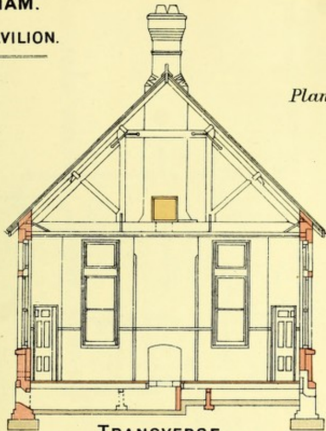
TRANSVERSE SECTION ON LINE A.A.
