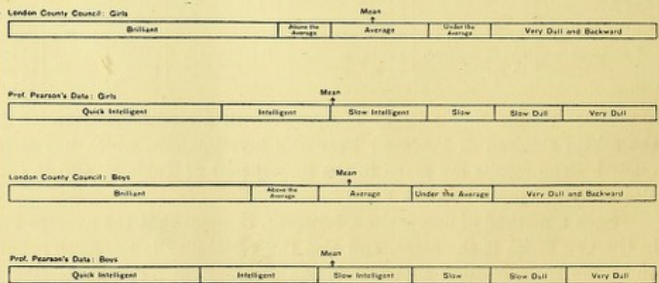
FIG. 3. RELATIVE SCALES OF INTELLIGENCE WITH L.C.C. GROUP "AVERAGE" AND PEARSON'S "SLOW AGE" AS EQUIVALENTS
