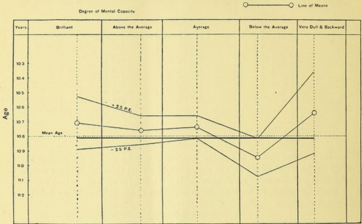
FIG. 6. DIAGRAMS TO SHOW THAT, WITHIN THE LIMITS OF PROBABLE ERRORS, THERE IS NO RELATIONSHIP BETWEEN AGE AND MENTAL CAPACITY.
