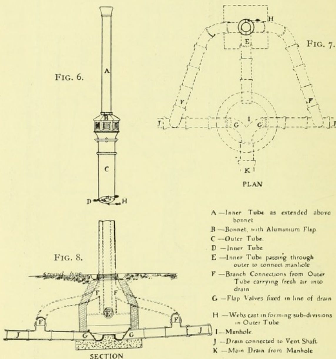
THE "OMNIFEX" SYSTEM OF SEWER VENTILATION.
