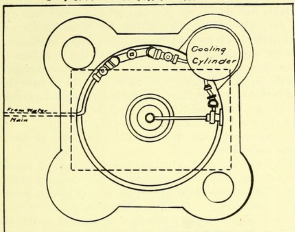
Plan on line A.A. Fig 21
