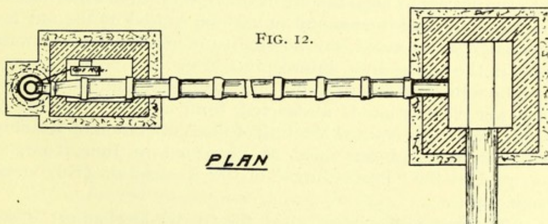
WEBB'S SEWER VENTILATING LAMP, BLACKPOOL.
