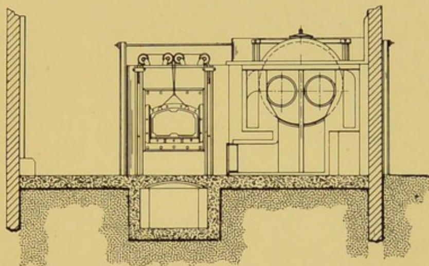
FIG. 66. GRAYS COMBINED DESTRUCTOR AND ELECTRICITY WORKS. Sectional Elevation.
