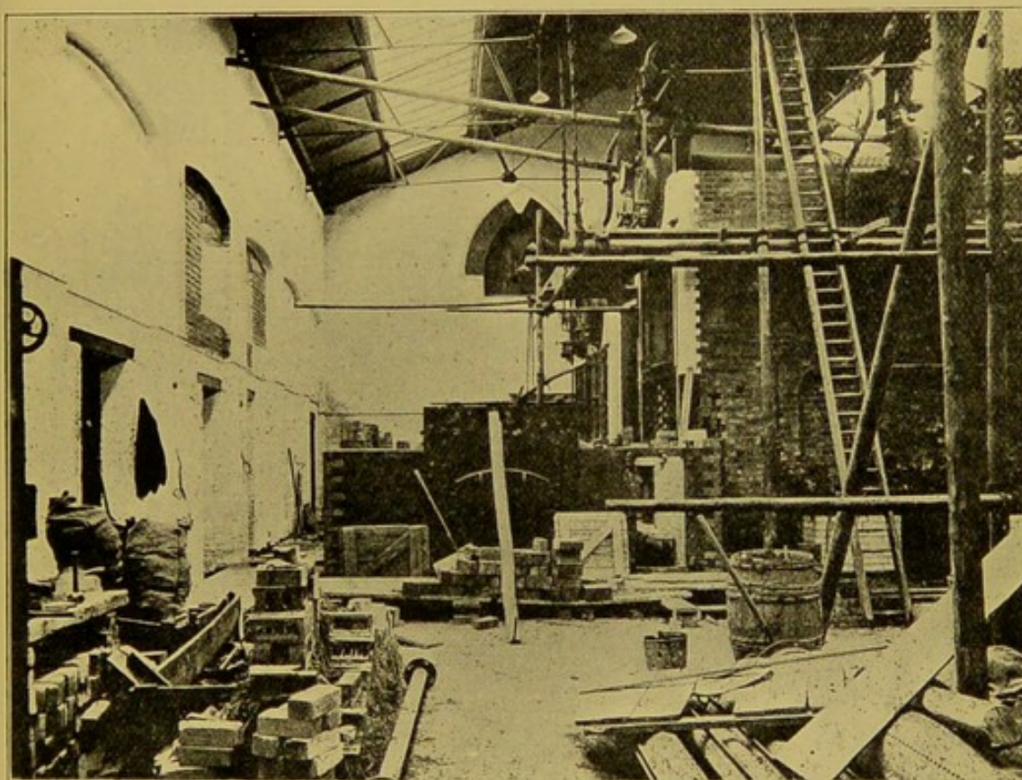
FIG. 90. WIMBLEDON COMBINED DESTRUCTOR AND SEWAGE WORKS. View of Cells in Course of Erection.
