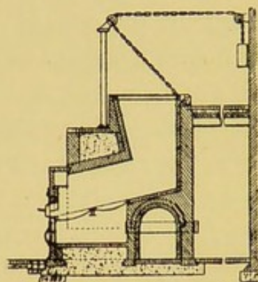
FIG. 23. WARNER'S DESTRUCTOR, DIRECT CHARGED TYPE.
