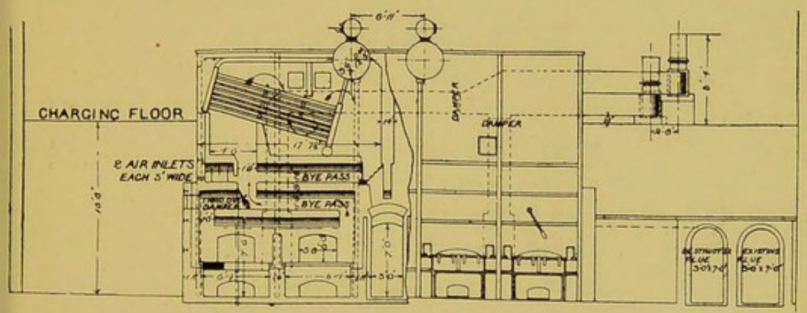
FIG. 30. HEENAN'S TWIN-CELL DESTRUCTOR.
