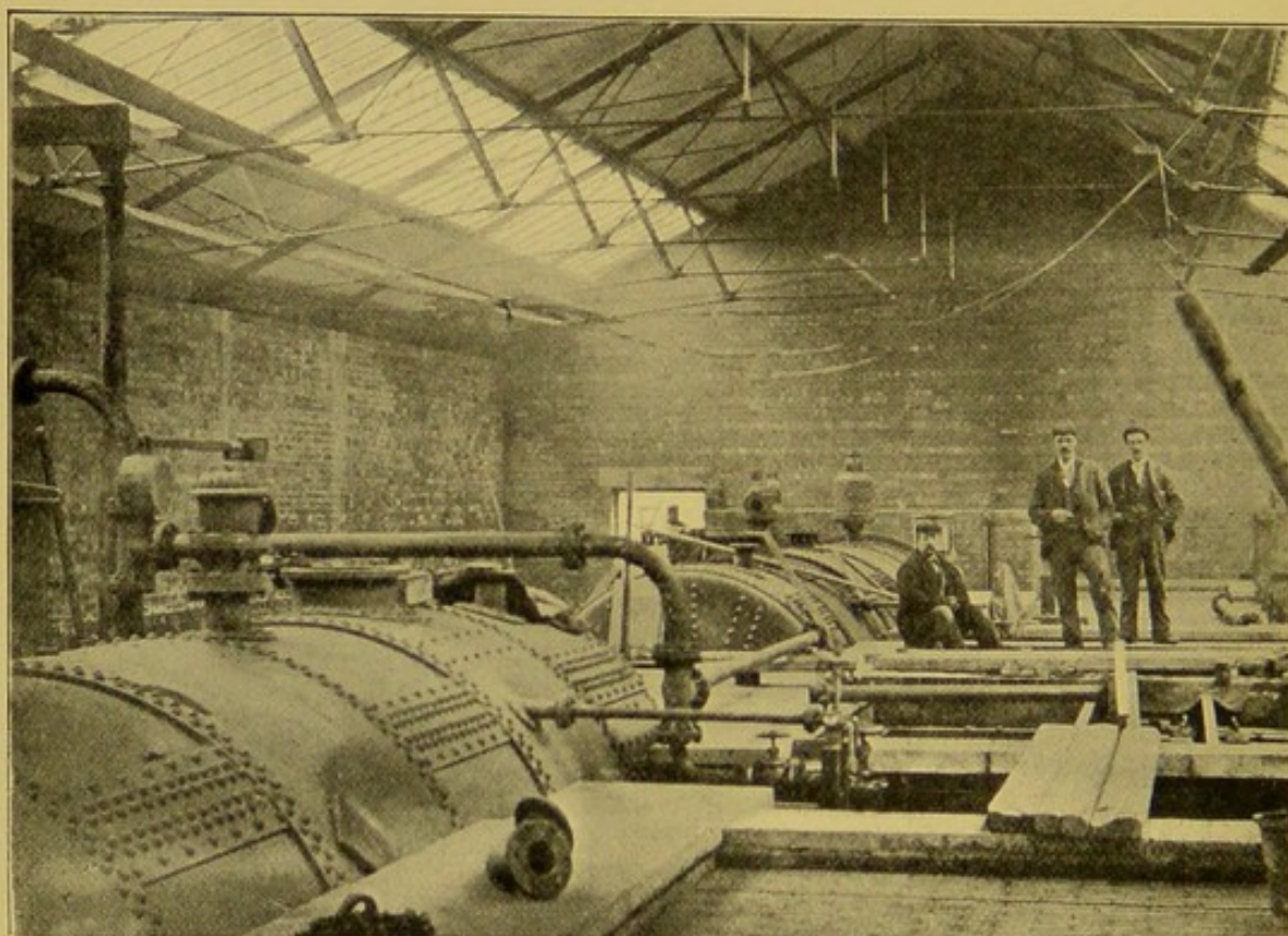
FIG. 71. LANCASTER COMBINED DESTRUCTOR AND ELECTRICITY WORKS. View of Boilers.
