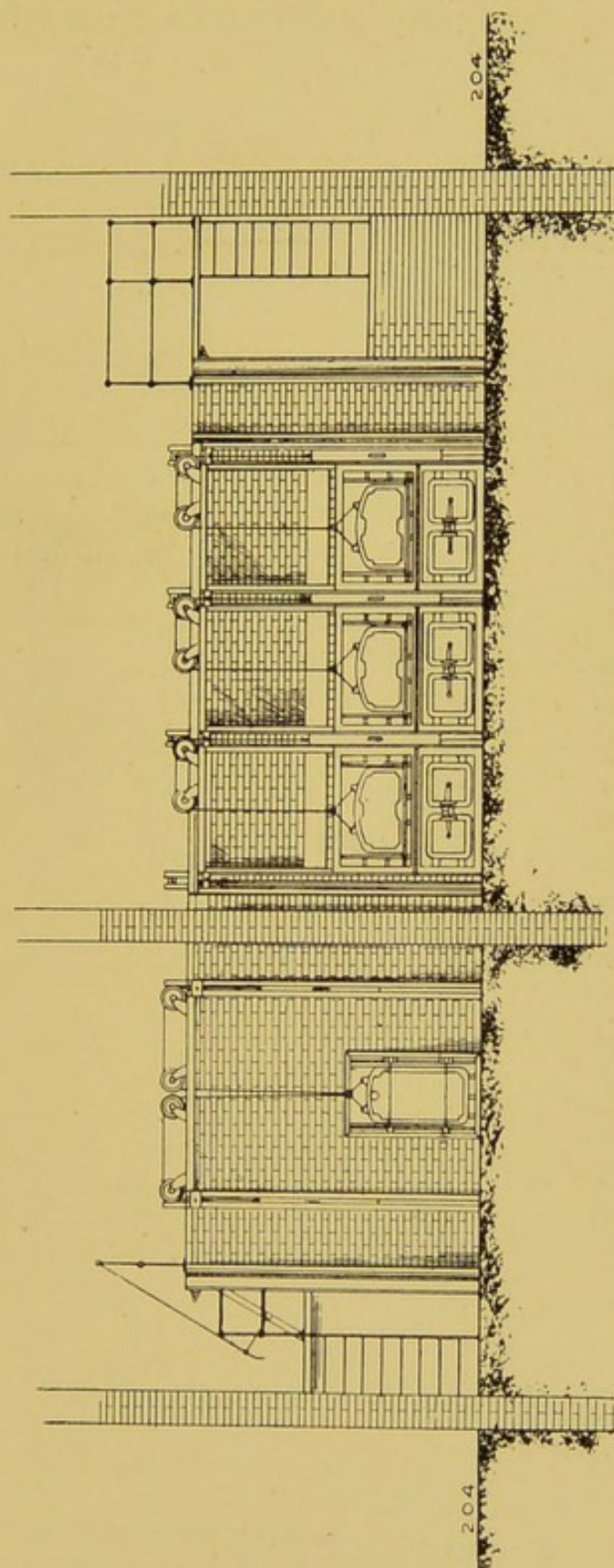
FIG. 10. MELDRUM'S PATENT SIMPLEX REGENERATIVE REFUSE DESTRUCTOR FURNACE, BACK FEED TYPE. Front Elevation.
