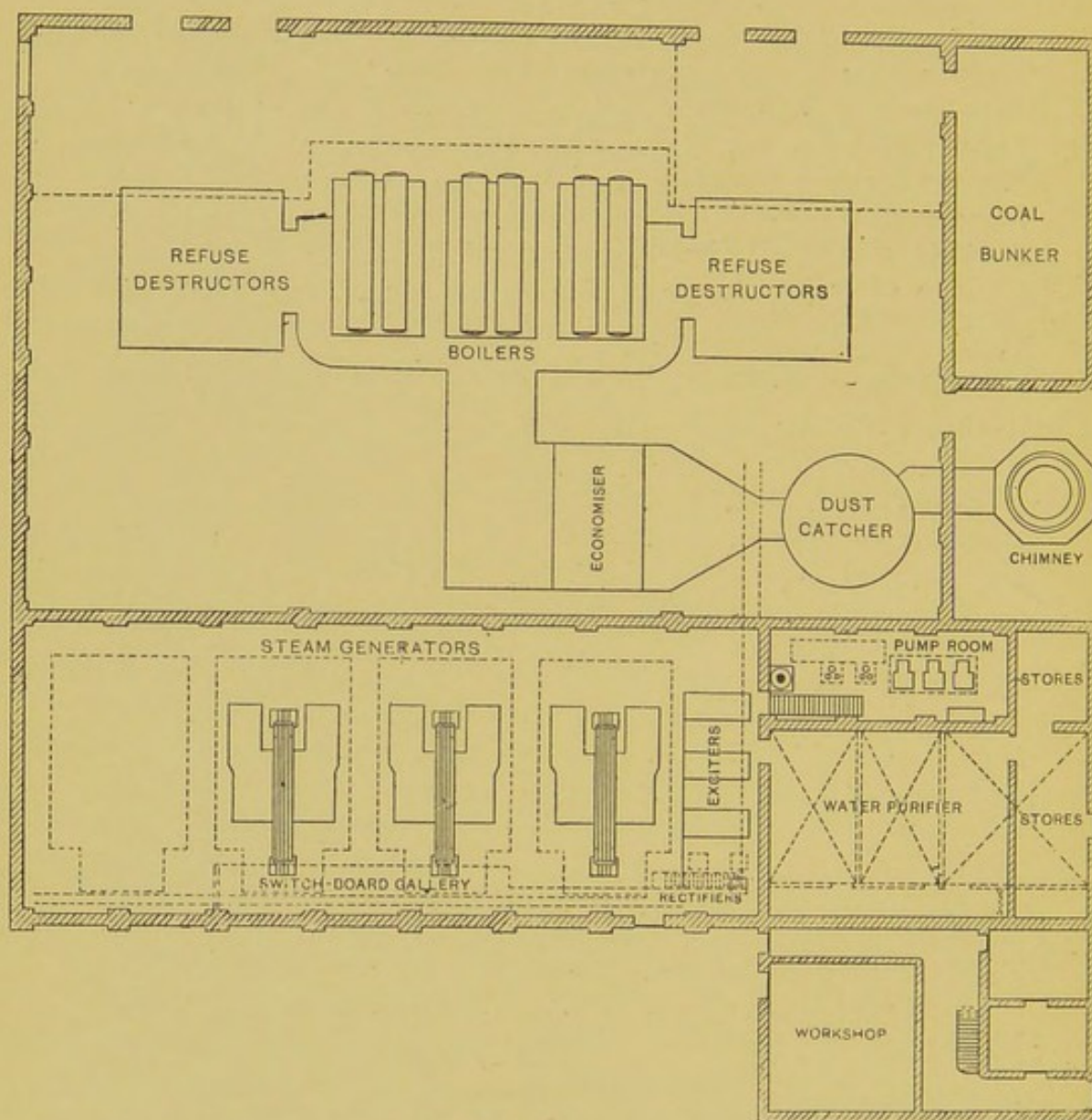
FIG. 47. FULHAM COMBINED DESTRUCTOR AND ELECTRICITY WORKS. Plan.
