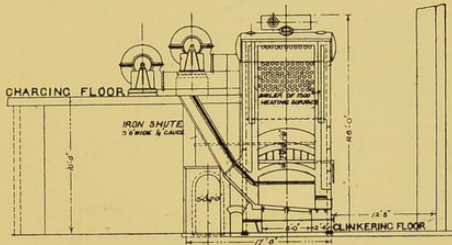
FIG. 12. HEENAN'S DESTRUCTOR, BACK HOPPER FED TYPE. Section.
