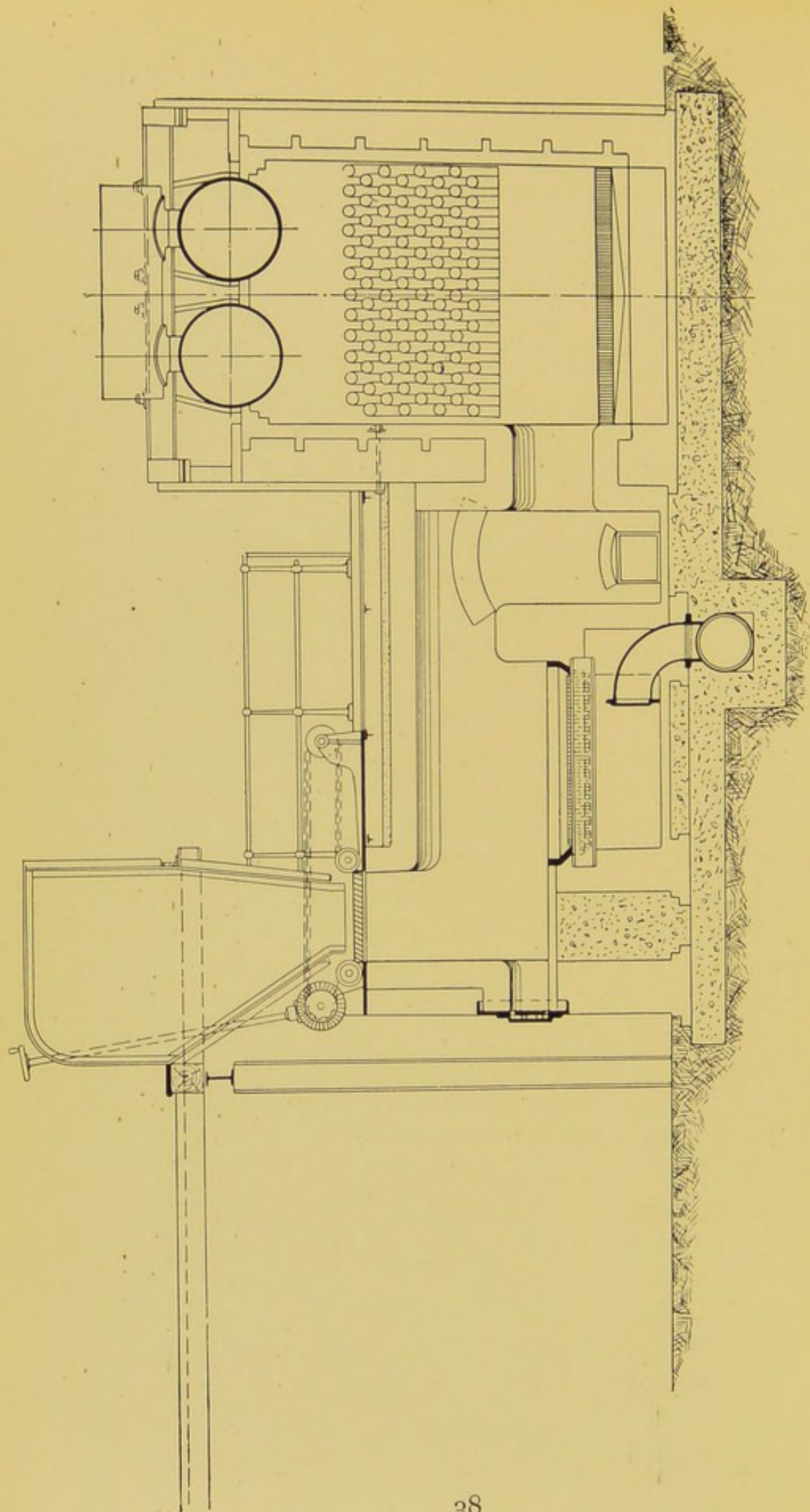
8. MELDRUM'S, BEAMAN & DEAS' TYPE OF DESTROYER WITH MARTEN'S PATENT DIRECT CHARGING APPARATUS. Section through Cell and Boiler.
