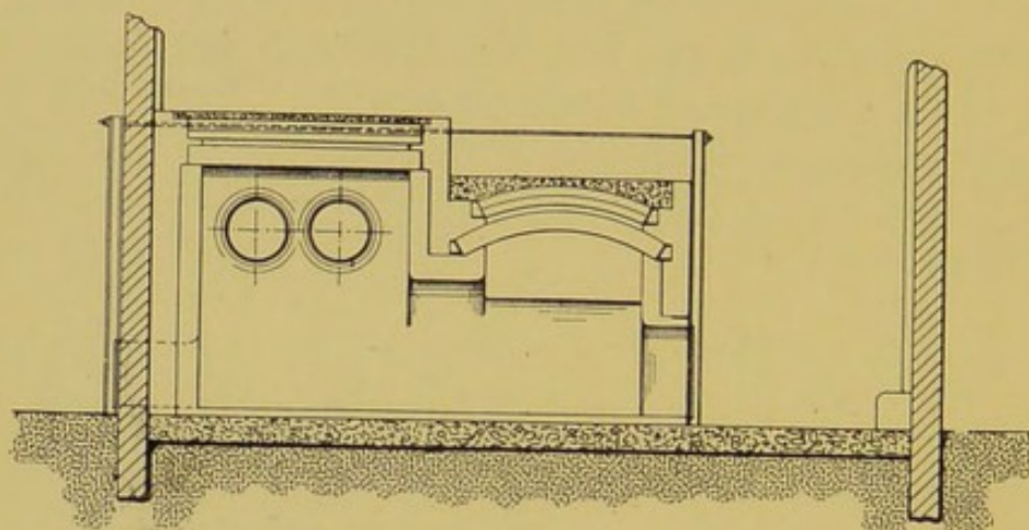
FIG. 64. GRAYS COMBINED DESTRUCTOR AND ELECTRICITY WORKS Sectional Elevation.
