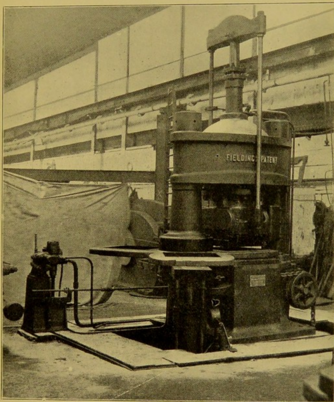
FIG. 31. FIELDING & PLATT'S THREE MOULD HYDRAULIC FLAG PRESS.
