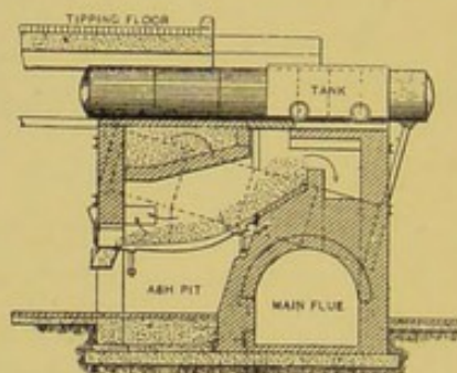
FIG. 19. FRYER'S IMPROVED TOP FED DESTRUCTOR, EMBODYING BOULNOIS, WOOD & BRODIE'S PATENTS.
