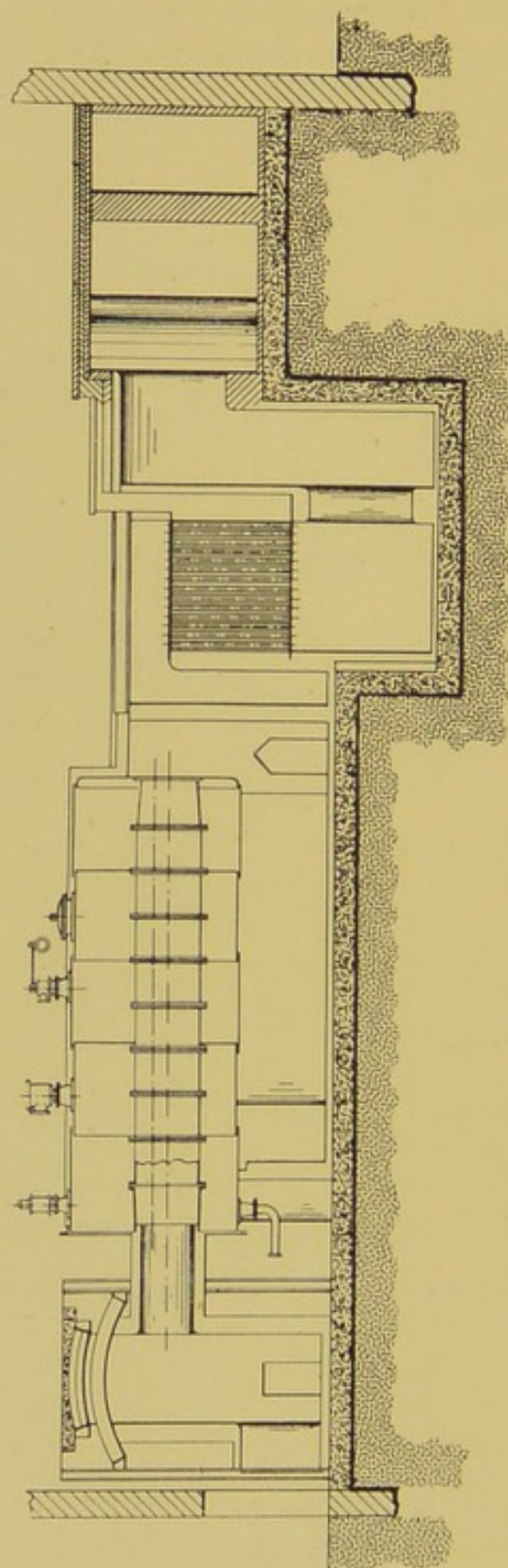
FIG. 67. GRAYS COMBINED DESTROYER AND ELECTRICITY WORKS. Longitudinal Elevation.
