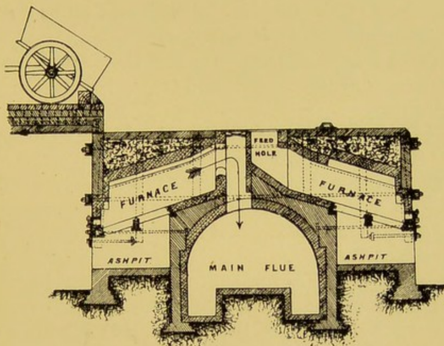
FIG. 14. FRYER'S ORIGINAL TOP FED DESTRUCTOR.
