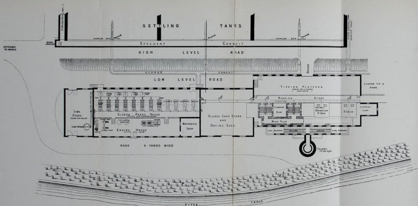
FIG. 57. HACKEN COMBINED DESTROYER AND SEWAGE WORKS, BOLTON. General Plan.
