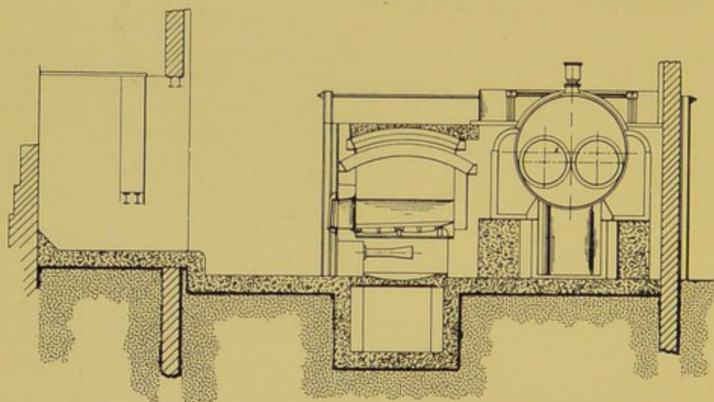
FIG. 65. GRAYS COMBINED DESTRUCTOR AND ELECTRICITY WORKS. Sectional Elevation.
