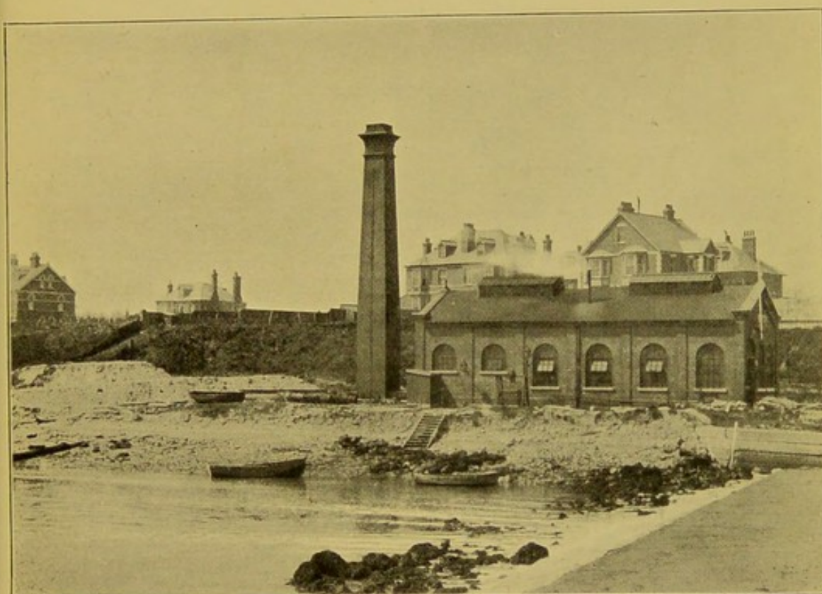
FIG. 89. WEYMOUTH COMBINED DESTRUCTOR AND SEWAGE WORKS. External View.
