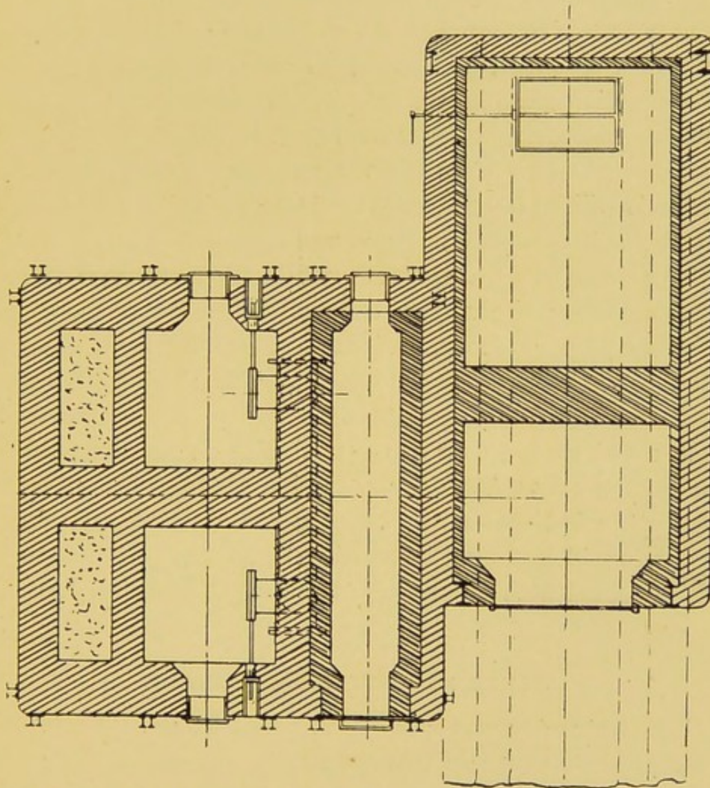
FIG. 28. MELDRUM'S "BEAMAN & DEAS" TYPE DESTRUCTOR. Plan.
