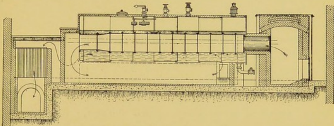
FIG. 25. MELDRUM'S SIMPLEX REGENERATIVE DESTRUCTOR, FRONT HAND OR SHOVEL FED TYPE. Elevation of Boiler and Regenerator.
