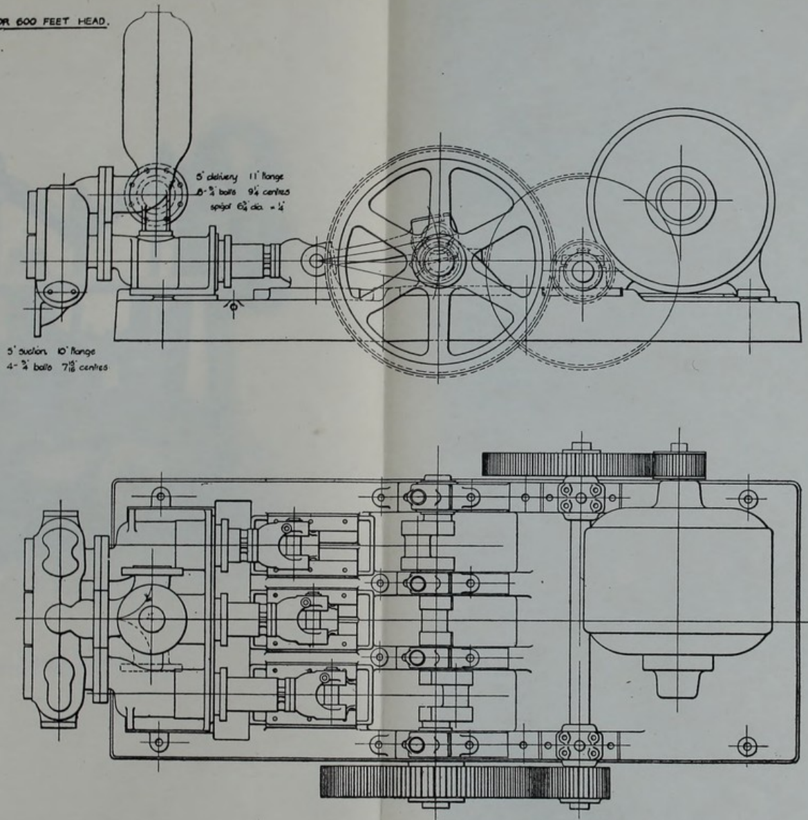
FIGS. 65, 66.—HORIZONTAL TRIPLE RAM PUMP. ARRANGED FOR ELECTRIC DRIVE.
