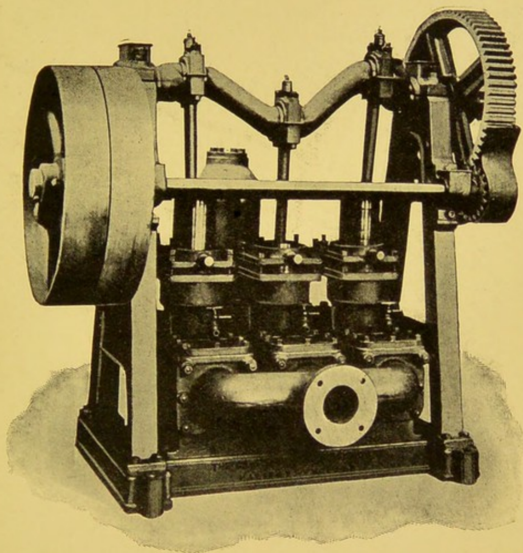
FIG. 67.—THREE-THROW PUMP.
