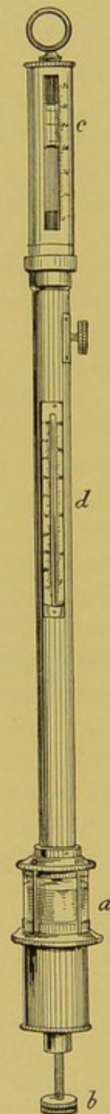
FIG. 1.—Mercurial barometer: a , cistern containing the mercury; b , screw in movable bottom of cistern, to raise or lower the mercury to the "fiducial" point; c , the vernier; d , the thermometer.
