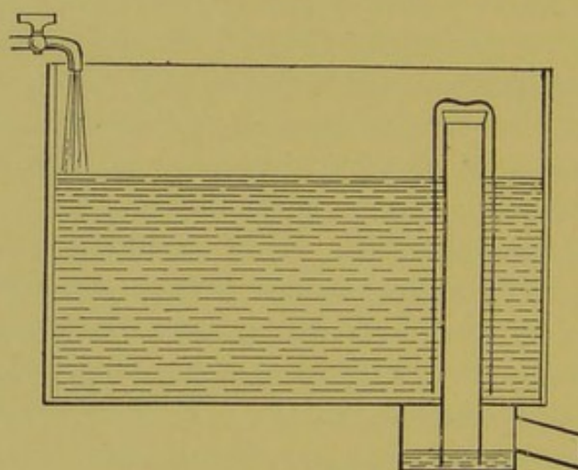
FIG. 43.—Field's flushing tank.
