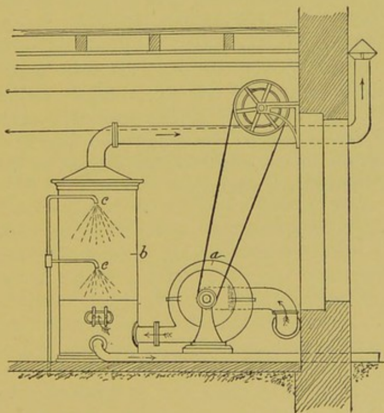
FIG. 21.—Apparatus for removing dust in manufacturing establishments: a , blower; b , dust-collecting chamber; c , water-sprays.
