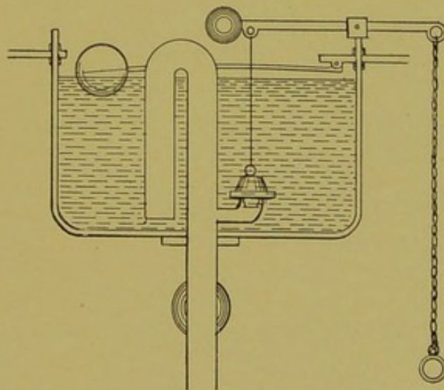
FIG. 34.—Water-waste preventer.
