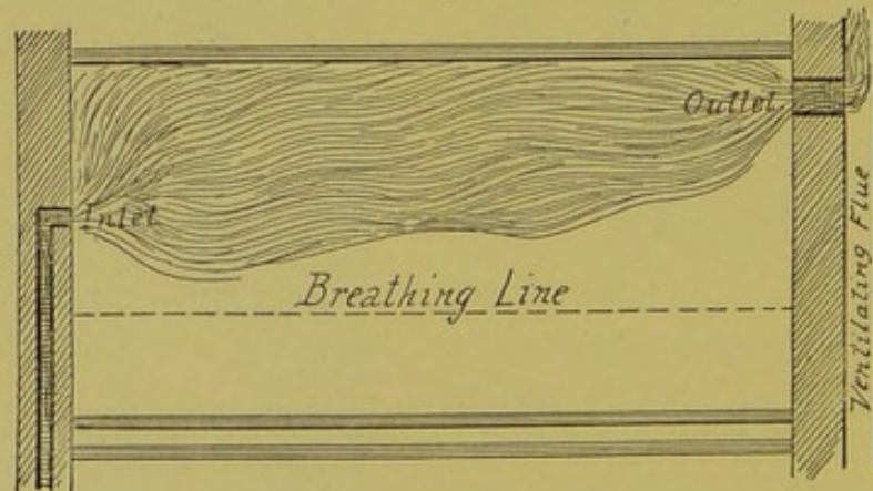
FIG. 12.—Air introduced on side, discharged at top.
