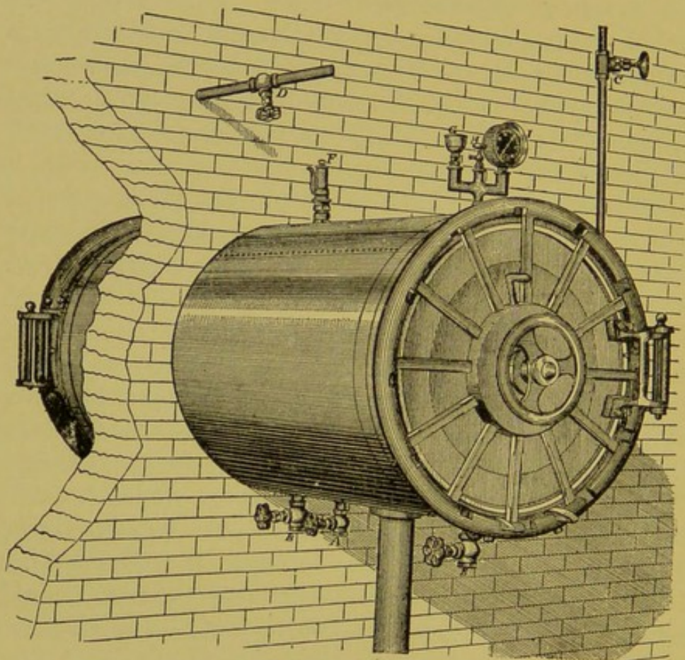
FIG. 60.—Steam disinfecting plant.
