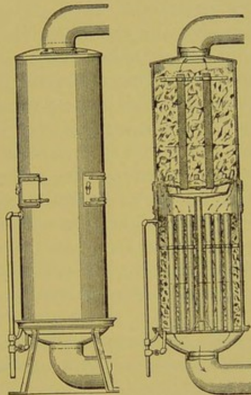
FIG. 58.—The Nevo. Front and sectional views.
