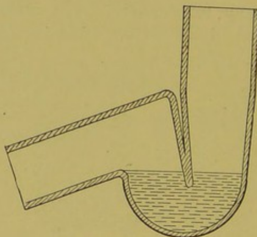
FIG. 38.—Anti-D trap.
