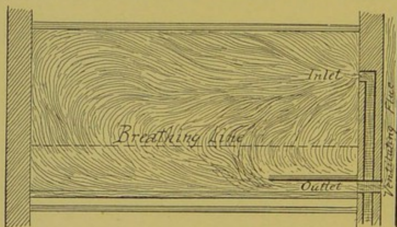
FIG. 16.—Inlet near top, discharge near bottom.
