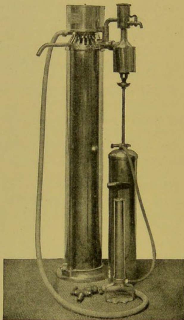
FIG. 55.—Forbes' portable water sterilizer, army type.
