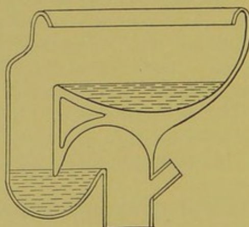
FIG. 32.—Wash-out closet.
