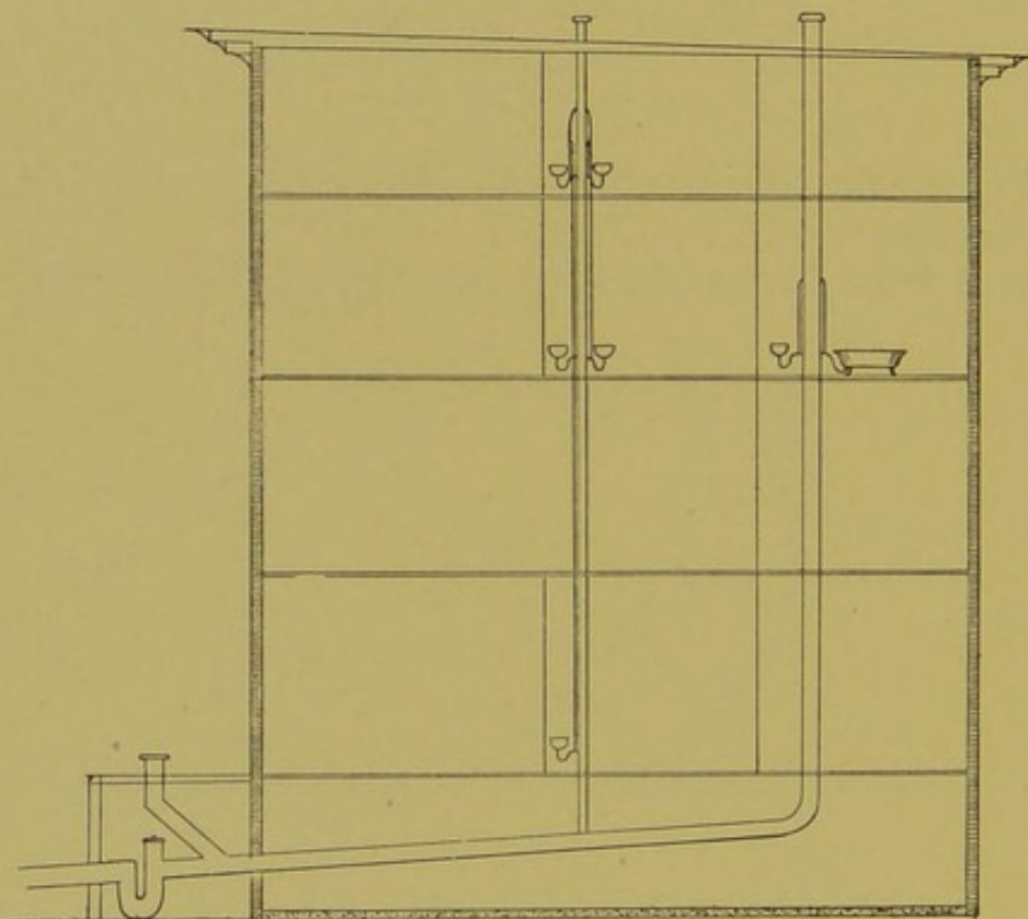
FIG. 41.—Arrangement of soil pipe.
