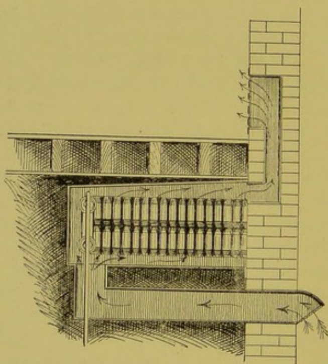
FIG. 22.—Arrangement of indirect heating surface.
