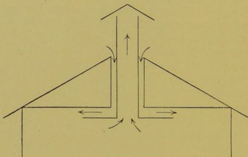
FIG. 56.—Diagram illustrating ridge ventilation.
