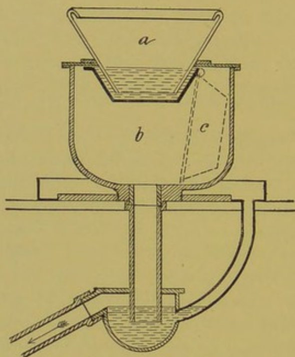
FIG. 30.—Pan closet.
