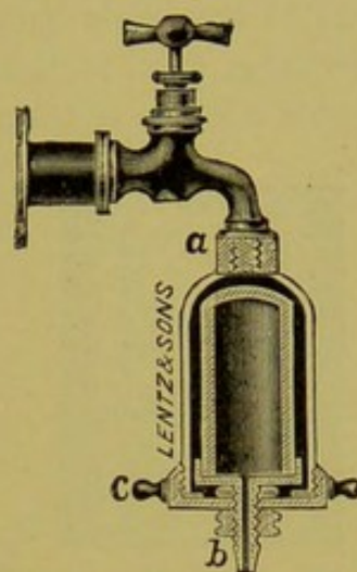
FIG. 26.—Domestic filter—Berkefeld: a , point of attachment to faucet; b , outlet.
