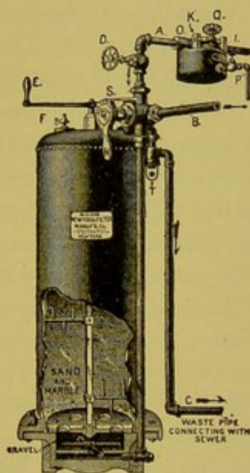
FIG. 25.—Mechanical filter: A, inlet pipe; B, outlet pipe; C, waste pipe; D, valve to cut off water from filter; E, lever to operate the agitator; F, air valve; H, handle of valve used to change the course of the water through the filter; I, distal attachment of coagulating tank to inlet pipe; K, lever valve regulating the quantity of alum supplied; O, proximal attachment of coagulating tank to inlet pipe; P, waste pipe leading from the coagulating tank to the sewer; Q, valve which fastens on the cover of the coagulating tank; S, pointer which indicates the course of the water through the filter; T, sight glass.
