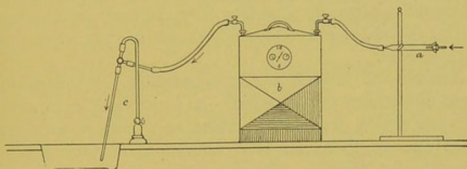
FIG. 5.—Apparatus required with this method. It consists of: a , a small glass tube, twenty centimeters in length, consisting of a narrow portion four centimeters long and three millimeters in its internal diameter, and a dilated portion sixteen centimeters long and twelve millimeters in its internal diameter. This tube contains the granular pumice-stone which serves as the absorbent material in this method; b , is the gas-meter; and c , a Chapman water pump.
