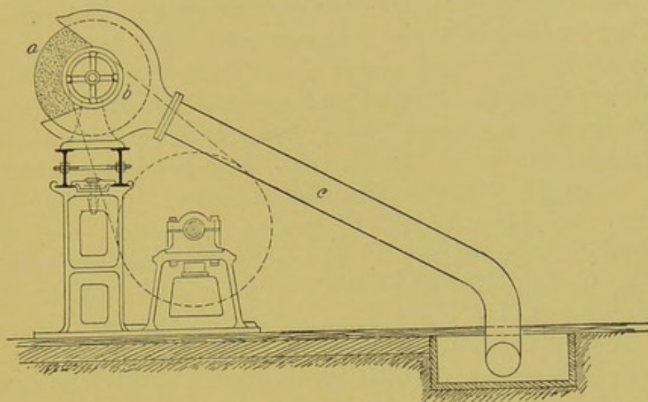
FIG. 20.—Apparatus for removing dust in manufacturing establishments: a , emery wheel; b , hood over emery wheel; c , exhaust shaft.
