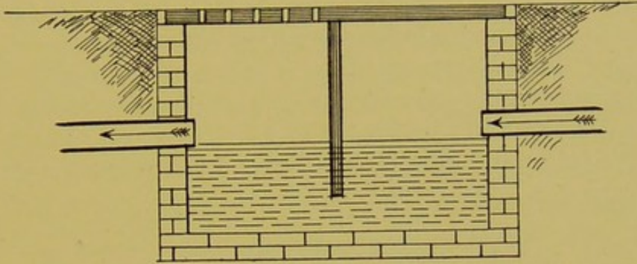
FIG. 39.—Mason's trap.
