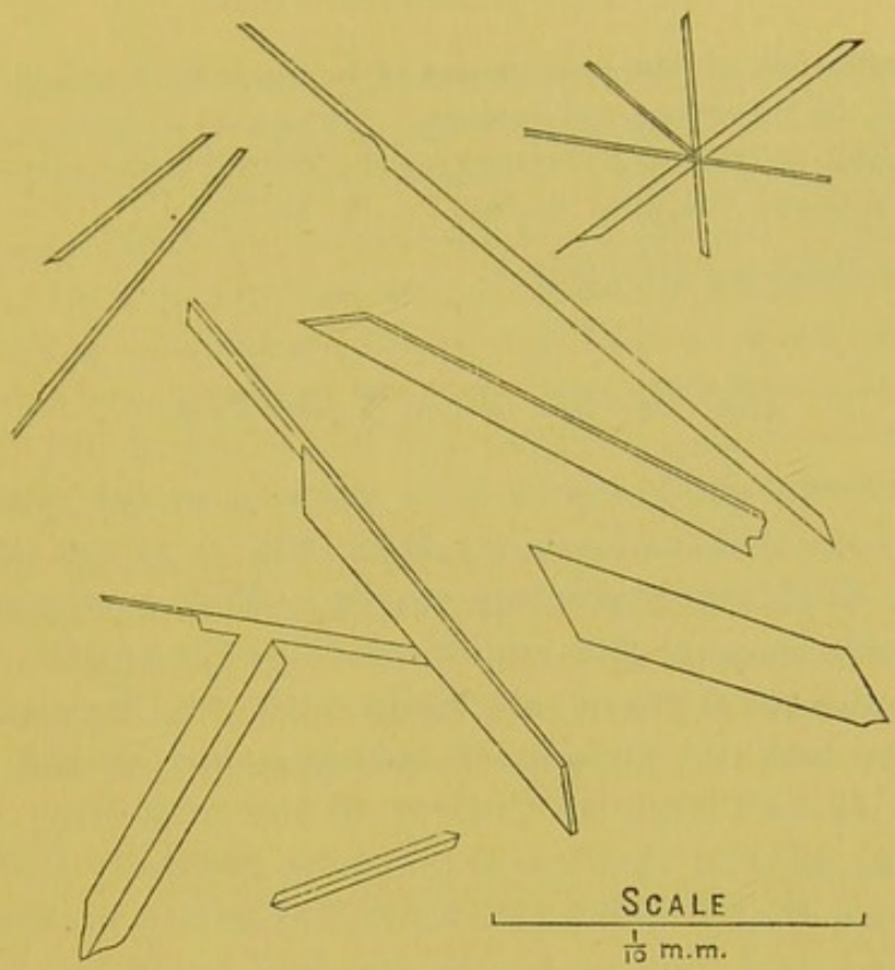
Crystals of Pyrocatechin.
