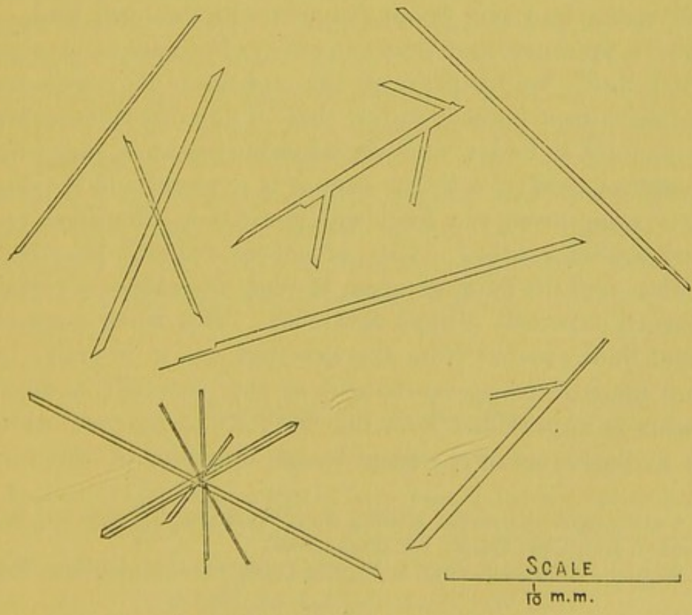
Crystals from Cerebro-spinal Fluid.
