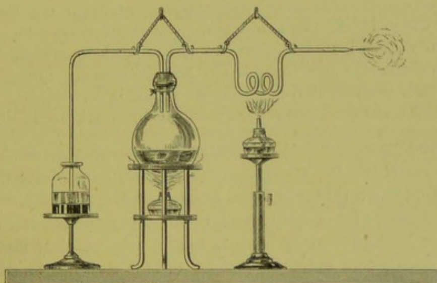
FIG. 1.—SCHWANN'S METHOD.
