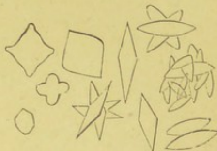
Uric acid, deposited from alkaline urates by the addition of excess of acid \times 216 p. 181.
