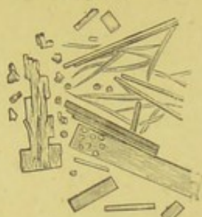
Human blood crystals. x 215. p. 192.
