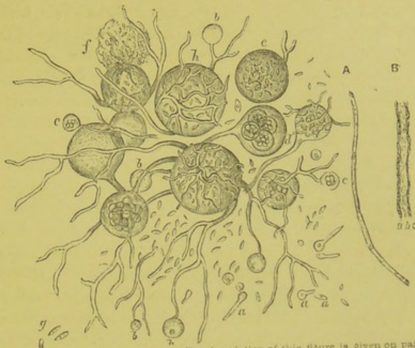
Chionophye Carteri . After Dr. CARTER. The description of this figure is given on page 497. x about 250 (reduced from large drawing) p. 496
