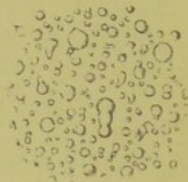
Oil globules from Milk \times 215
