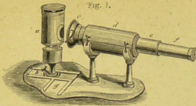
Clinical microscope with stand, arranged for class purposes, with lamp. † 2. p. 23.
