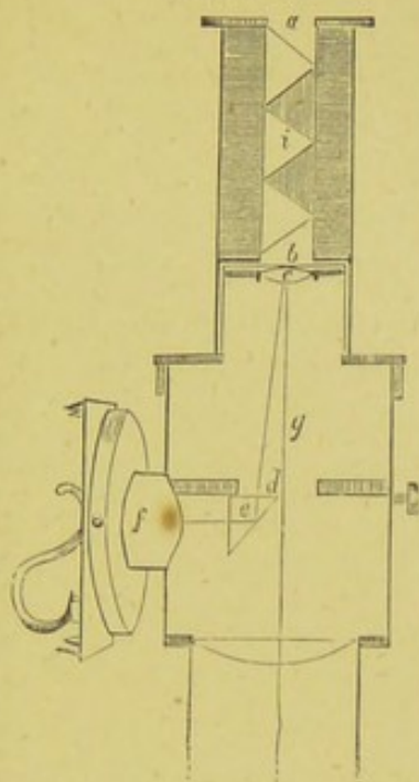
Mr. Sorby's spectrum eye-piece for the microscope, with arrangement for producing two spectra for comparison, p. 195.
