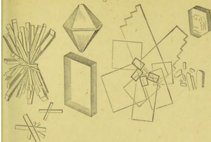
Crystals of Creatine p. 180.
