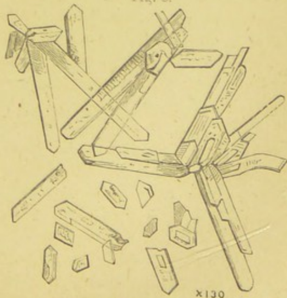
Crystals of diabetic sugar from urine. p. 196.
