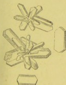
Lactate of copper. p. 181.
