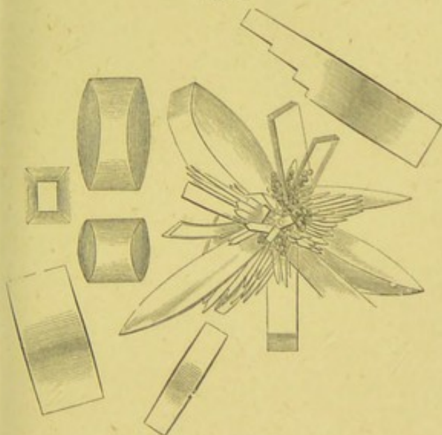
Crystals of Creatinine. p. 181.
