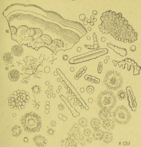
Crystals of Leucine. a crystals d from water, the remainder from an alcoholic solution. p. 189.
