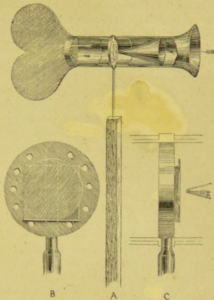
Apparatus employed by Dr. Cunningham, in India, for collecting atmospheric dust for microscopical examination. a , vane; b , diaphragm-plate enlarged; c , sectional view of collecting glass shown on a larger scale.
