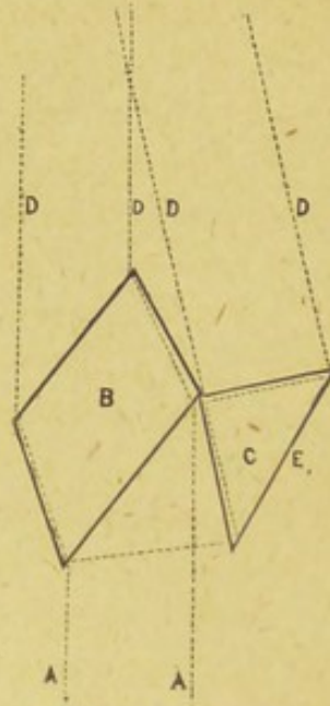
Powell & Lealand's binocular arrangement for high powers. AA, rays of light proceeding from object glass, B, parallel piece of glass, C, triangular prism DDDD, emergent rays. p. 25.
