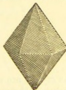
The Triangular Dodecahedron.
