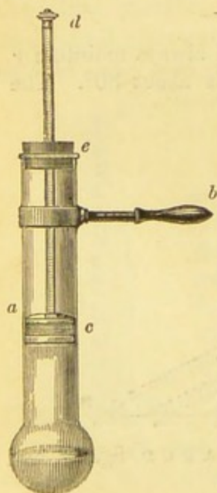
(20) a represents the glass tube, with the bulb at its lower end; b is the handle by which it is held; c is the piston, the rod of which passes through a cork at e .
