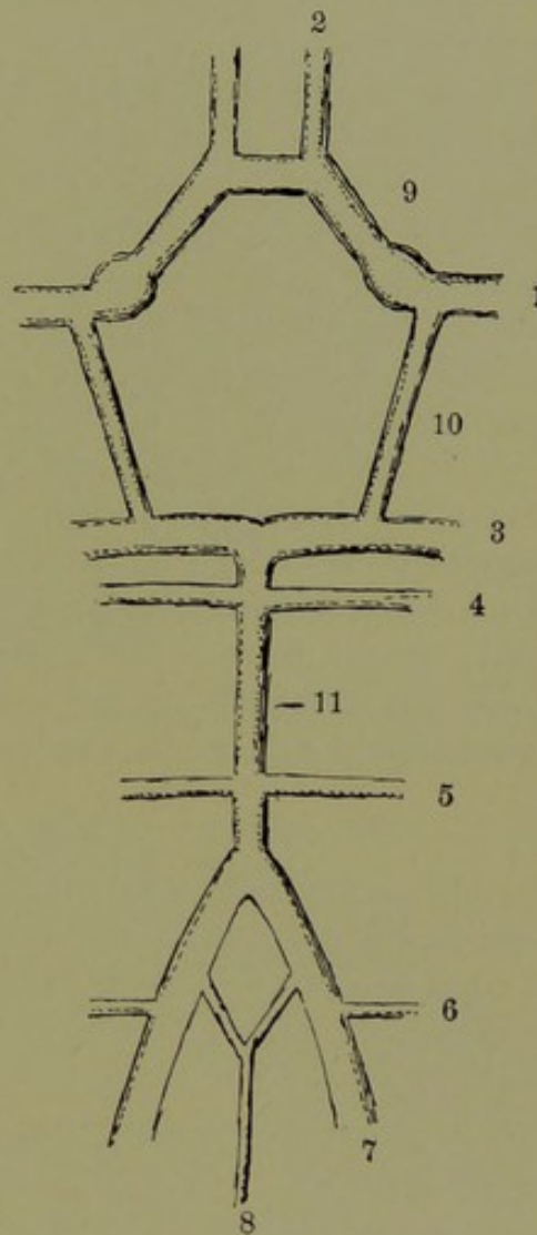
FIG. 1.—DIAGRAM OF THE CIRCLE OF WILLIS. 1, Sylvian artery; the bulbous enlargement represents the confluence of the internal carotid with the Sylvian artery; 2, anterior cerebral artery; 3, posterior cerebral artery; 4, superior cerebellar artery; 5, middle cerebellar artery; 6, inferior cerebellar artery; 7, vertebral artery; 8, anterior spinal artery; 9, anterior communicating artery; 10, posterior communicating artery. After VAN GEHUCHTEN.
