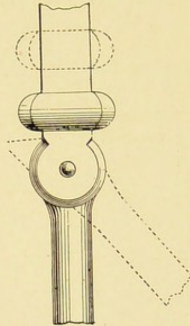
Fig. 38.—Ring-catch Joint.
