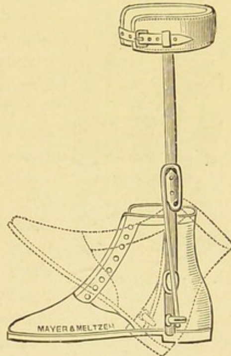
Fig. 54.—Boot and Iron, with Spring for elevating foot in Talipes Equinus.
