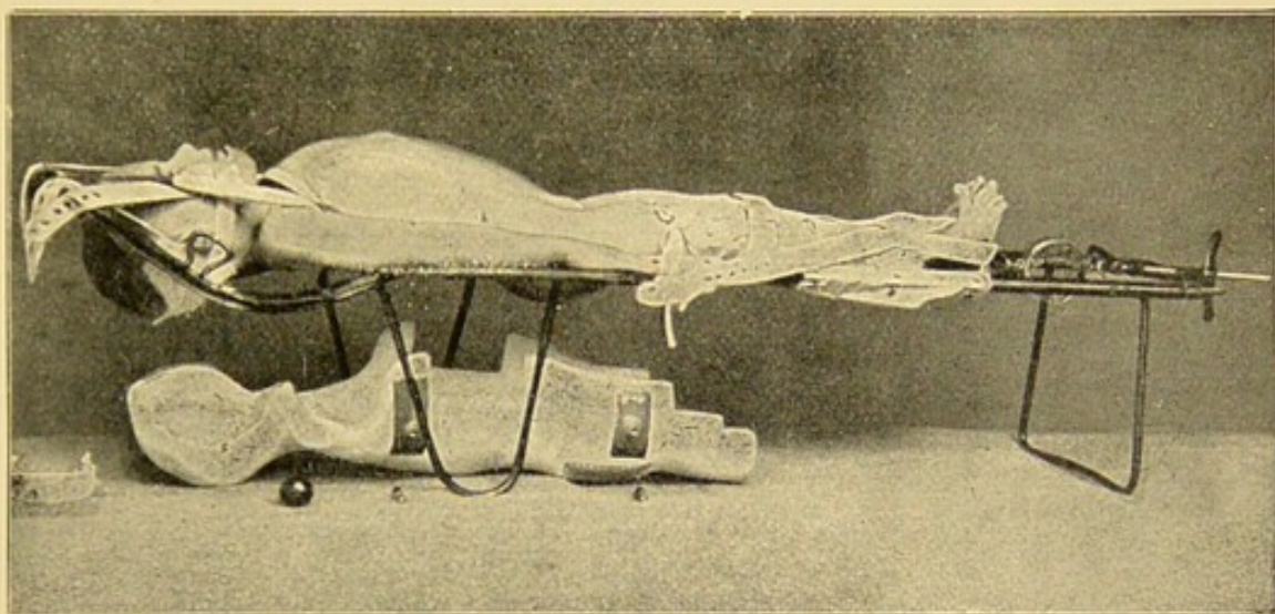
Fig. 288.—Wullstein's Apparatus for the Gradual Correction of Deformity in Spinal Disease. ( Centralblatt für Chirurgie. )
