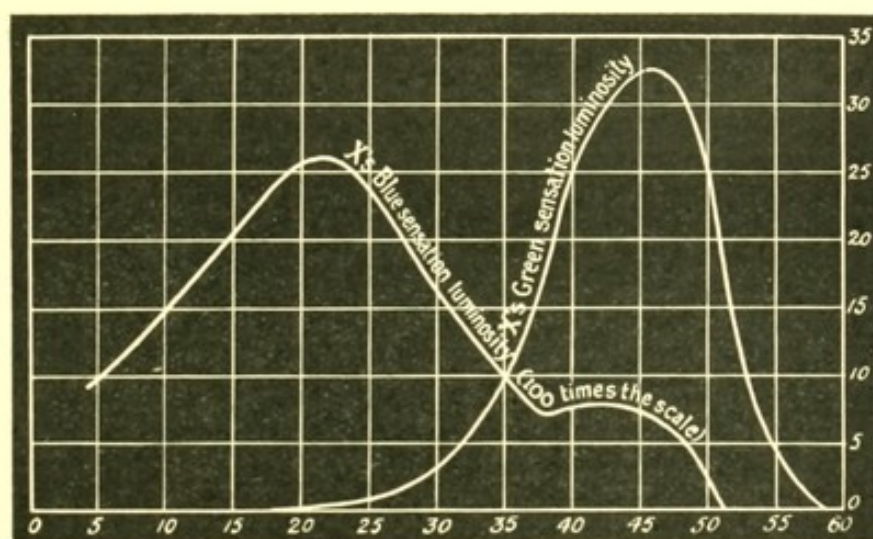
FIG. 88.—X.'s colour curves. (Red blind.)
