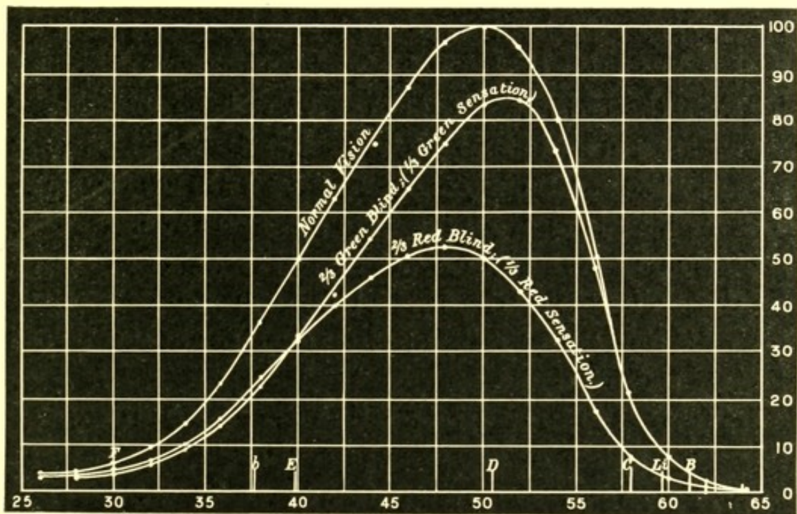
A is 67.2; B, 61.3; Red lithium, 59.8; C, 58.1; D, 50.6; E, 39.8; b , 37.7; F, 30.0; Blue lithium, 22.8; G, 11.2; H, -7.1.
