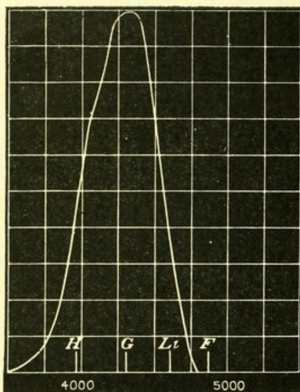
FIG. 76.—Effect of Spectrum on Silver Chloride.
