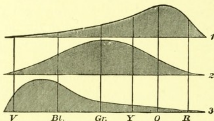
FIG. 75.—Helmholtz's Colour Sensation.
