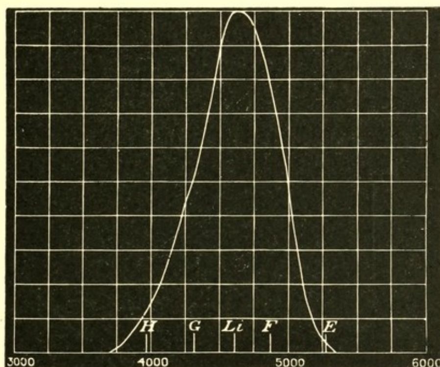
FIG. 77.—Effect of Spectrum on Silver Bromide.
