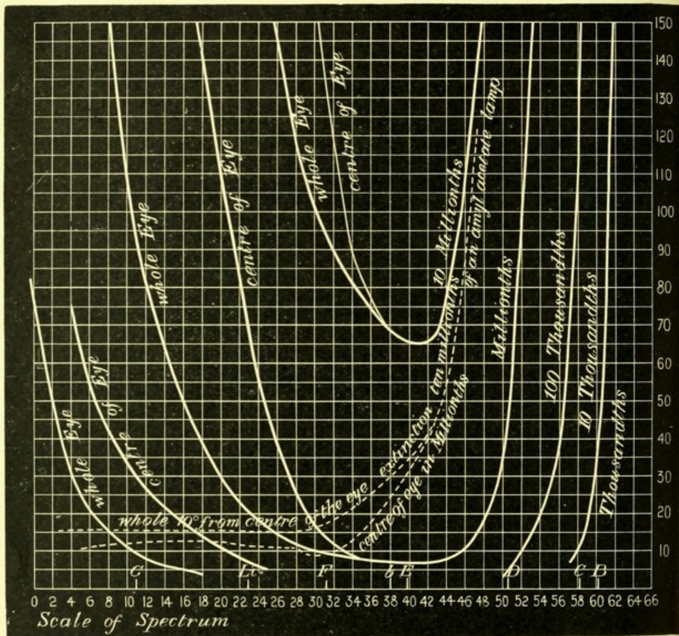
FIG. 56.—Extinction Curves of Normal Eye.
