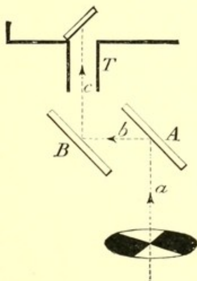
FIG. 55.—Method of Double Reflection into Extinction Box.
