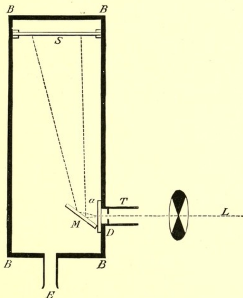
FIG. 54.—Apparatus to Measure Extinction of Light.
