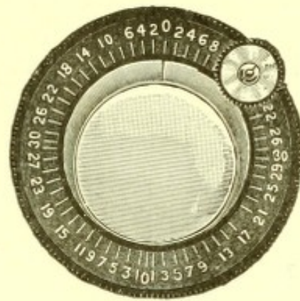
Fig. 54.—Risley rotary prism.
