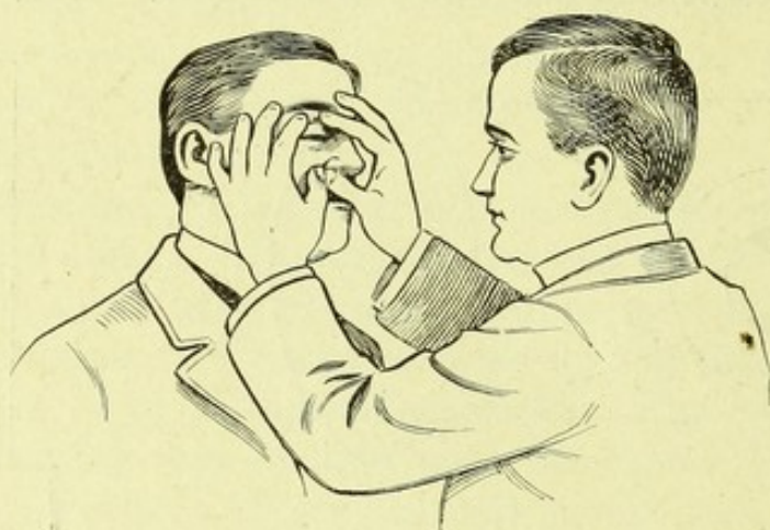
Fig. 20.—Method of testing the tension of the eye. (Ball.)
