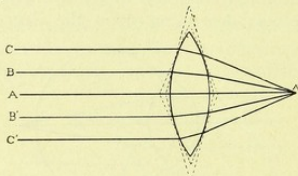
Fig. 28.—Union of parallel rays effected by a convex lens. (Fuchs.)
