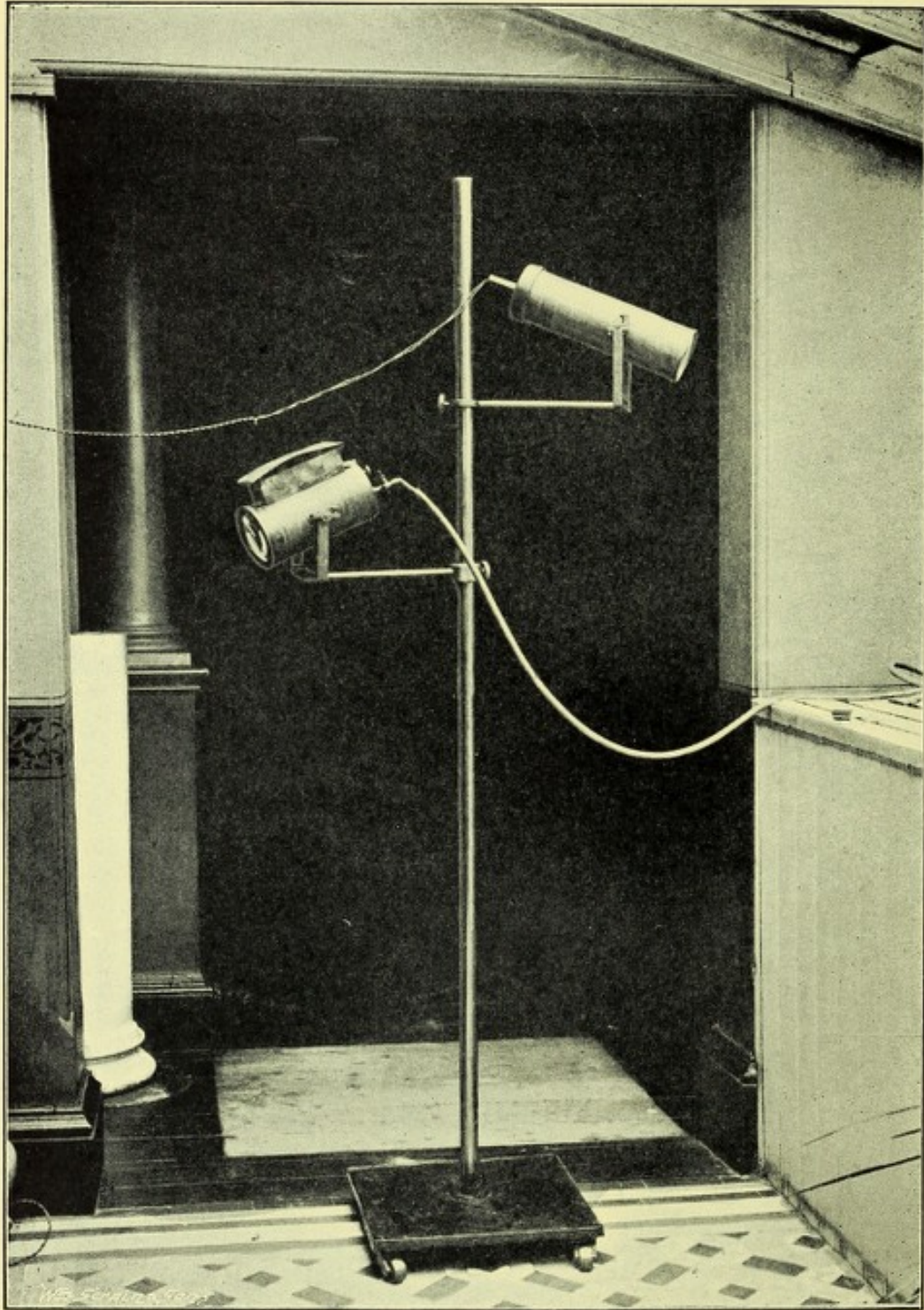
FIGS. 67 AND 68.—The above plate is made from a recent photo, and is meant to be substituted for figs. 22 and 23 on Plate III. It shows the form of the electric lamp I at present use. There is no change in the acetylene lamp.
