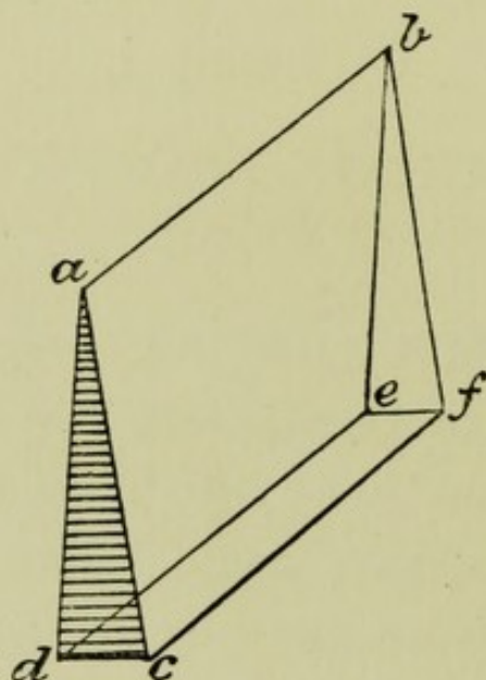
Fig. 1. —A Prism.
