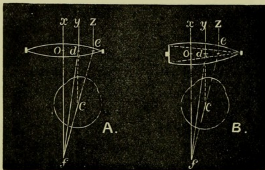
Fig. 53.— A . The right eye is looking at a distant object through a lens displaced inwards, rim and all , by a distance o d ; d c e is the effect on convergence. B is the same eye looking through a lens of the same focal length, but decentred in its rim by the same distance o d . The dotted lines indicate the prism that would be equivalent to the decentering, and the effect on convergence is the same as with A .
