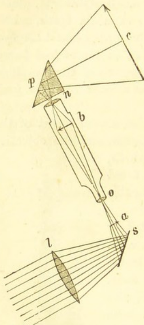
Mode of showing the image of a microscope as an object.
