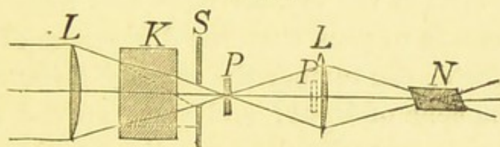
Polarising apparatus of Dubosq.
