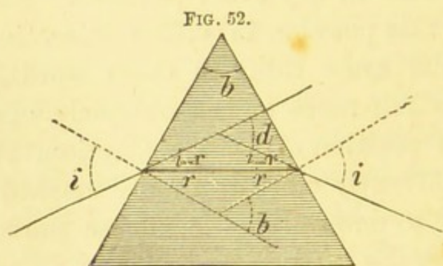
Smallest deflection through a prism.
