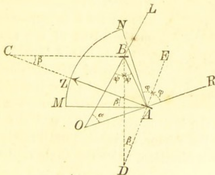
Principle of the mirror sextant.
