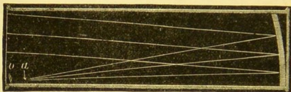
Action of the reflecting telescope with anterior opening.
