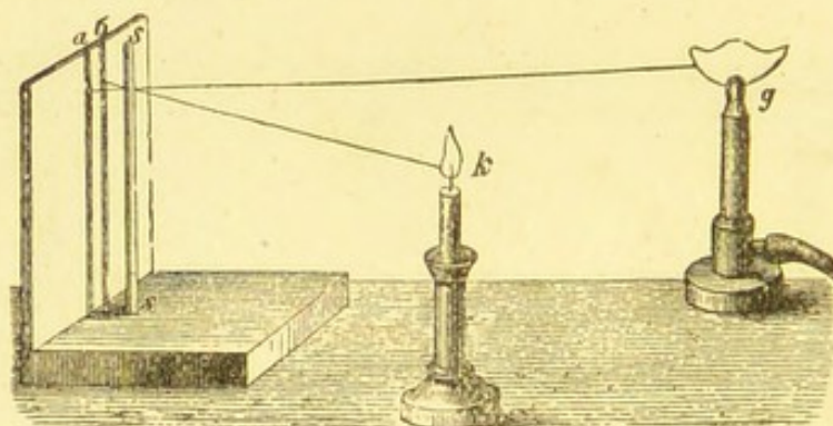
Rumford's Photometer.
