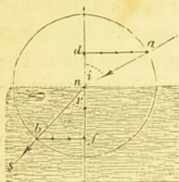
Law of refraction.
