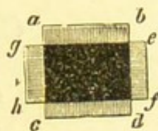
Tourmaline plates placed at right angles.
