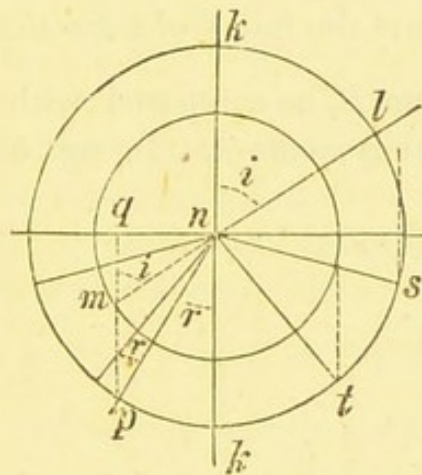
Construction of the refracted ray.
