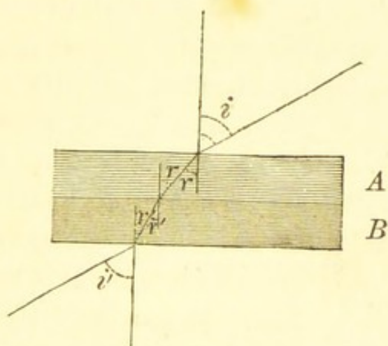
Refraction through two parallel plates.
