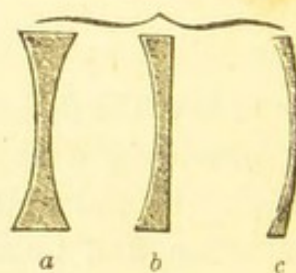
Concave lenses.
