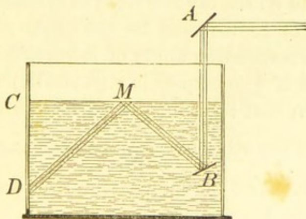
Total reflexion.
