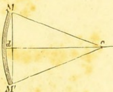
Concave mirror.
