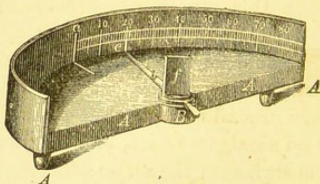
Model for the demonstration of the law of reflexion of light.
