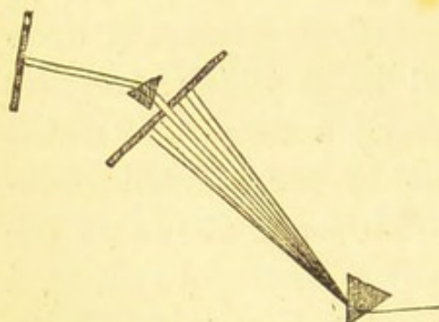
Undecomposability of the colours of the spectrum.
