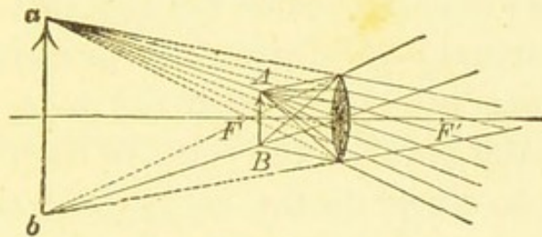
Virtual image with a convex lens.
