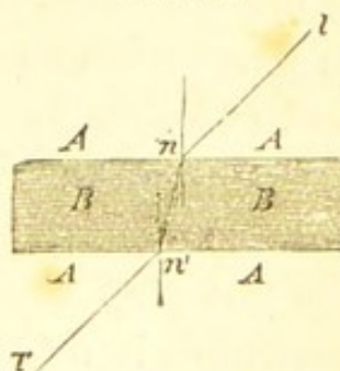
Refraction through a transparent plate with parallel surfaces.
