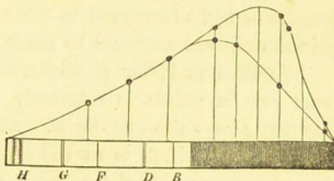
Heat-curves of the spectra thrown by flint glass and rock salt.
