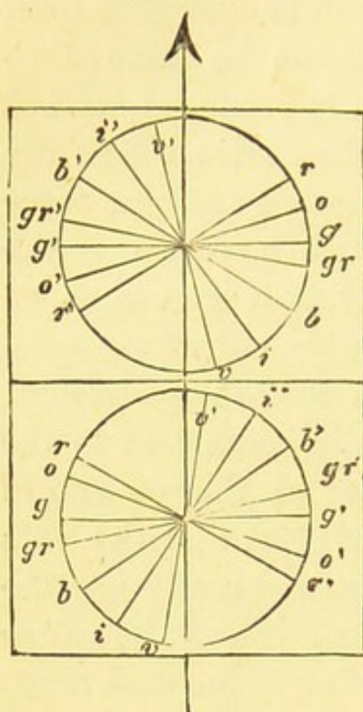
Rotation of the planes of vibration in Quartz.
