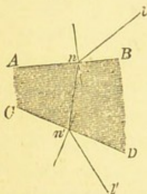
Refraction through a piece of glass, the surfaces of which are not parallel.
