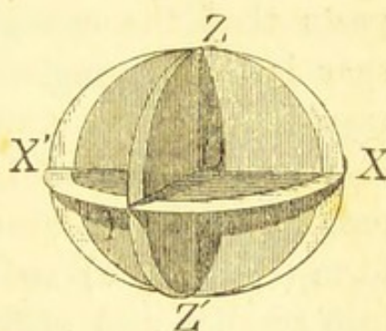
Wave-surface of a negative uniaxial crystal.
