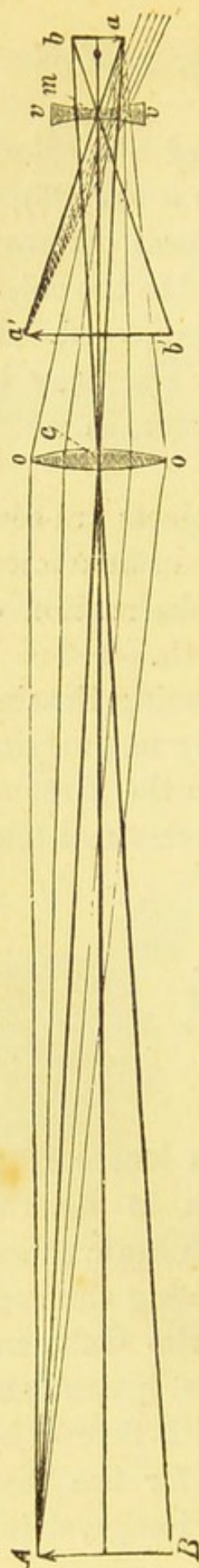
Fig. 83.—Construction of Galileo's telescope.
