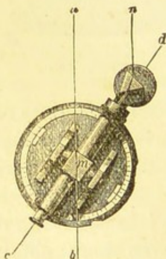
Measurement of refraction as practised by Fraunhofer.
