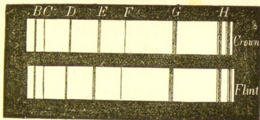
Spectrum thrown by crown glass and by flint glass.
