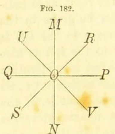
Decomposition of vibrations.
