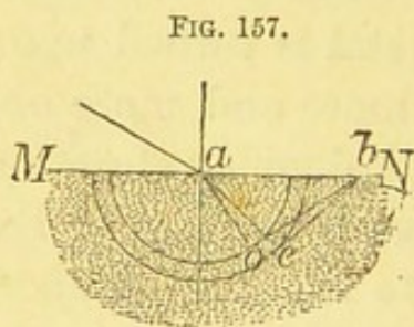
Double refraction. First case.
