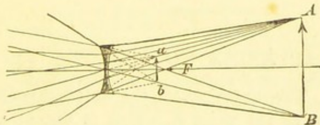
Virtual image formed by a concave lens.
