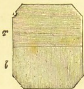
Double plate composed of right and left ro- tating Quartz.
