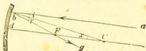
Determination of the position of the principal focal point.
