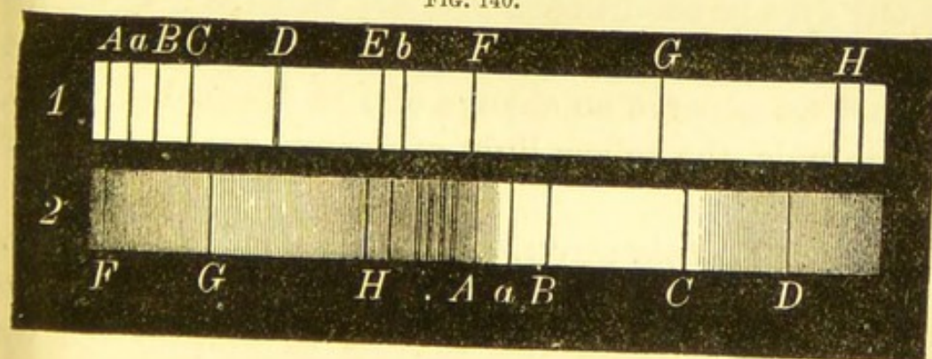
Unusual dispersion power of Fuchsin.
