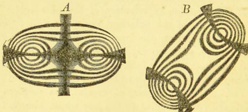
Rings of colour produced by biaxial crystals.
