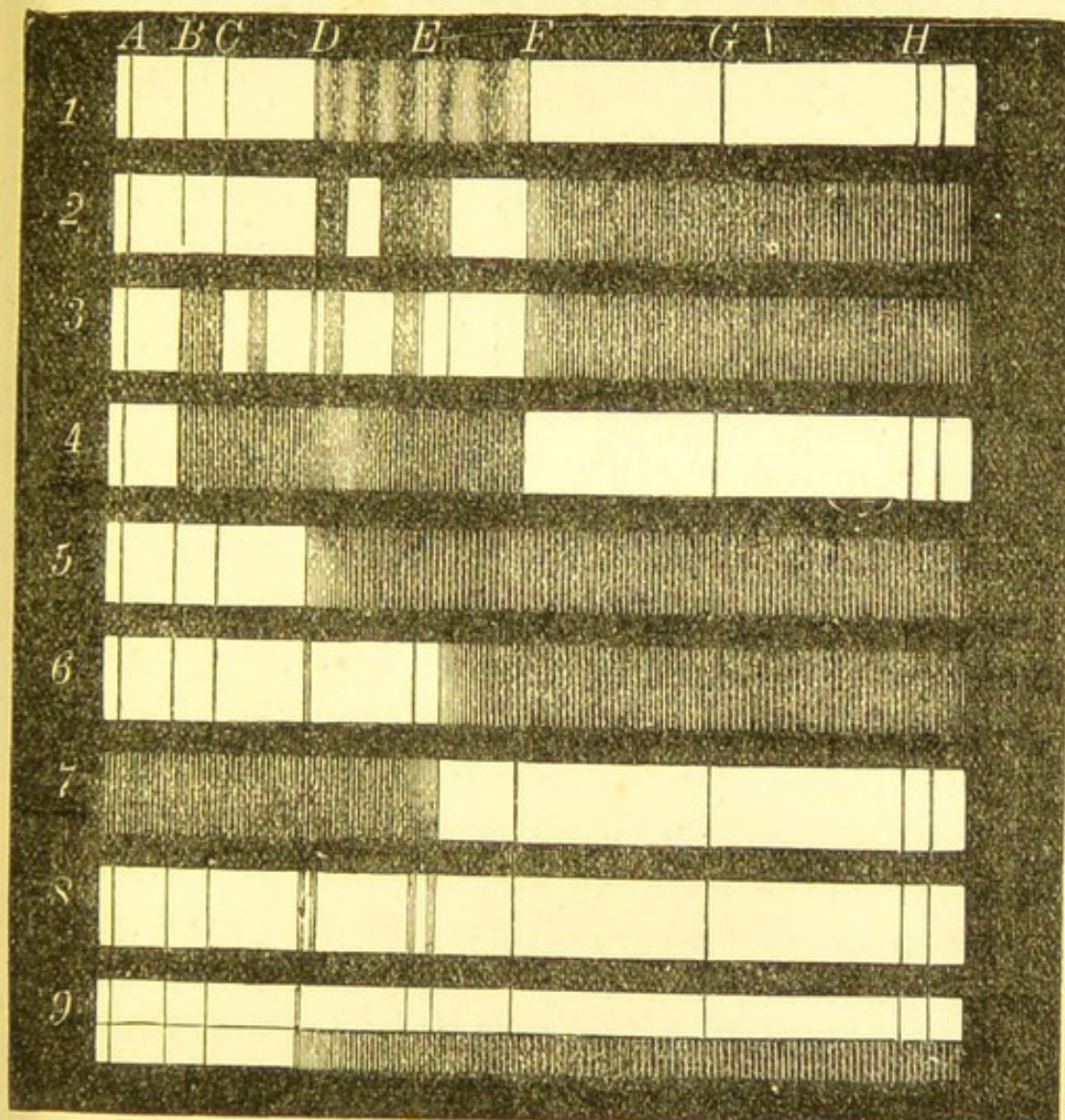
Absorption spectra.
