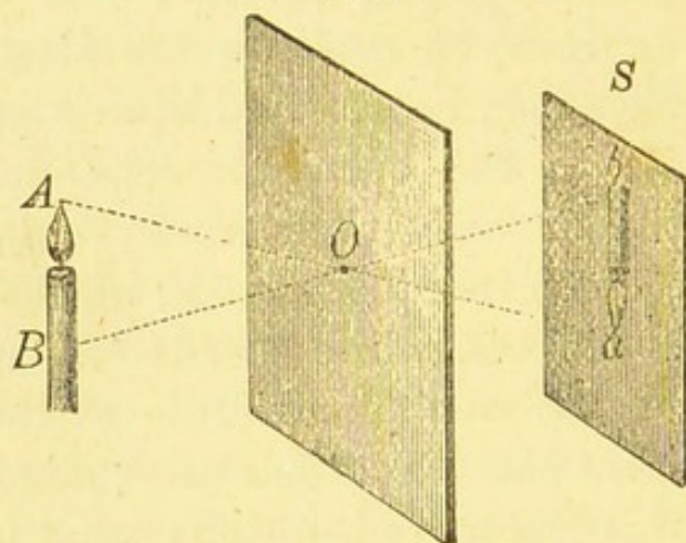
Projection of an image through a small aperture.
