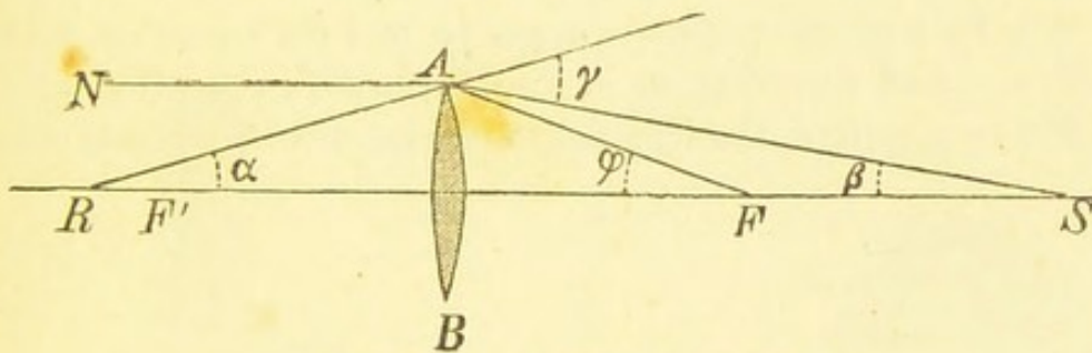
Determination of conjugate points.
