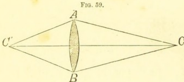
Axis and centres of curvature.
