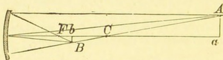
Construction showing the formation of the image.
