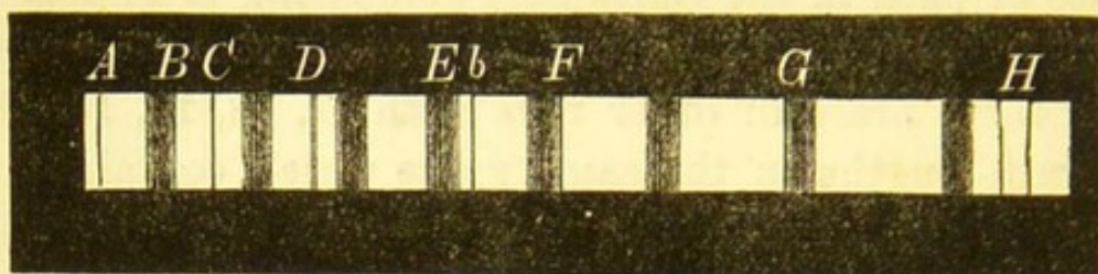
Interference striæ in the spectrum.
