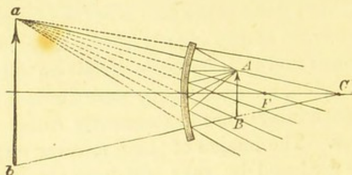
Production of a virtual image.
