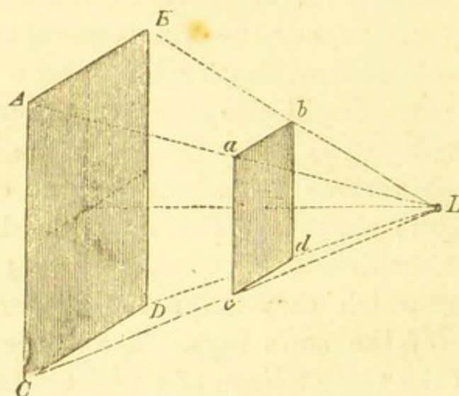
Diminution of the illumination in the ratio of the square of the distance.
