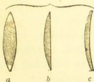
Convex lenses.
