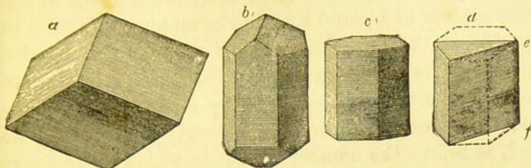
Crystalline forms of Iceland spar.
