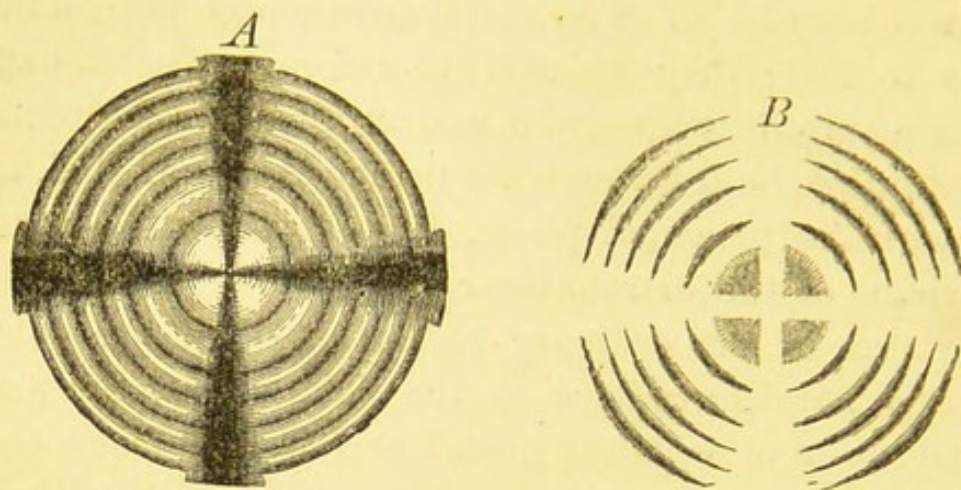
Rings of colour produced by uniaxial crystals.
