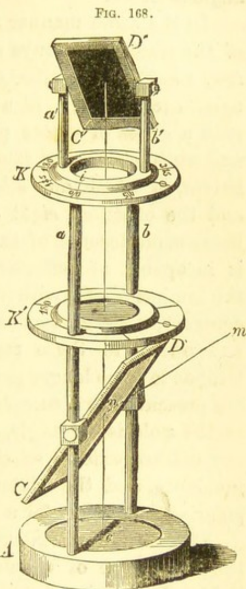
Nörremberg's polarising apparatus.
