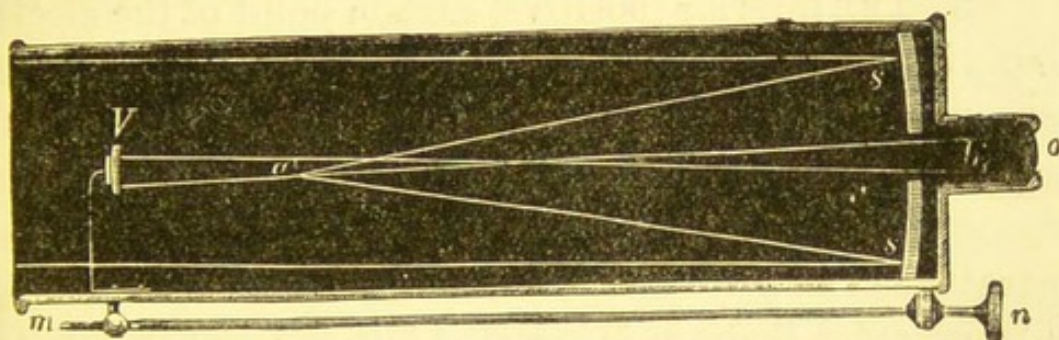
Action of Gregory's reflector.
