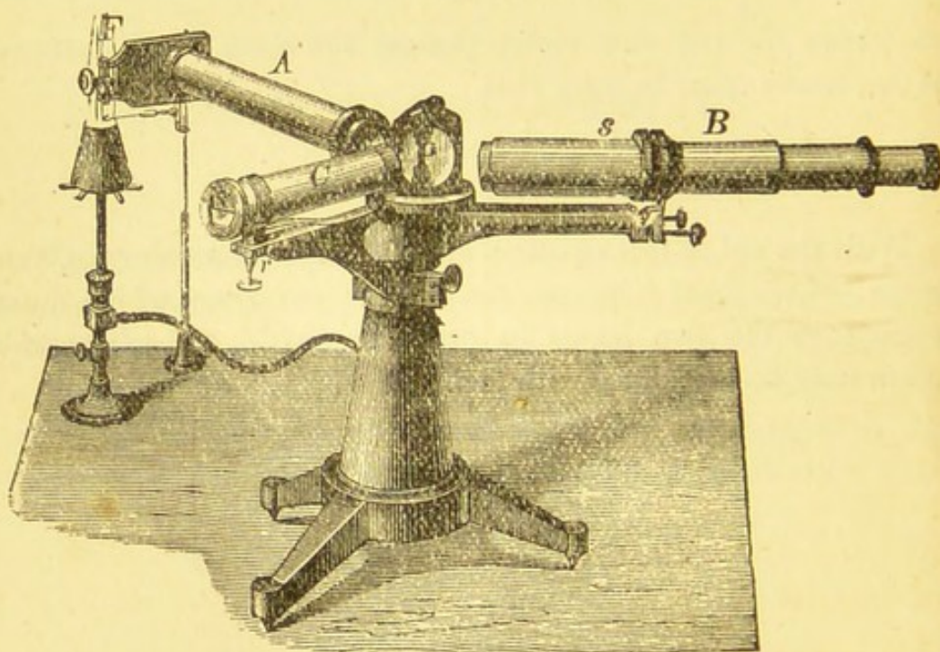
Bunsen's spectroscope.
