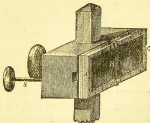
Fresnel's mirror.
