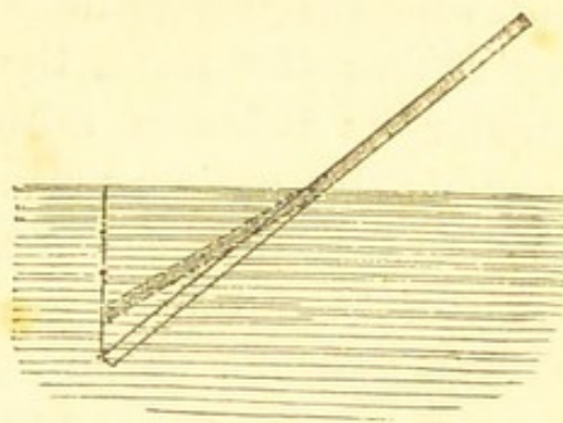
Appearance presented by a rod dipped in water.
