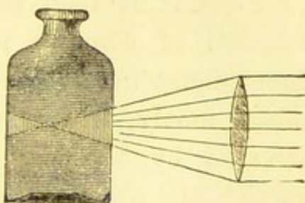
Fluorescence.
