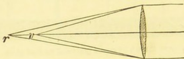
Dispersion of colour of a lens.
