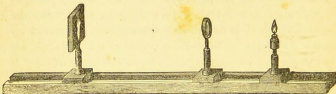
Real image seen through a convex lens.
