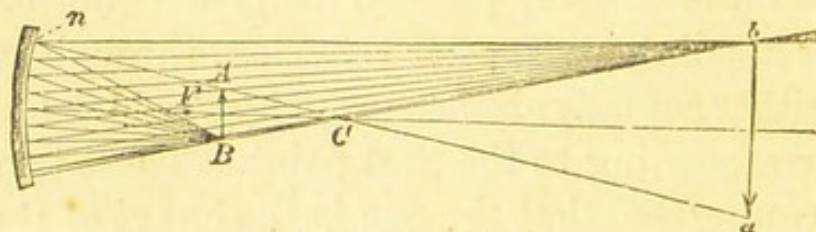
Production of real images.
