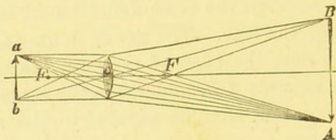
Production of a real image.
