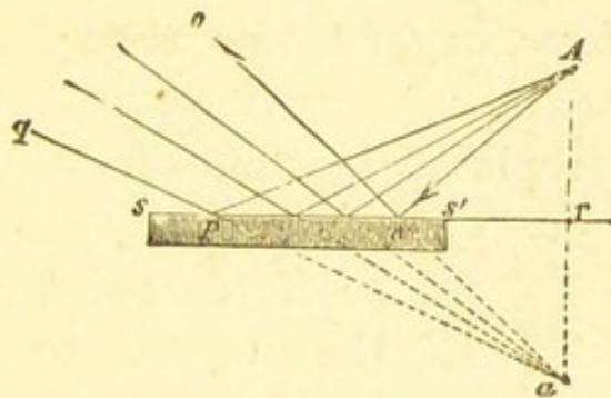
Production of the image point in a plane mirror.
