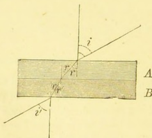
Refraction through two parallel plates.
