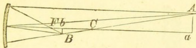
Conjugate foci on a secondary axis.
