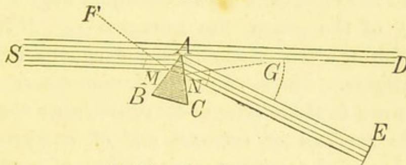
Deflection through a prism.
