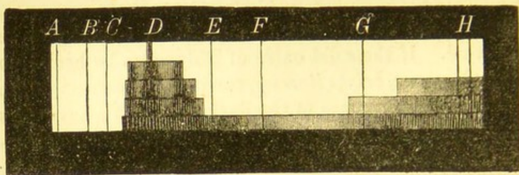
Absorption of the colouring matter of litmus with different thicknesses of the layer.
