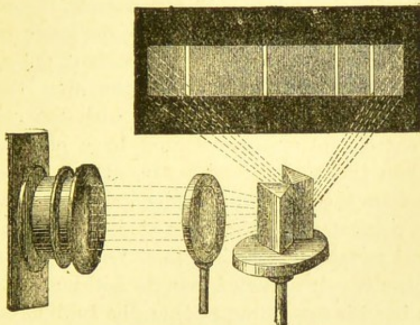
Different deflection of different coloured rays of light.
