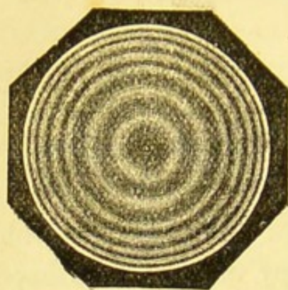
Newton's coloured rings.
