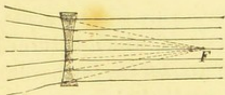
Virtual focus of a concave lens.
