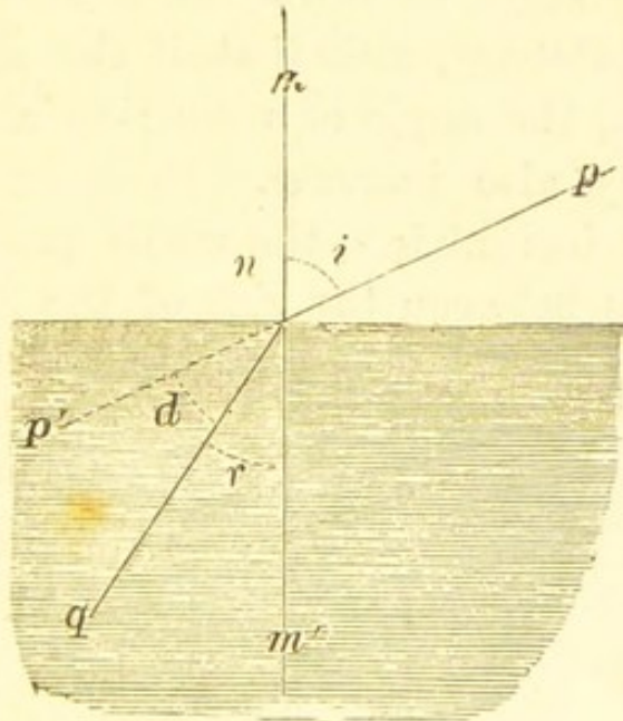
Angles of incidence and of refraction.
