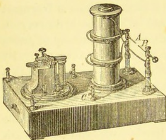
Induction apparatus.
