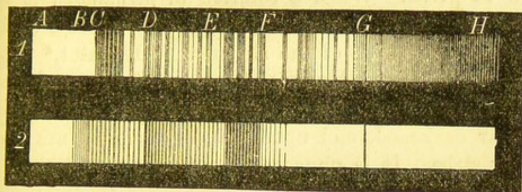
Absorption spectra of nitrogen tetroxide and of the vapour of iodine.
