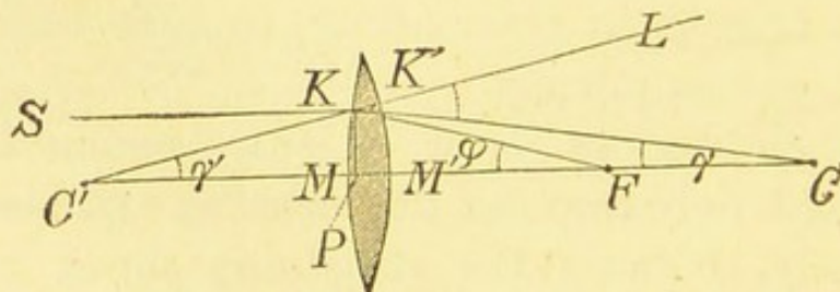
Determination of the focal distance.
