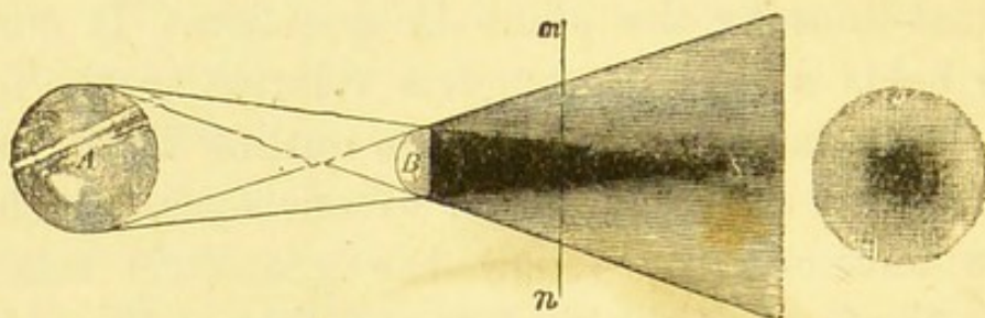
Shadow nucleus, and penumbra.
