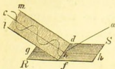
Polarisation by reflexion.
