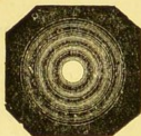
Phenomena of diffraction with a circular aperture.
