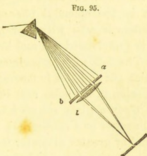
Combination of two homogeneous colours.
