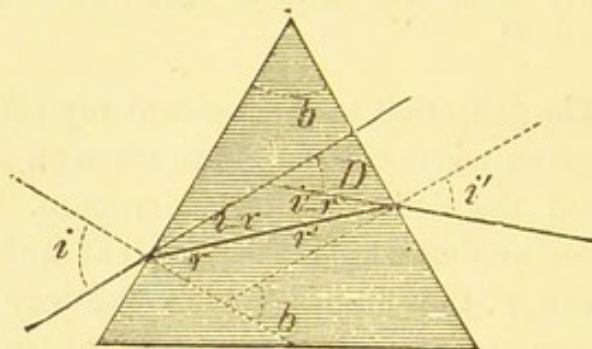
Passage of a ray of light through a prism.
