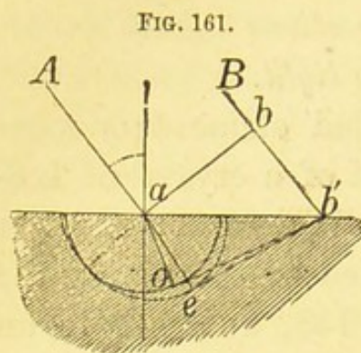
Huyghens' construction of double refraction.
