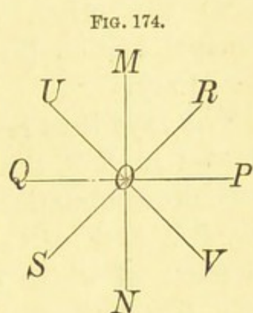
Decomposition of vibrations.
