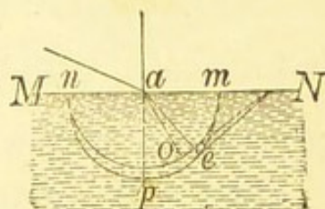
Double refraction. Second case.
