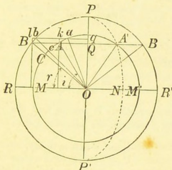
Theory of the rainbow.
