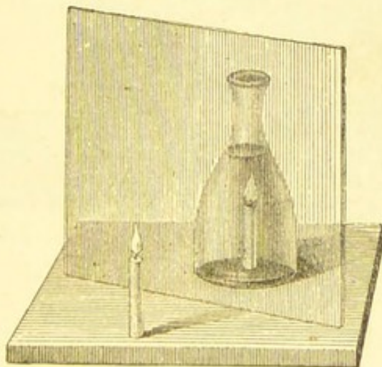
Mirror-image in a transparent plate of glass.
