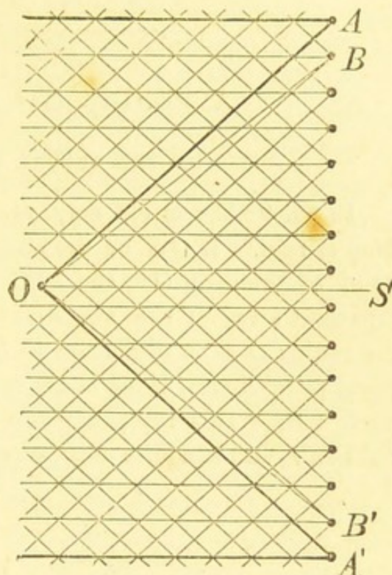
Mode of formation of the rainbow.
