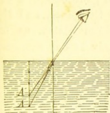
Apparent position of a point situated beneath the surface of the water.
