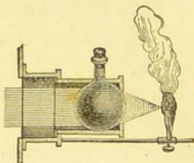
Action of the invisible thermotic rays.
