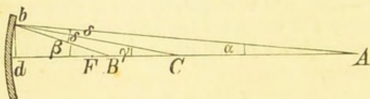
Determination of the position of conjugate points.
