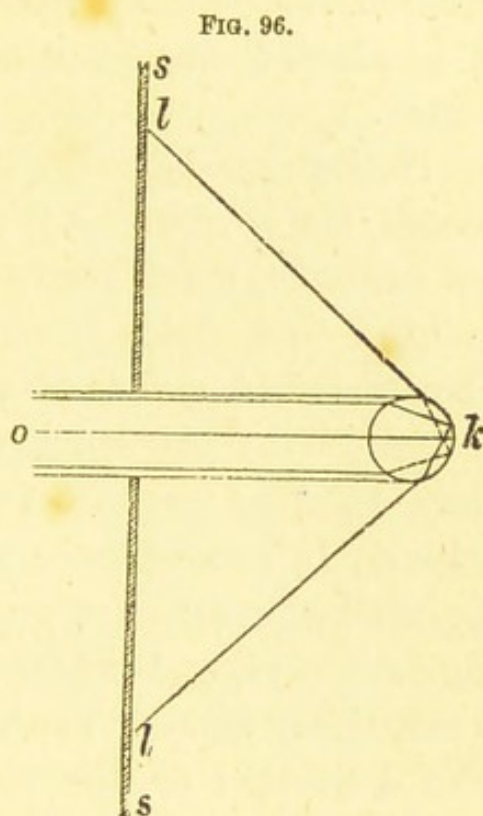
Refraction and internal reflexion in a rain-drop.
