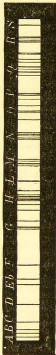
FIG. 123.—Solar spectrum with the ultra-violet portion.
