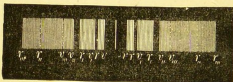
Diffraction phenomena through a grating.
