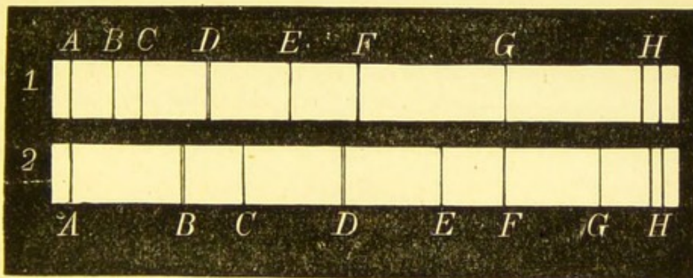
Comparison of the prismatic with the grating spectrum.
