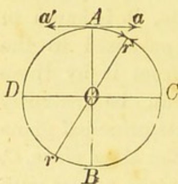
Combined effect of two opposite circular vibrations.
