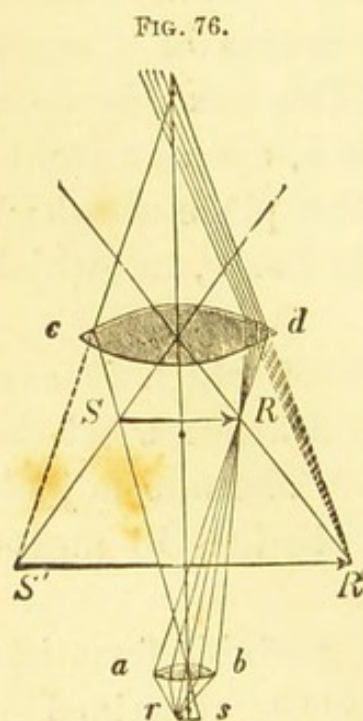
Action of the Microscope.
