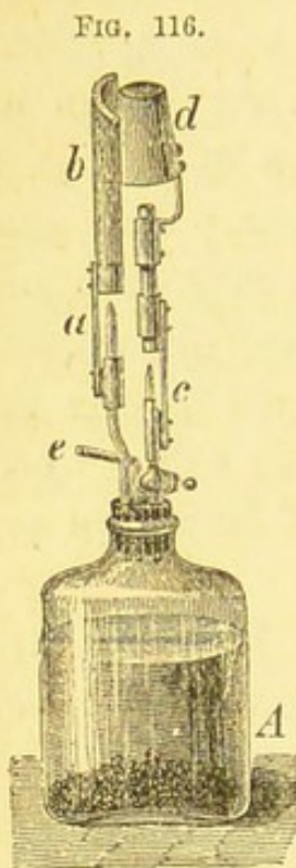
Bunsen's apparatus for the absorption of Sodium light.
