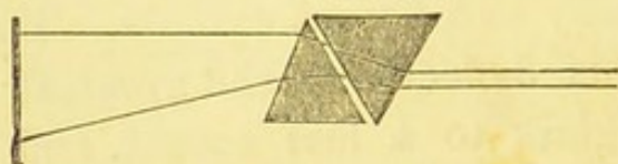
Combination of two similar prisms without deflection and without dispersion.
