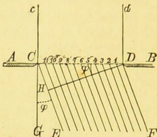
Explanation of diffraction taking place through a slit.
