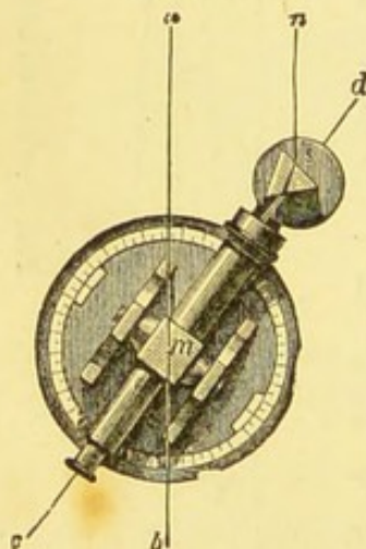
Instrument for measuring the prismatic deflection.
