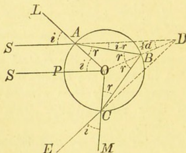
Refraction and internal reflexion in a drop of water.
