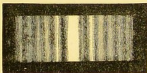
Diffraction or inflection image of a narrow slit.
