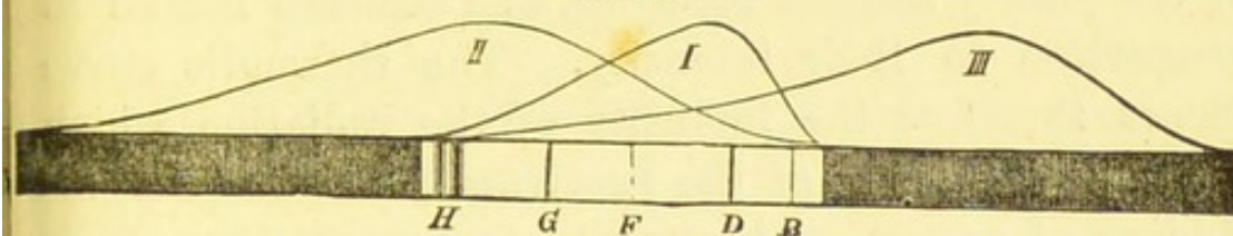
Light, heat, and photographic action of the solar spectrum.
