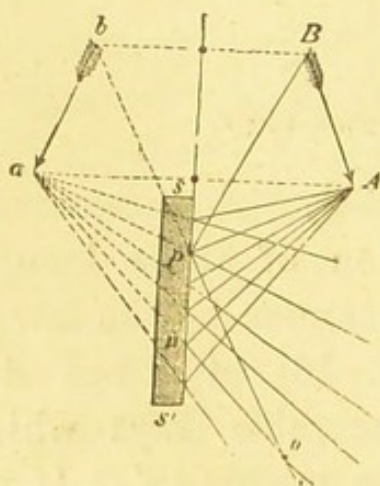
Production of the image in a mirror.
