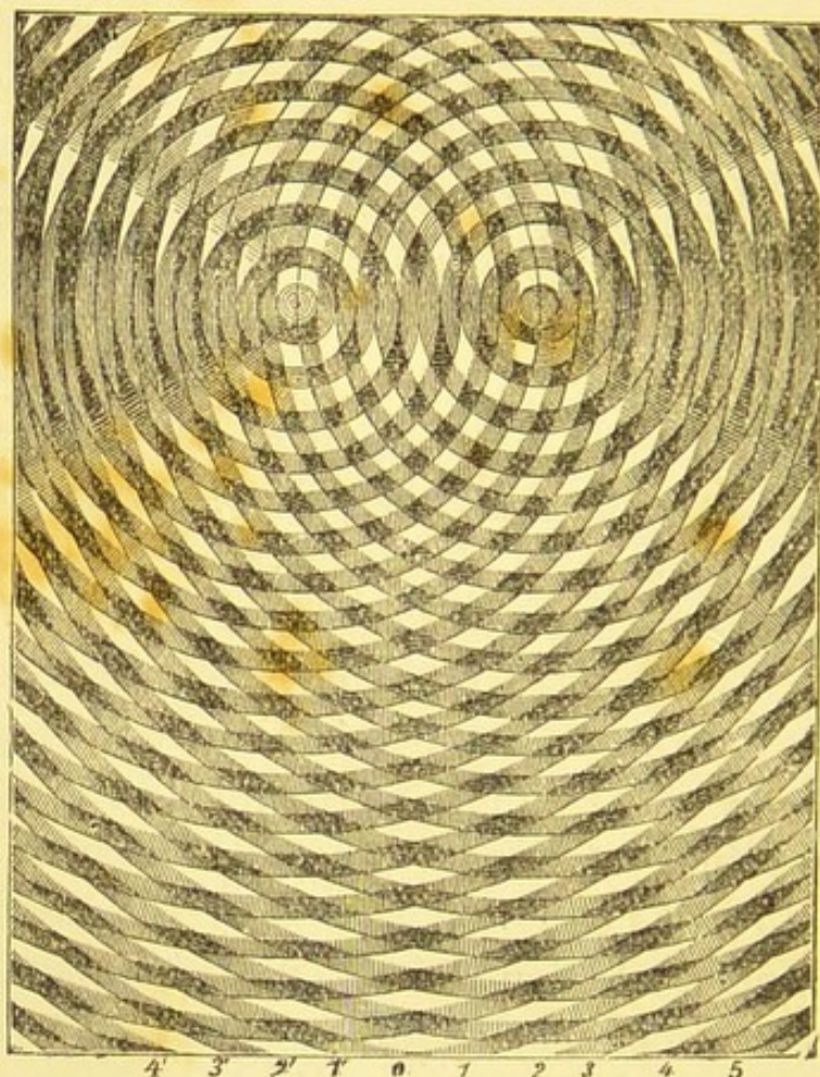
Interference of two systems of waves.
