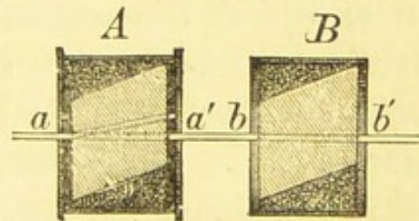
Two rhombohedra of Iceland spar.
