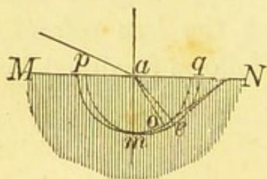
Double refraction. Third case.
