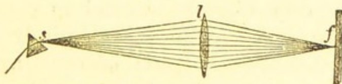
Combination of the colours of the spectrum to form white light.
