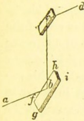
Two polarising mirrors.
