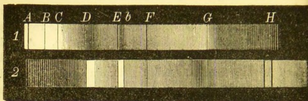
Absorption and fluorescing spectrum of Naphthalin red.
