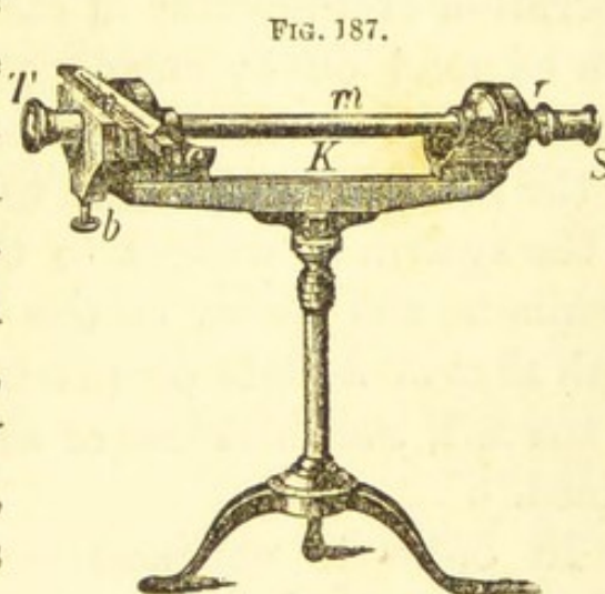
Soleil's Saccharimeter.
