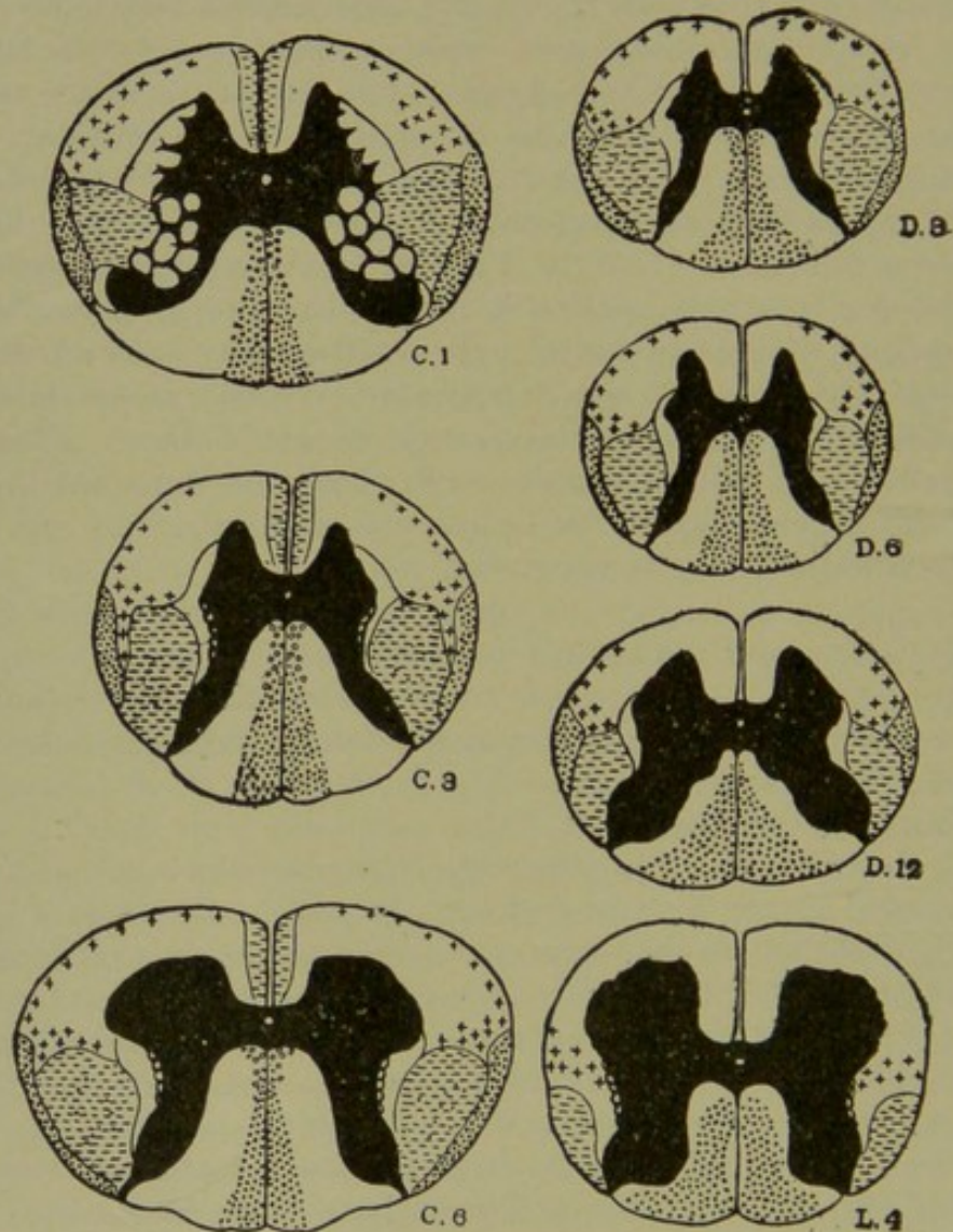
FIG. 71.—Diagram of the elements of the white substance at various levels of the spinal cord. (Modified from Flechsig.) The pyramidal tracts are shaded by short horizontal lines; the direct cerebellar tract by dots; the posterior median column by dots, as it degenerates in disease of the lowest part of the cord or of the nerves of the cauda equina; the small circles in the forepart of this column indicate the area which degenerates in disease of the cervical enlargement. The antero-lateral ascending tract is shown by crosses. The anterior ground-fibres, lateral limiting layer, and postero-external column are left white. Fig. 66 should be compared with this.
