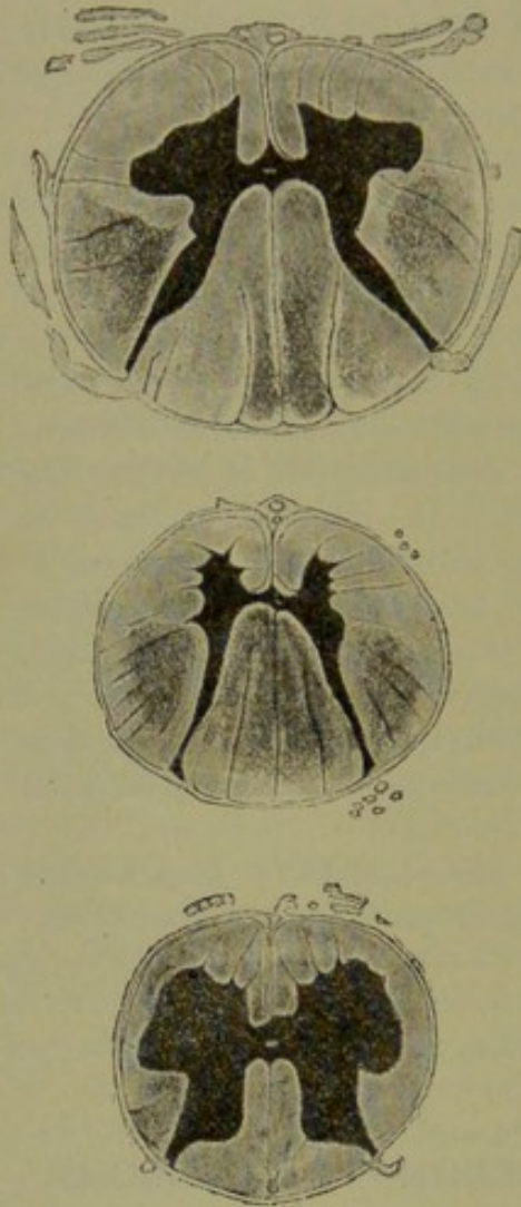
FIG. 136.—Sclerosis in pellagra (Tuzek). The darkly shaded areas indicate the sclerosis.
