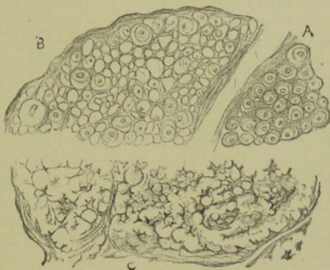
FIG. 143.—Hereditary ataxy; degeneration of posterior nerve-roots (from the same case as Fig. 142). A, normal anterior root, for comparison. B, posterior root, partially degenerated; a few normal nerve-fibres are seen, but most of the spaces which should contain nerve-fibres are empty. C, posterior root, totally degenerated, probably by a more acute process than that of B, since there is some destruction of the septa and increase of amorphous connective tissue. The products of degeneration are rendered invisible by the mode of preparation. (Compare C with the similar changes in a totally degenerated peripheral nerve shown in Fig. 59 B, p. 165.)
