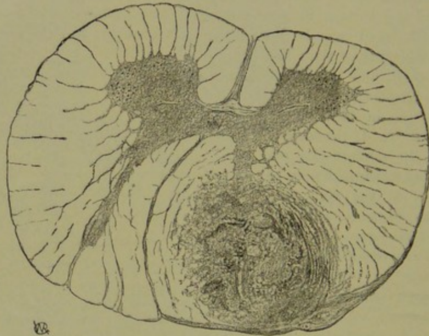
FIG. 182.—Syphiloma in the spinal cord, occupying the position of the posterior cornu and adjacent parts of the posterior and lateral columns, in the lower cervical region. The tumour presented the usual combination of grey translucent, and yellow cheesy areas. A second similar, but much smaller tumour existed higher up. The symptoms were complicated by hemiplegia, &c., of cerebral origin, due to a gumma in the brain. Paralysis with rigid flexor contracture of the left arm and leg were apparently due to the growth. The disease was certainly syphilitic, but it is noteworthy that it had developed during continuous treatment by full doses of iodide, which had entirely removed earlier symptoms, but to which the system had apparently become accustomed.
