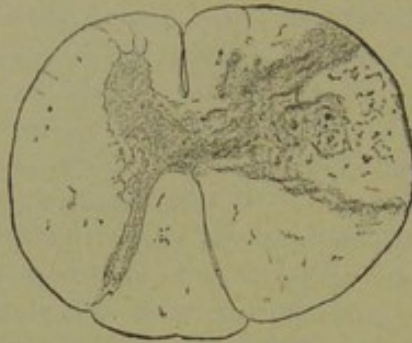
FIG. 84.—Section of spinal cord between the second and third cervical nerves, contused by gunshot injury.
