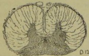
FIG. 125.—Locomotor ataxy involving the legs only. Sclerosis of the whole posterior columns in the lumbar region, gradually becoming limited, in the lower dorsal region, to the root-zone and posterior median column. The latter only is affected in the upper half of the cord (ascending degeneration). There is also conspicuous degeneration in the antero-lateral ascending tract. This is rather greater on the left side, while the post.-median degeneration is greater on the right, in harmony with the fact that the latter consists of fibres which do not decussate.
