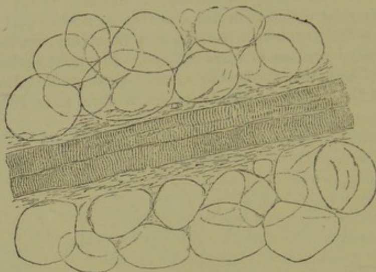
FIG. 166.—Gastrocnemius muscle; two nearly normal muscular fibres, accompanied by fibrous tissue, surrounded by fat-cells.
