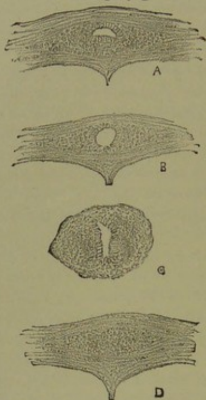
FIG. 82.—Central canal in normal cords. It has the form of a transverse slit in A, a vertical slit in C (from the conus medullaris ), while in B it is circular. In each it is lined by columnar epithelium and surrounded by cellular elements, rounded, or angular from compression, mingled with granules. In D, which is from the same spinal cord as C, the position of the canal is occupied by a mass of nuclear tissue.
