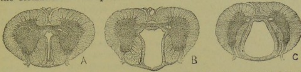
FIG. 184.—Syringomyelia, from a child two years old, with encephalocele and absence of cerebellum. (After Leyden.) In A, cervical region, the central canal is large, lined with epithelium, and from it a medial fissure extends backwards nearly to the periphery of the cord, limited by a layer of homogeneous tissue, more abundant at the posterior limit. In B, lower down, the fissure is enlarged to a cavity of considerable size, while in C it is still larger, and the posterior columns are reduced to a narrow zone between the layer of tissue which bounds the cavity and the grey substance.
