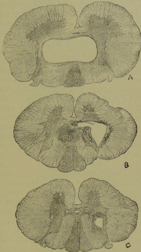
FIG. 187.—Syringomyelia, from a case in which there were tumours in the dorsal region of the cord, the cauda equina, and the pons Varolii. A, mid-cervical region. A large oval cavity lies behind the grey commissure, surrounded by a narrow wall, chiefly composed of fine fibres, but with a wavy membrane on the inner surface. In front of the posterior commissure, an oval group of nuclei has the aspect of an obliterated central canal. A few short processes extend from the wall of the cavity into the posterior columns. There is secondary ascending degeneration of the post. med. cols., right direct pyramidal tract, and ascending antero-lateral tract in all the sections. B, first dorsal. Behind the posterior commissure is a growth consisting of small cells, round and fusiform, the latter with round nuclei. It contains many vessels with thickened walls. A fringe of fine processes extends from it into the posterior columns. An irregular cavity occupies, on the right side, the posterior half of the grey matter, which is reduced to a narrow layer around the cyst. This is lined by a delicate nucleated membrane, outside which is a thicker membrane, lying in folds, the section of which is thus sinuous. Outside this again is a small-celled growth similar to that behind the commissure. In C, a little lower, this cavity is smaller, the sinuosities of the wall greater, and the growth outside it more abundant. (Still lower the area was entirely occupied by the growth.) In the posterior commissure there is only a quantity of loose nucleated tissue in the situation of the growth.*
