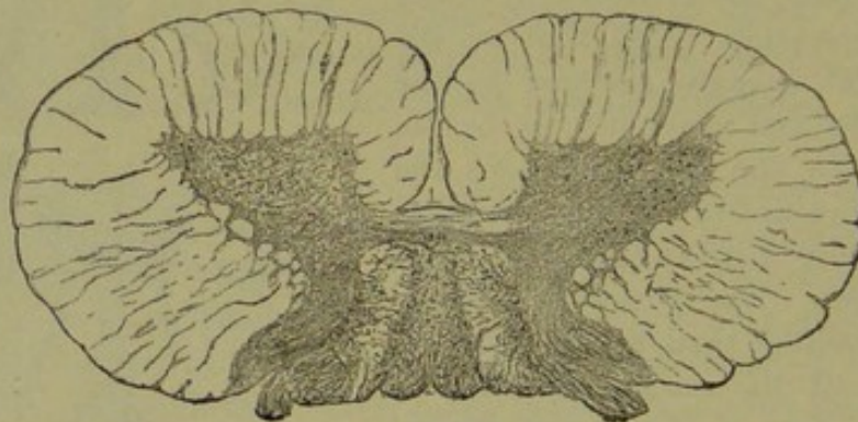
FIG. 126.—Tabes with ataxy of the arms as well as the legs. Section of cord in cervical region, showing sclerosis of the post.-med. column and root-zone of post.-ext. col. Degeneration of left ant. cornu.
