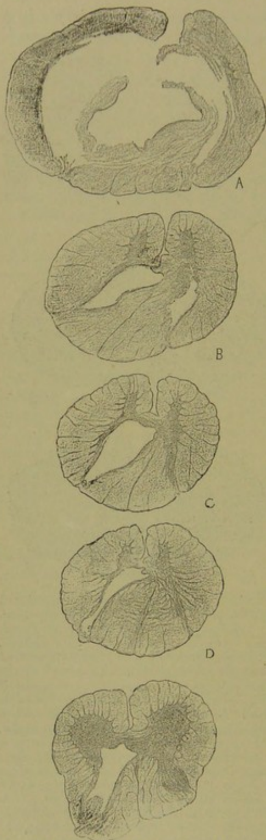
FIG. 188.—Sections of a spinal cord in which a cavity existed throughout its length. Hæmorrhage in the cervical region was the immediate cause of death. The extravasation had there distended the cord (A), and had burst into the cavity, which was filled with blood. A smaller cavity existed in the right cornu, in the upper dorsal region (B). In most parts the inner surface was slightly irregular, as if produced by breaking down of the tissue, but near the position of the central canal a sinuous membrane existed in places, without, however, any epithelial covering.
