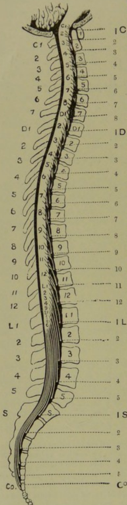
FIG. 64.—Diagram (framed from an original investigation) showing the relation of the vertebral spines to their bodies and to the origin of the several nerve-roots. It will be seen that the ends of the vertebral spines are opposite the middle of their own bodies only in the lumbar region; they correspond to the lower edge of their own bodies in the cervical and the first two dorsal vertebræ, and to the upper part of the body below in the rest of the dorsal region. Each cervical spine is nearly opposite the lower roots of the nerve below; the vertebra prominens is opposite the first dorsal roots, and from the 3rd to the 10th dorsal the spines correspond to the second root below; the 11th spine corresponds to the 1st and 2nd lumbar nerves, the 12th to the 3rd, 4th, and 5th; the 1st lumbar to the 1st, 2nd, and 3rd sacral nerves, while the tip of the cord is opposite the upper part of the 2nd lumbar.
