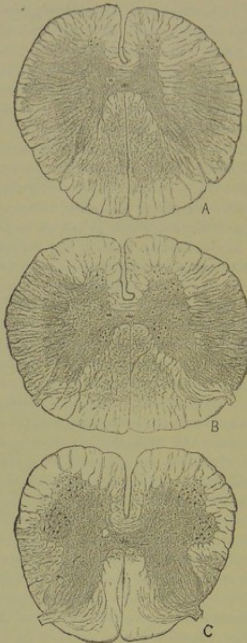
FIG. 135.—Ataxic paraplegia, combined lateral and posterior sclerosis. A, upper dorsal; B, last dorsal; C, mid-lumbar. The posterior columns are free from sclerosis in C, except in their anterior parts; in B the disease involves the middle and anterior parts of both post.-med. and post.-ext. columns except in the neighbourhood of the neck of the horn; in A the sclerosis is slighter and is confined to the middle three fifths of these columns. The sclerosis of the lateral columns in C is limited, on the right, to the pyramidal tract, on the left it extends in front of this; in B it is very dense in the whole lateral column, involving not only the pyramidal tract but the limiting layer, and part of the "mixed zone;" in A it is similar in extent but slighter in degree. There is some increase of tissue throughout the anterior columns, and a focus of sclerosis near the anterior fissure, on the right in A and B, on both sides in C.†
