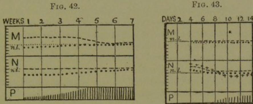
FIG. 42.—Slight neuritis: power regained during the second week. Deg. react. in muscle distinct on eighth day, lessening during second and third weeks. Nerve: lowered faradic, normal voltaic irritability.
