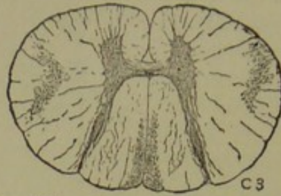
FIG. 75.—Degeneration of the antero-lateral ascending tract in a case of locomotor ataxy (q. v. figure), showing its position in the upper cervical region, where the direct cerebellar tract passes outside it into the restiform body.
