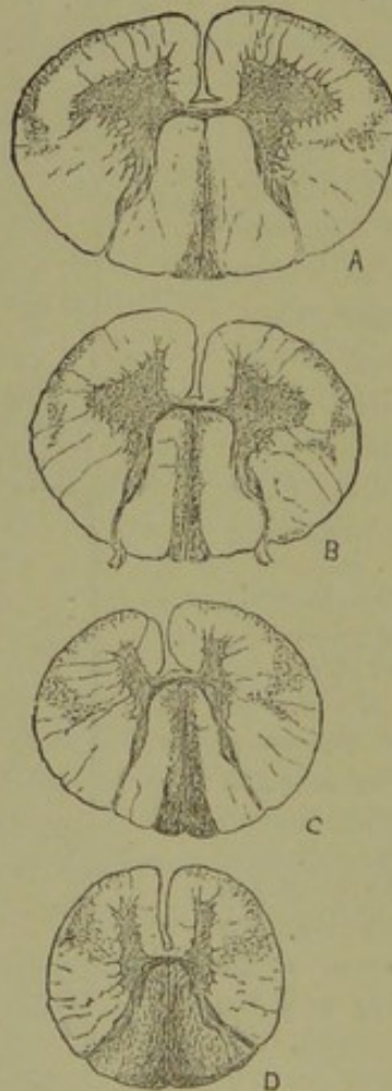
FIG. 76.—Ascending degeneration in the postero-medial column and antero-lateral ascending tract. The cord was crushed at the first lumbar segment.
