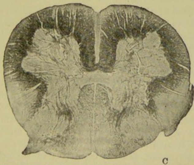
FIG. 137.—Showing sclerosis occurring in a case of profound anæmia. The sclerotic areas are decolourised. Note in the lumbar cord the comparative escape of the septo-marginal and cornu-commissural tracts. A, cervical. B, dorsal. C, lumbar.
