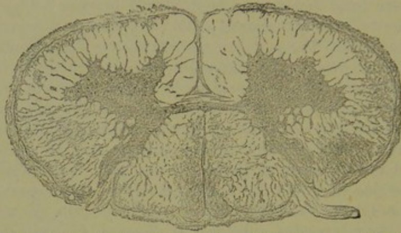
FIG. 129.—Tabes. Chronic meningitis. Cervical region. Sclerosis of post-median columns and slight diffuse sclerosis of the cord, least in ant. cols., dense in the right lateral column. Thickened pia mater, and damage to subjacent superficial layer of the cord.
