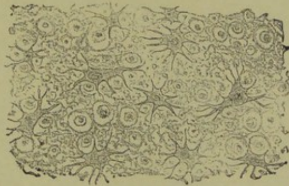
FIG. 100.—Subacute disseminated myelitis; part of the posterior column. Nerve-fibres separated by granular material and products of degeneration, and by numerous large spider cells. The myelitis in this case was attended by optic neuritis. (From a section lent by Dr. Dreschfeld.)
