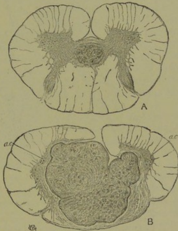
FIG. 181.—Tumour of spinal cord, springing from the tissue around the central canal. A, upper part of the tumour in the middle of the cervical region; the growth is here within the posterior commissure. B, section through the largest part of the tumour, which occupies the whole central region of the cord. The vertical extent was 2 cm. It was a sarcoma composed chiefly of spindle-cells arranged in fasciculi and in concentric layers. The patient was suffering also from a cerebral tumour causing hemiplegia, and the spinal growth, which apparently developed rapidly during the final period of palsy and prostration, was not suspected during life.
