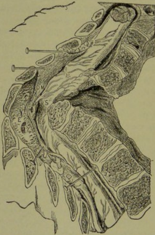
FIG. 92.—Caries of the spine, mid-dorsal region. The spinal cord is much narrowed and discoloured at s from compression between the displaced bone and a mass of inflammatory products, E , outside the dura mater, DM , the inner surface of which is normal. (After Leyden.)
