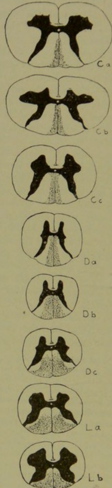
FIG. 77.—Degeneration after injury to the cauda equina. C a, b, c, upper middle and lower cervical; D a, upper; b, c, lower dorsal; L a, upper; and L b, middle lumbar region. (After Schultze.)
