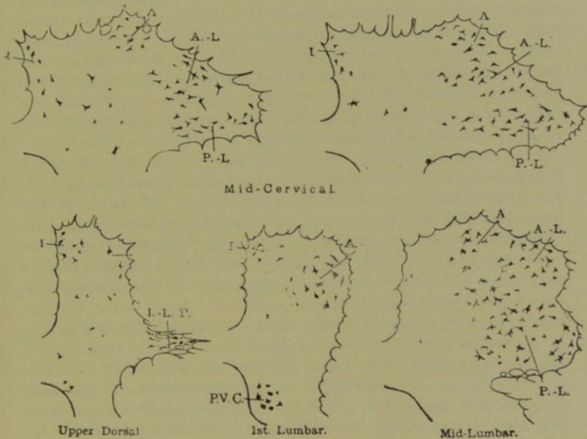
FIG. 70.—Diagrams of the groups of nerve-cells in the anterior cornu. Groups:—I., inner or medial; A., anterior; A.-L., antero-lateral; P.-L., postero-lateral; I. L. P., intermediate lateral process; P. V. C., posterior vesicular column or tract. The two mid-cervical sections are only a few millimetres apart, and show how the anterior group, separate in the one, may be blended with the antero-lateral group in a neighbouring part of the cord.
