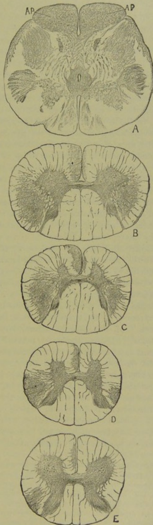
FIG. 154.—Progressive muscular atrophy. A, medulla oblongata; degeneration of the anterior pyramids, A P. B, cervical, C, first dorsal, D, first lumbar, E, mid-lumbar sections. The nerve-cells have disappeared from the anterior cornua, except in E, in which a few remain. There is complete degeneration of the pyramidal tracts, anterior and lateral. The decussation at the medulla was unequal in this case; of the left pyramid fewer fibres crossed than of the right, and hence the left anterior pyramidal tract is larger, while the right lateral tract is smaller than normal, and, moreover, has ceased at the middle of the lumbar enlargement, to which the left anterior tract extends.*
