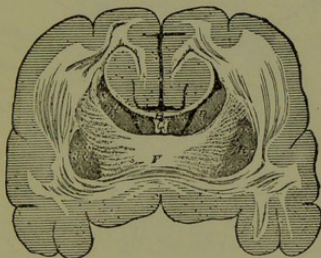
Fig. 29.—Frontal section of brain of kangaroo ( Macropus major ) (after Flower). B , body of corpus callosum (connecting the hippocampi ; F , anterior commissure ; G , septal area ; R , corpus striatum.
