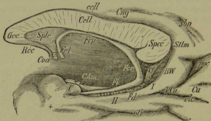
Fig. 28 (after Obersteiner).— Ccl , corpus callosum; Gcc , genu of corpus callosum; Coa , anterior commissure; Fcl , columns of fornix; Fcr , crus of fornix; CAm , cornu ammonis; Tf , tuberculum fascia dentata; BW , Balkenwindung (splenial convolution); I , isthmus gyri fornicati; U , uncus; PCu , pedunculus cunei; Sbp , sulcus subparietalis; clc , fissura calcarina; Rcc , rostrum of corpus callosum; Spcc , splenium of corpus callosum; Splc , septum lucidum; Fcp , body of fornix; Fi , fimbria; Fd , fascia dentata; Stlm , stria longitudinalis medialis; g , gyrus cinguli; H , gyrus hippocampi; Cu , cuneus; ccll , sulcus corporis callosi; poc , fissura parieto-occipitalis; oti , sulcus occipito-temporalis inferior.
