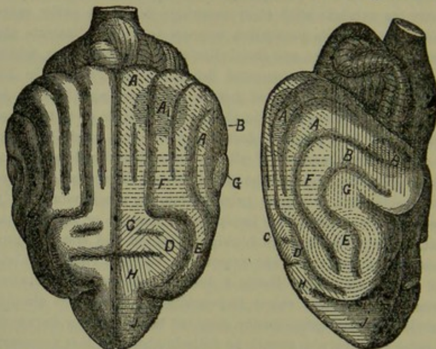
Fig. 14.—Cortical centres of the dog, after Munk. A, Visual area; B, auditory area; C to J, tactile sensory area ( Fühlsphäre ); D, fore-limb region; C, hind-limb region; E, head region; F, eye region; G, ear region; H, neck region; J, trunk region.
