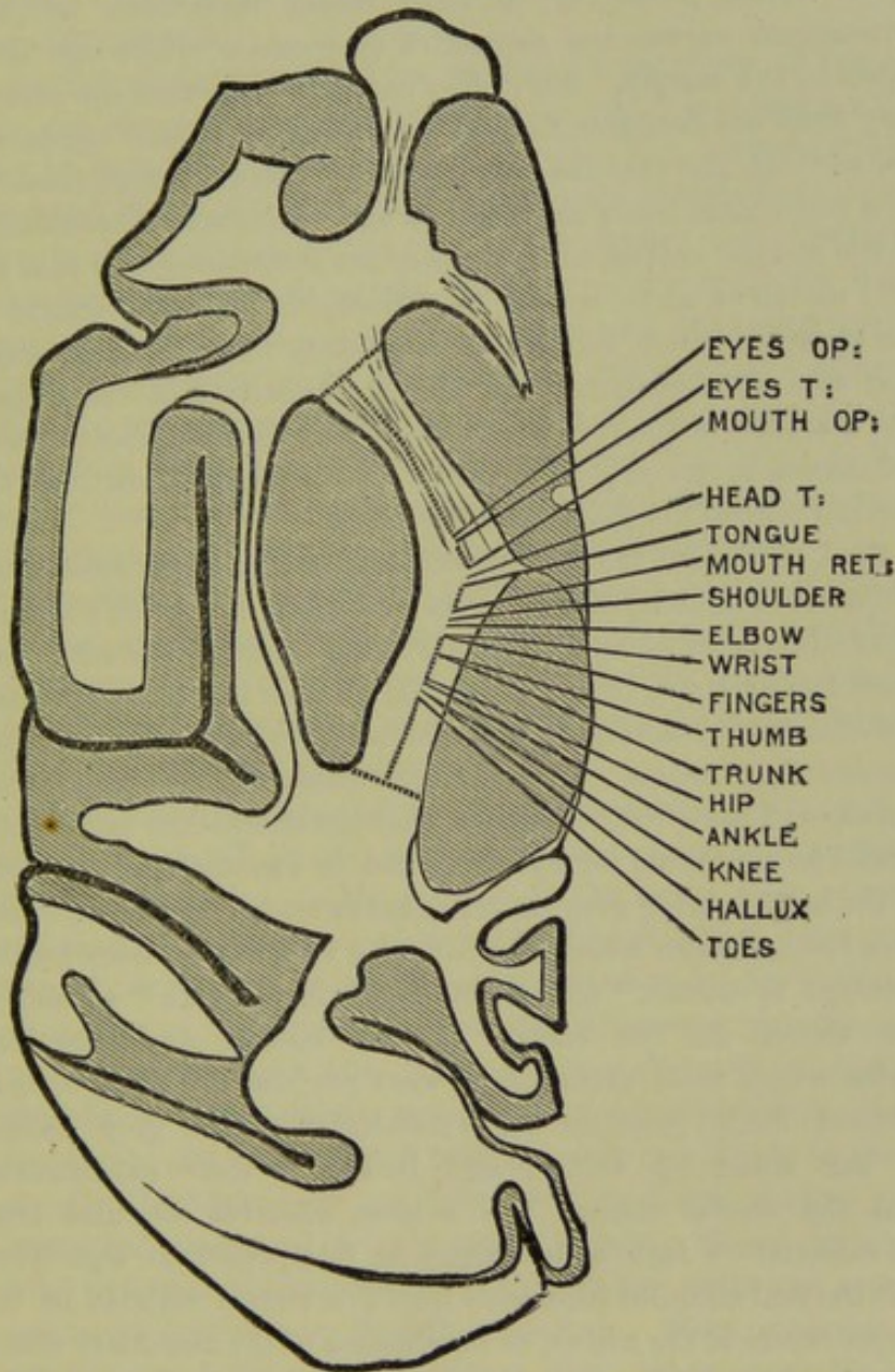
Fig. 4.—Arrangement of the motor fibres of the internal capsule, according to Beevor and Horsley.
