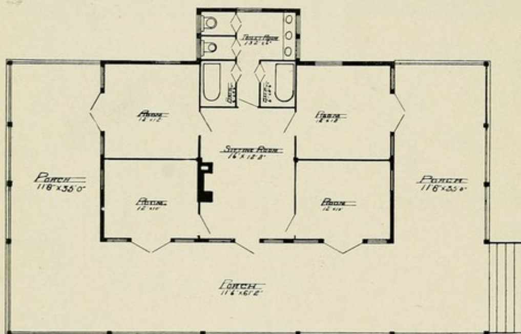
No. 99.—Association Sanatorium, Louisville, Ky. D. X. MURPHY & BROTHER, ARCHITECTS. COTTAGE. VIEW OF FRONT AND SIDE ELEVATION AND FLOOR PLAN. CAPACITY, 12 PATIENTS. ESTIMATED COST, $2,250.
