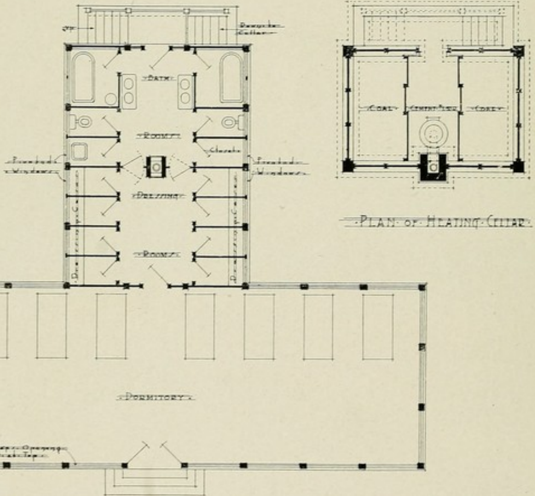
No. 83.—Eudowood Sanatorium, Towson, Md. ARCHER & ALLEN, ARCHITECTS. LEAN-TO. VIEW OF FRONT ELEVATION AND FLOOR PLANS. CAPACITY, 8 PATIENTS. ESTIMATED COST, $4,000. * (See illustrations 22 and 61 for further description of this institution.)
