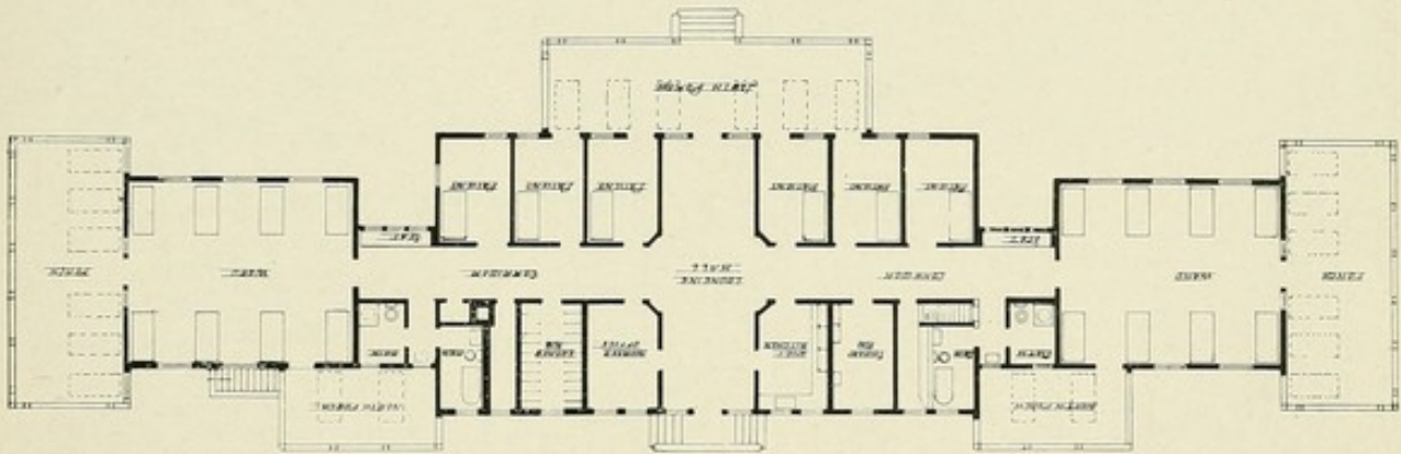
No. 65.—Georgia State Sanatorium, Alto, Ga. SCOPES & FEUSTMANN, AND WALTER W. JUDELL, ASSOCIATED ARCHITECTS. INFIRMARY BUILDING. VIEW OF FRONT ELEVATION, AND FLOOR PLAN. CAPACITY, 24 PATIENTS. COST, $18,000. (See illustrations 4 and 78 for further description of this institution.)
