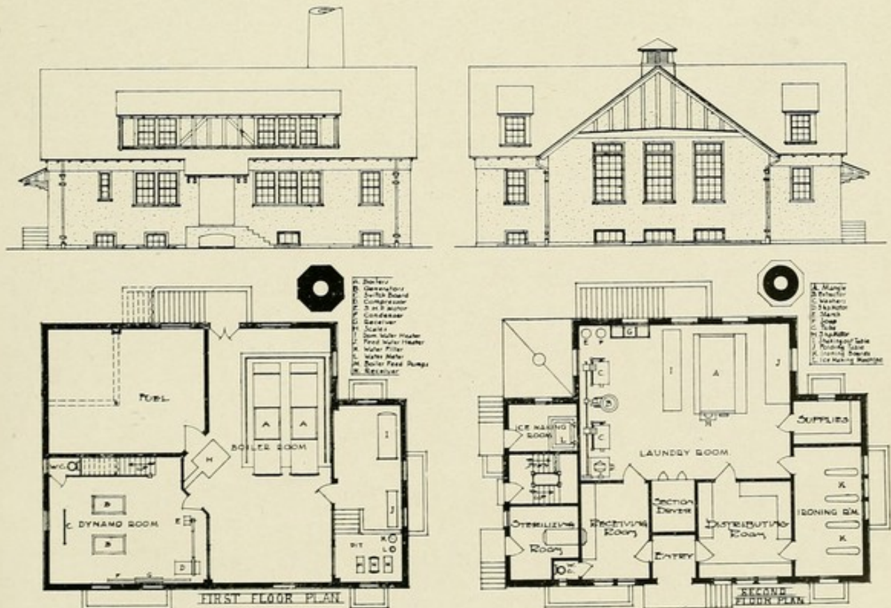
No. 19.—Preventorium for Children, Farmingdale, N. J. SCOPES & FEUSTMANN, AND WALTER W. JUDELL, ASSOCIATED ARCHITECTS. POWER HOUSE AND LAUNDRY. FRONT AND SIDE ELEVATIONS WITH FIRST AND SECOND FLOOR PLANS. (See illustrations 12, 27 and 95 for further description of this institution.)
