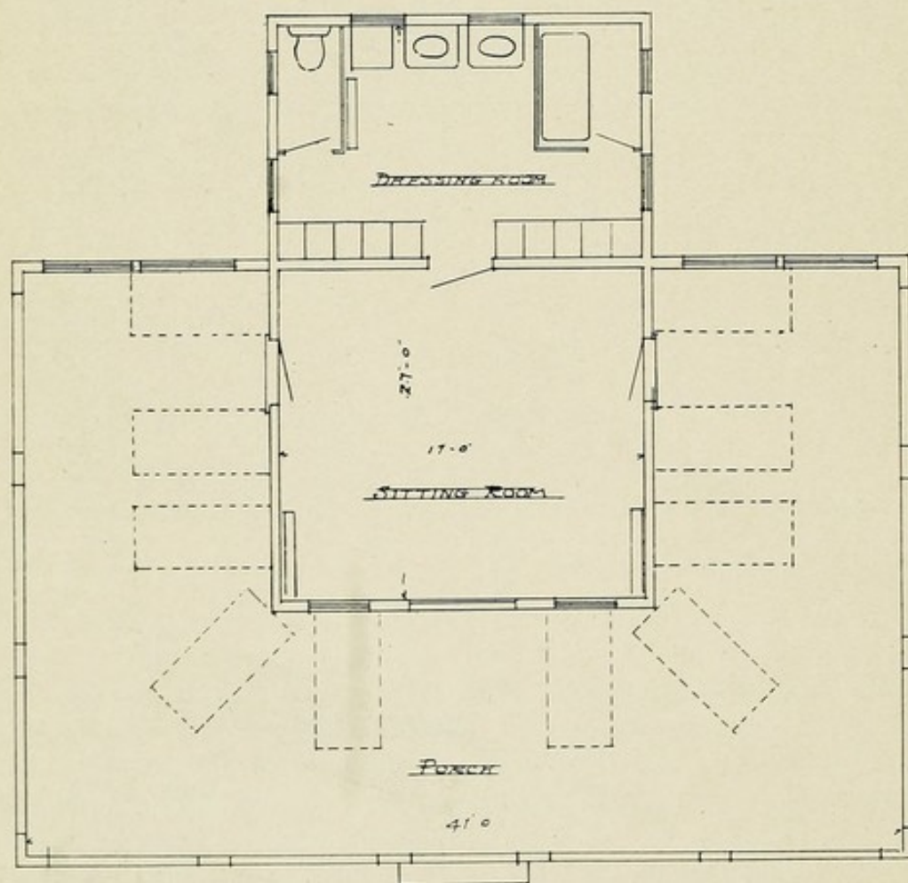
No. 103.—Iowa State Sanatorium, Oakdale, Ia. DESIGN BY DR. H. E. KIRSCHNER. H. F. LIEBBE, ARCHITECT. COTTAGE. VIEW OF FRONT AND SIDE ELEVATION AND FLOOR PLAN. CAPACITY, 8 PATIENTS. ESTIMATED COST, $1,500. (See illustrations 24, 29 and 84 for further description of this institution.)
