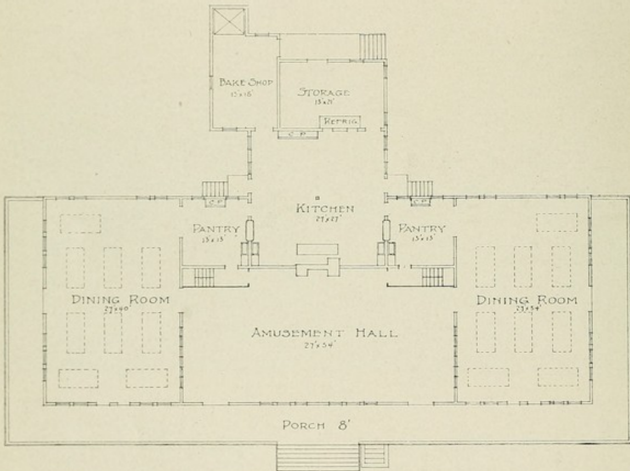
No. 30.—Catawba Sanatorium, Catawba, Va. DESIGNED BY DR. ENNION G. WILLIAMS. SERVICE BUILDING, CONTAINING AN AMUSEMENT HALL. FRONT ELEVATION AND FLOOR PLAN. SERVICE CAPACITY, 70 PATIENTS. ESTIMATED COST, $10,000. (See illustrations 17, 69 and 80 for further description of this institution.)
