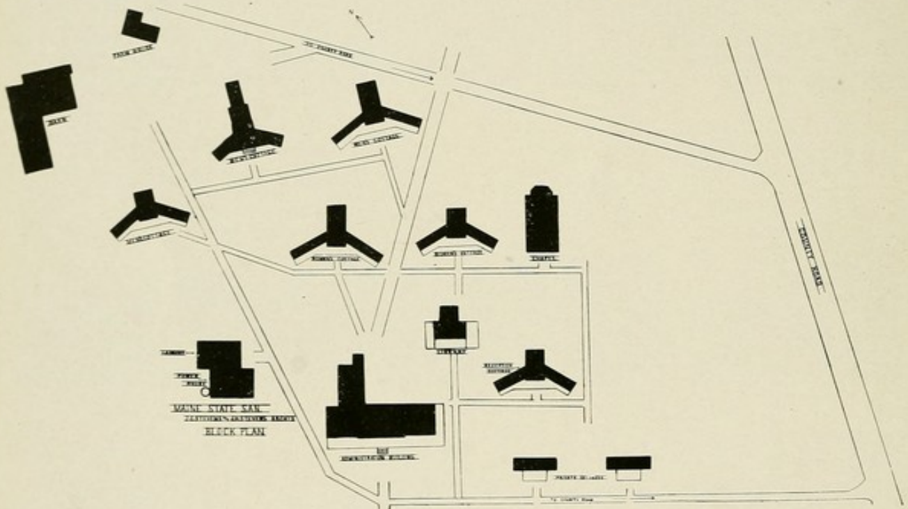
No. 11.—Maine State Sanatorium, Hebron, Me. T. C. STEVENS AND J. H. STEVENS, ARCHITECTS. VIEW AND BLOCK PLAN SHOWING METHOD OF GROUPING PAVILIONS IN THE REAR OF THE ADMINISTRATION BUILDING AND POWER HOUSE. CAPACITY, 100 PATIENTS. ESTIMATED COST, $150,000. (See illustrations 23 and 58 for further description of this institution.)
