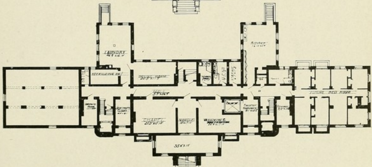
No. 39.—Franklin County Tuberculosis Hospital, Columbus, Ohio. HOWARD & MERRIAM, ARCHITECTS. FRONT ELEVATION AND FLOOR PLANS. CAPACITY, 100 PATIENTS. ESTIMATED COST, $85,000.
