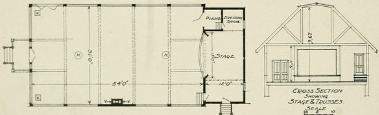
No. 13.—Adirondack Cottage Sanitarium, Saranac Lake, N. Y. THE AMUSEMENT PAVILION. VIEWS OF THE EXTERIOR AND INTERIOR WITH FLOOR PLAN AND CROSS SECTION. (See illustrations 63, 98, 104 and 109 for further description of this institution.)
