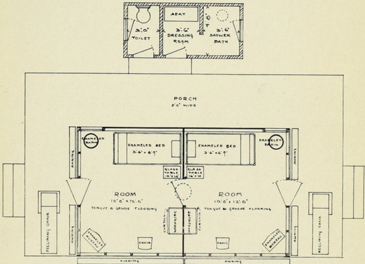
No. 106.—Barlow Sanatorium, Los Angeles, Cal. DESIGNED BY DR. W. JARVIS BARLOW. COTTAGE. VIEW OF FRONT AND SIDE ELEVATIONS AND FLOOR PLAN. CAPACITY, 2 PATIENTS. ESTIMATED COST, $500.
