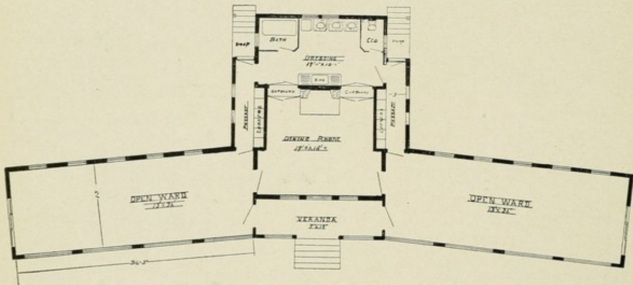
No. 89.—Iowa State Hospital, Mt. Pleasant, Ia. H. F. LIEBBE, ARCHITECT. LEAN-TO. FRONT ELEVATION AND FLOOR PLAN. CAPACITY, 12 PATIENTS. ESTIMATED COST, $3,000.
