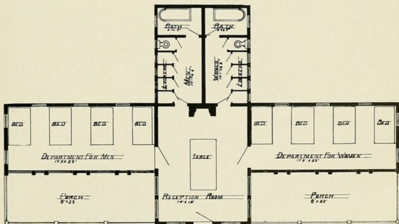
No. 76.—Delaware State Sanatorium, Wilmington, Del. J. & M. KENNEDY, ARCHITECTS. HEBREW SOCIETY LEAN-TO. VIEW OF FRONT ELEVATION AND FLOOR PLAN. CAPACITY, 8 PATIENTS. ESTIMATED COST, $1,000.
