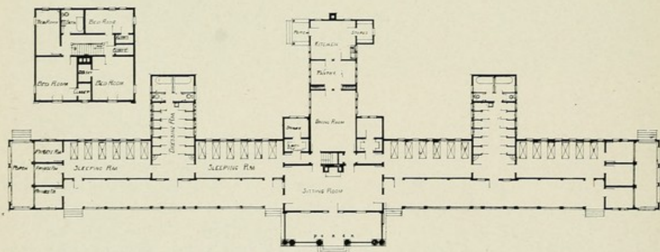
No. 61.—Eudowood Sanatorium, Towson, Md. ARCHER & ALLEN, ARCHITECTS. INFIRMARY BUILDING. VIEWS OF THE FRONT AND REAR ELEVATIONS. FLOOR PLANS. CAPACITY, 30 PATIENTS. ESTIMATED COST, $30,000. (See illustrations 22 and 83 for further description of this institution.)
