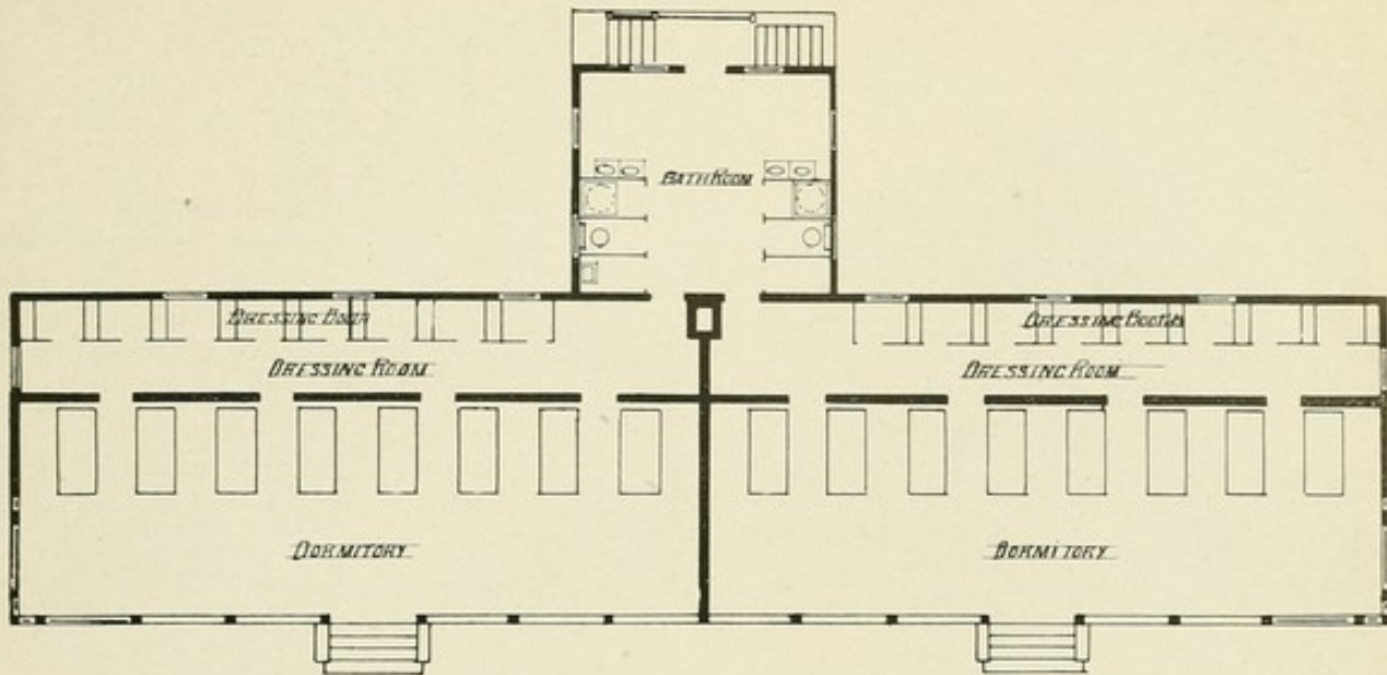
No. 78.—Georgia State Sanatorium, Alto, Ga. SCOPES & FEUSTMANN, AND WALTER W. JUDELL, ASSOCIATED ARCHITECTS. DESIGN FOR A LEAN-TO. FLOOR PLAN. CAPACITY, 16 PATIENTS. ESTIMATED COST, $2,500. (See illustrations 4 and 65 for further description of this institution.)
