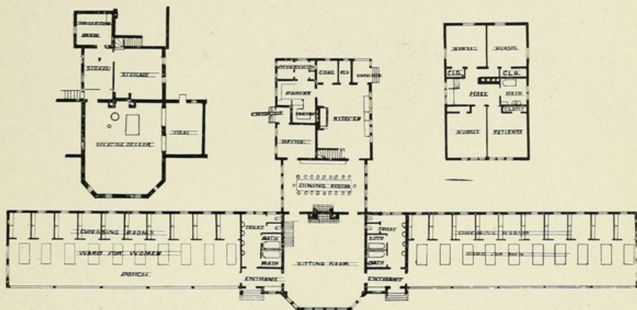
No. 42.—Association Sanatorium, Colorado Springs, Colo. N. VAN DEN AREND, ARCHITECT. ELEVATION AND FLOOR PLANS. CAPACITY, 24 PATIENTS. ESTIMATED COST, $25,000.
