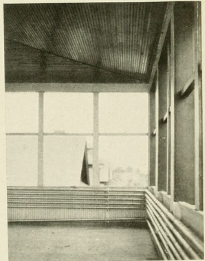
No. 47.—Isolation Hospital, Paterson, N. J. CHARLES E. WHITE, ARCHITECT. VIEW OF THE CORNER OF ONE OF THE PORCHES SHOWING METHOD OF HEATING FOR ADVANCED CASES BY STEAM PIPES. (See illustration 52 for further description of this institution.)
