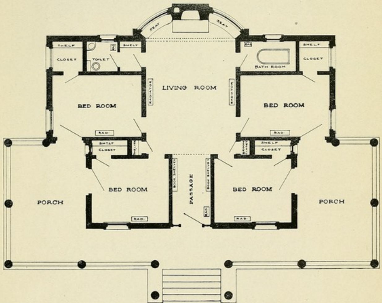
No. 109. —Adirondack Cottage Sanitarium, Saranac Lake, N. Y. SCOPES & FEUSTMANN, ARCHITECT NATHAN COTTAGE. VIEW OF FRONT ELEVATION AND FLOOR PLAN. CAPACITY, 4 PATIENT ESTIMATED COST, $5,000. (See illustrations 63, 98 and 104 for further description of this institu- tion.)
