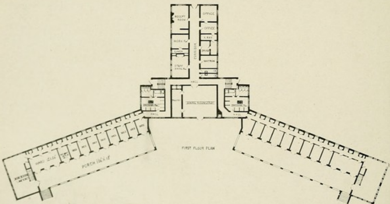
No. 43.—District Tuberculosis Hospital, Lima, Ohio. McLAUGHLIN AND HULSKIN, ARCHITECTS. VIEW OF FRONT AND REAR ELEVATIONS AND FLOOR PLANS. PRESENT CAPACITY, 28 PATIENTS. WINGS TO BE EXTENDED AS SHOWN IN FLOOR PLANS WITH A CAPACITY FOR 100 PATIENTS. (For plan of basement see illustration No. 20.) ESTIMATED COST, $100,000.
