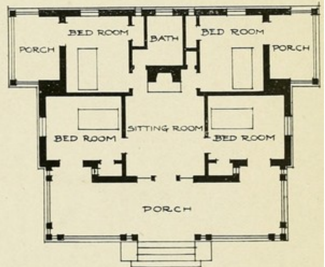
No. 104.—Adirondack Cottage Sanitarium, Saranac Lake, N. Y. SCOPES & FEUSTMANN, ARCHITECTS. WHEELER COTTAGE. VIEW OF FRONT ELEVATION AND FLOOR PLAN. CAPACITY, 4 PATIENTS. ESTIMATED COST, $4,000. (See illustrations 63, 98 and 109 for further description of this institution.)
