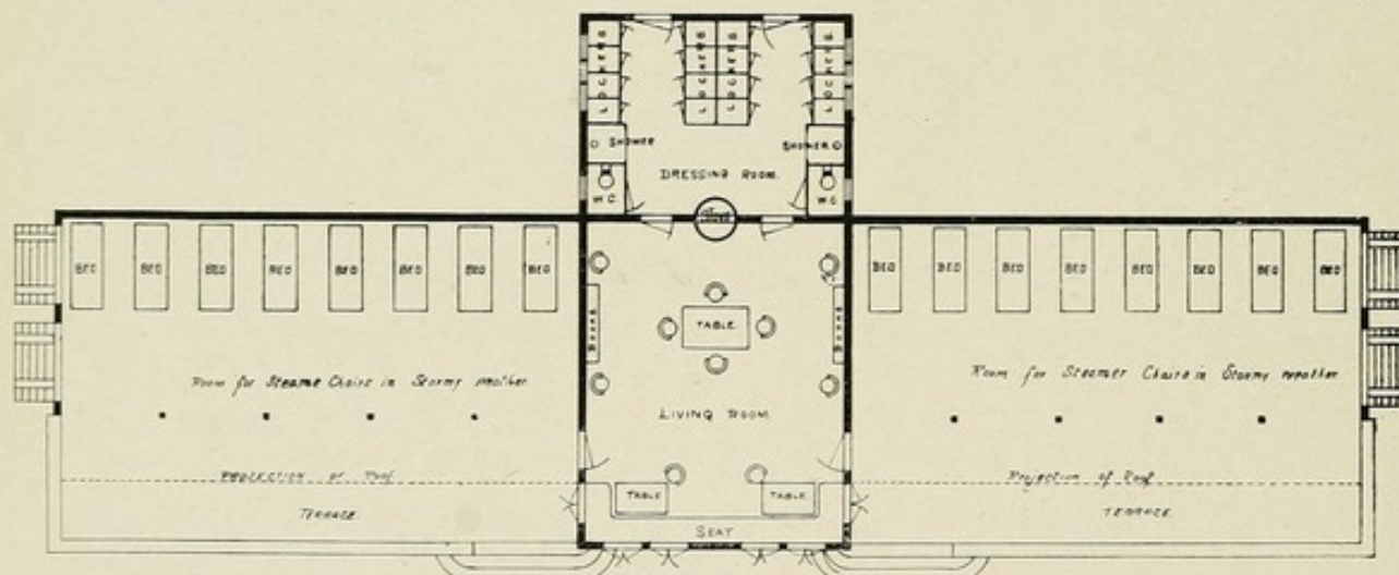
No. 73. —Loomis Sanatorium, Liberty, N. Y. ORIGINAL IMPROVED LEAN-TO. DESIGNED BY DR. HERBERT MAXON KING. VIEW OF FRONT ELEVATION AND FLOOR PLAN. CAPACITY, 16 PATIENTS. COST, $1,830. (See illustrations 1, 72, 91 and 108 for further description of this institution.)
