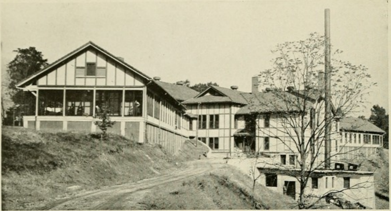
No. 18.—Waverly Hill Sanatorium, Waverly Hill, Ky. J. J. GAFFNEY, ARCHITECT. VIEW FROM THE REAR SHOWING A METHOD OF USING THE TOP AND SIDE OF A HILL IN ORDER TO OBTAIN A POSITION BELOW THE BUILDINGS FOR THE POWER PLANT. (See illustration 5 for further description of this institution.)
