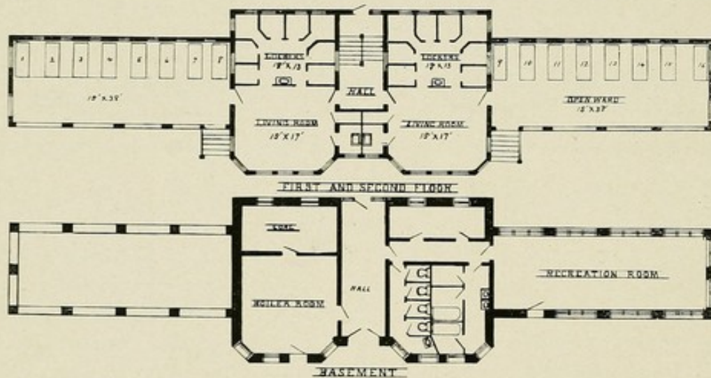
No. 94.—Municipal Sanatorium, Otisville, N. Y. DESIGNED BY DR. HERMANN M. BIGGS. JAMES D. BURT, ARCHITECT. LEAN-TO, No. 103. VIEW OF FRONT ELEVATION AND FLOOR PLANS. THE SPECIAL FEATURE OF THIS BUILDING IS AN ARRANGEMENT THAT FORMS THE PATIENTS INTO GROUPS OR UNITS BY SUPPLYING A SEPARATE LIVING ROOM AND TOILET APARTMENT IN CONNECTION WITH EACH PORCH. CAPACITY, 32 PATIENTS. COST, $9,000. (See Illustrations 14, 28, 59, 60, 85 and 101 for further description of this institution.)
