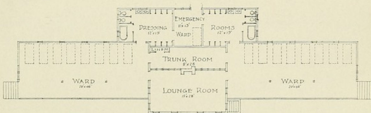
No. 80.—Catawba Sanatorium, Catawba, Va. DESIGNED BY DR. ENNION G. WILLIAMS. LEAN-TO. VIEW OF FRONT ELEVATION AND FLOOR PLAN. CAPACITY, 16 PATIENTS. ESTIMATED COST, $2,000. (See illustrations 17, 30 and 69 for further description of this institution.)
