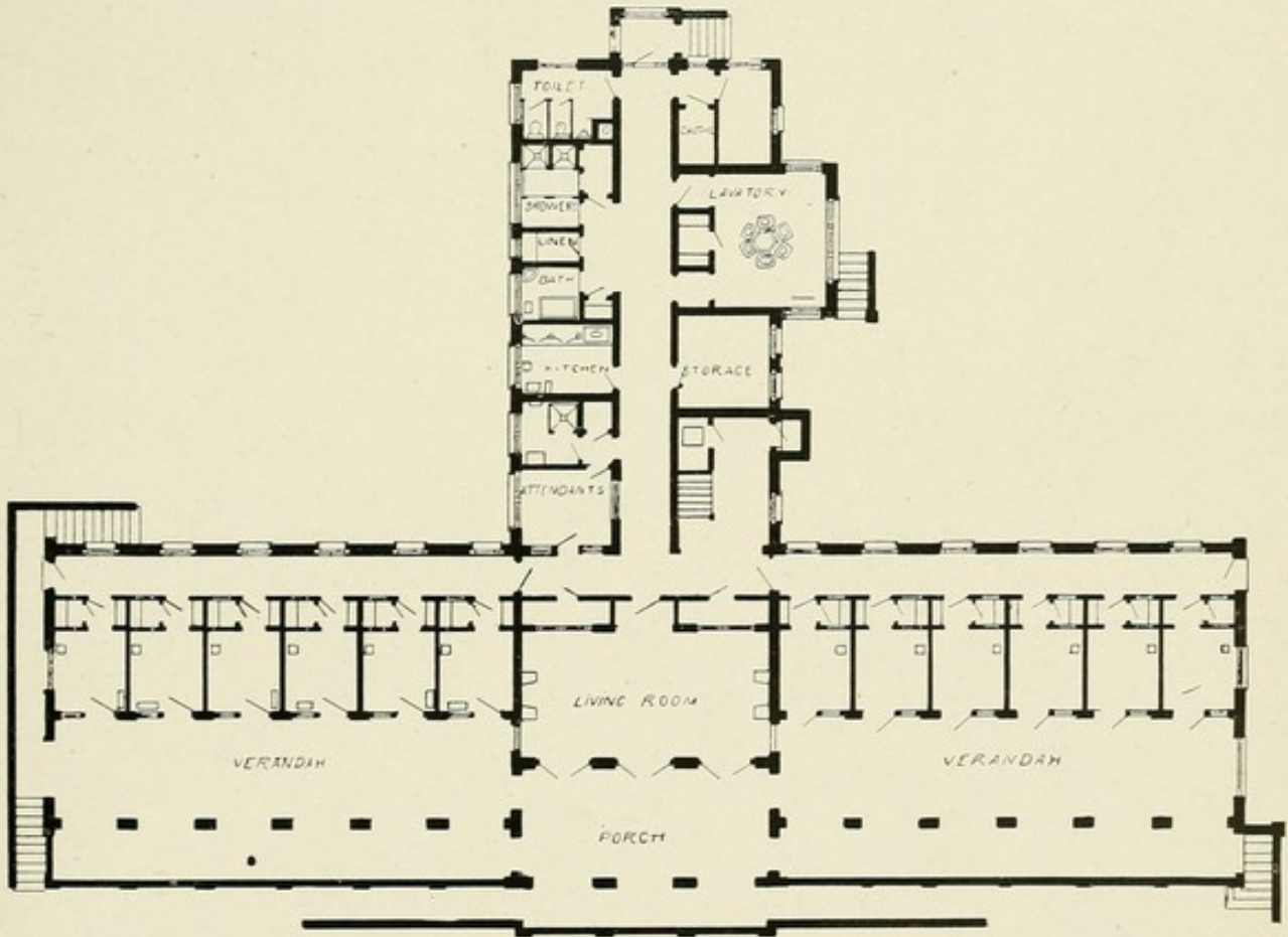
No. 67.—Ohio State Sanatorium, Mount Vernon, Ohio. F. L. PACKARD, ARCHITECT. RECEPTION HOSPITAL. VIEW OF FRONT ELEVATION AND FLOOR PLAN. CAPACITY, 24 PATIENTS. ESTIMATED COST, $30,000. (See illustration 77 for further description of this institution.)
