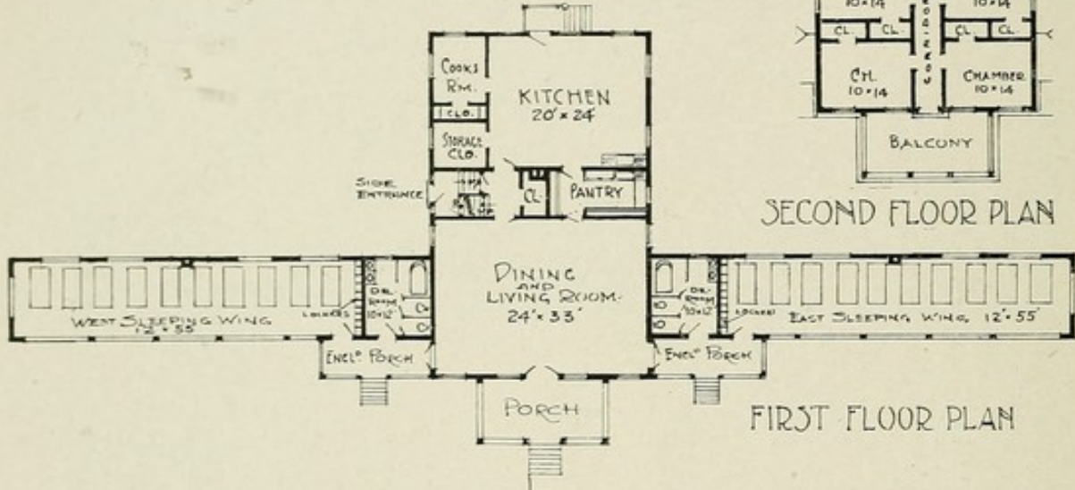
No. 41.—Cuenca Sanatorium, Bass Lake, Minn. ALFRED H. WHEELER, ARCHITECT. ELEVATION AND FLOOR PLANS. CAPACITY, 28 PATIENTS. COST, $9,000.
