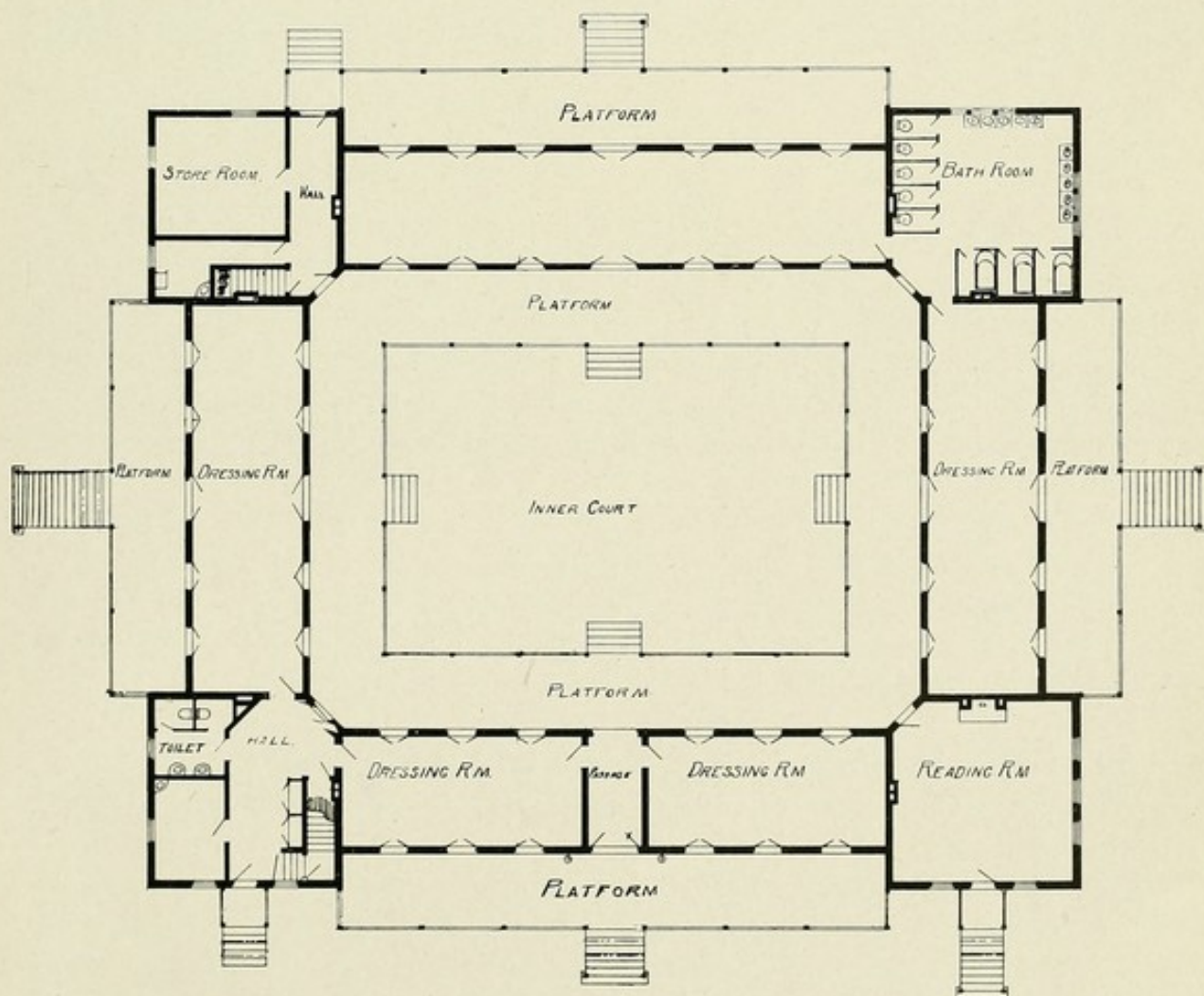
No. 54.—United States Army General Hospital, Fort Bayard, N. M. DESIGNED BY MAJOR GEORGE E. BUSHNELL. ENLISTED MEN'S WARD NO. 2. VIEW OF FRONT AND SIDE ELEVATION AND FLOOR PLAN. CAPACITY, 32 PATIENTS. ESTIMATED COST, $25,000.
