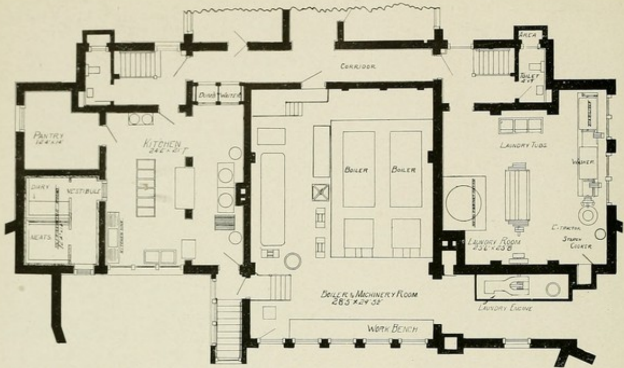
No. 20.—District Tuberculosis Hospital, Lima, Ohio. McLAUGHLIN & HULSKIN, ARCHITECTS. A PART OF THE BASEMENT FLOOR PLAN, SHOWING ARRANGEMENT OF LAUNDRY AND POWER PLANT, IN AN ADMINISTRATION BUILDING. (See illustration 43 for further description of this institution.)
