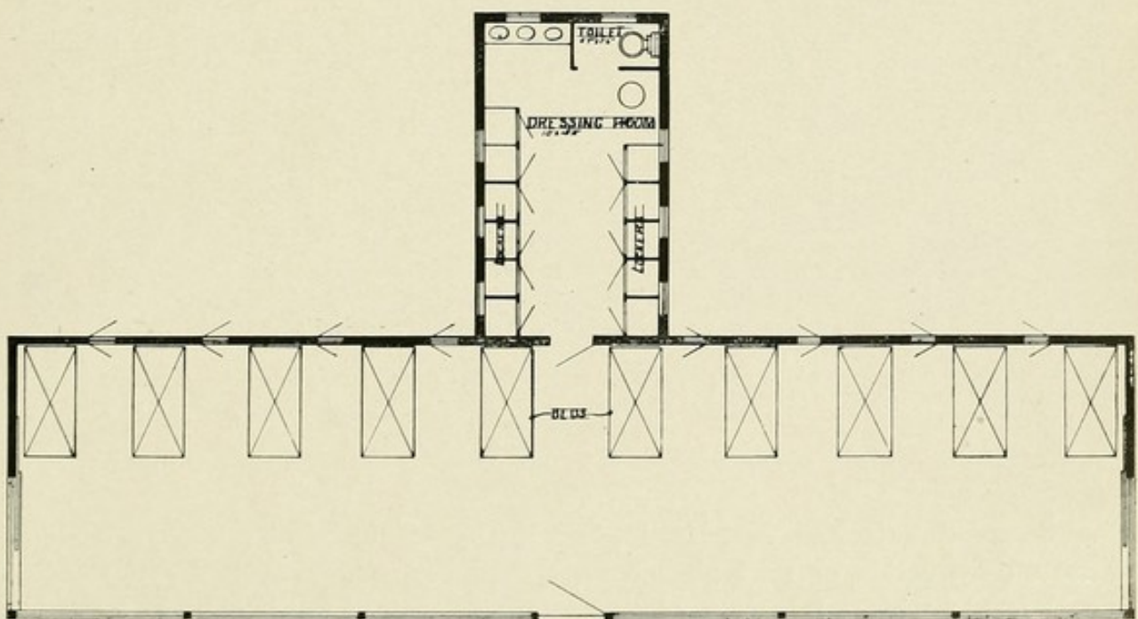
No. 82.—Edward Sanatorium, Naperville, Ill. W. A. OTIS AND EDWARD H. CLARK, ARCHITECTS. LEAN-TO. VIEW OF FRONT ELEVATION AND FLOOR PLAN. CAPACITY, 10 PATIENTS. ESTIMATED COST, $1,800. (See illustrations 62 and 88 for further description of this institution.)
