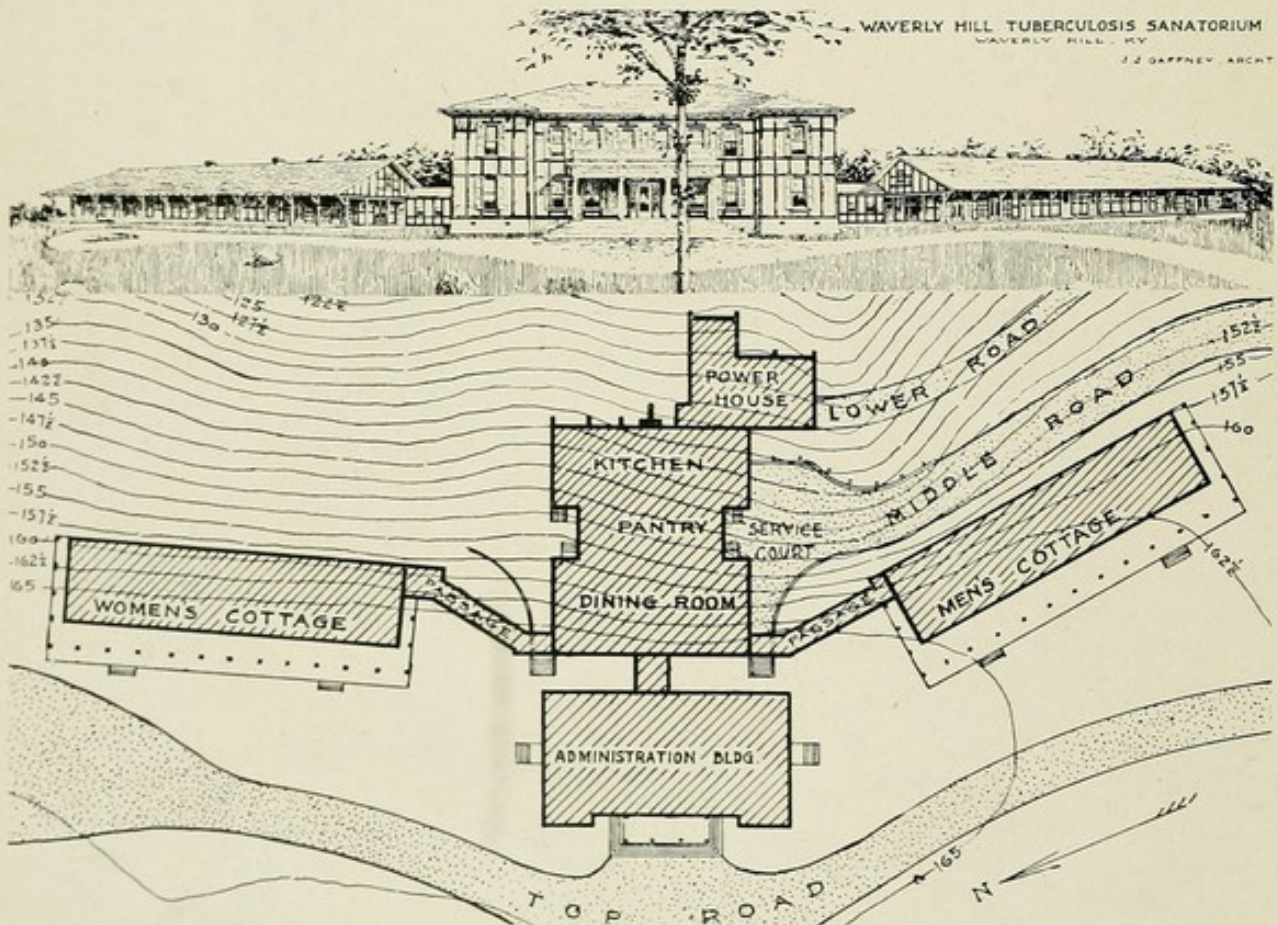
No. 5.—Waverly Hill Sanatorium, Waverly Hill, Ky. J. J. GAFFNEY, ARCHITECT. FRONT ELEVATION AND BLOCK PLAN SHOWING CONTOUR LINES AND METHOD OF GROUPING BUILDINGS ON THE EDGE OF A HILL WITH A STEEP SLOPE AT THE REAR. NOTE BACK VIEW OF PLANT, ILLUSTRATION NO. 18. CAPACITY, 40 PATIENTS. ESTIMATED COST, $100,000.
