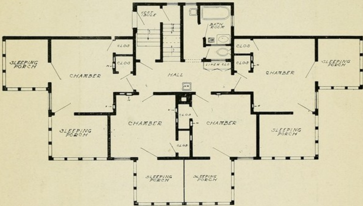
FIRST-FLOOR PLAN
