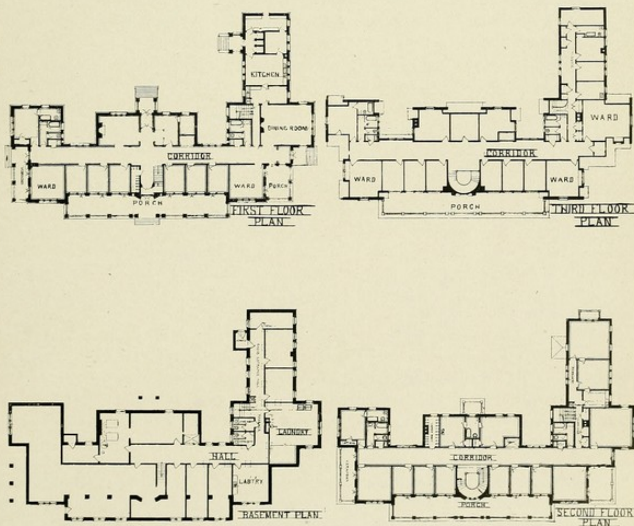
No. 37.—Lady Grey Hospital, Ottawa, Canada. WEEKS & KEEFER, ARCHITECTS. VIEW OF FRONT ELEVATION AND FLOOR PLANS. CAPACITY, 45 PATIENTS. COST, $60,000.
