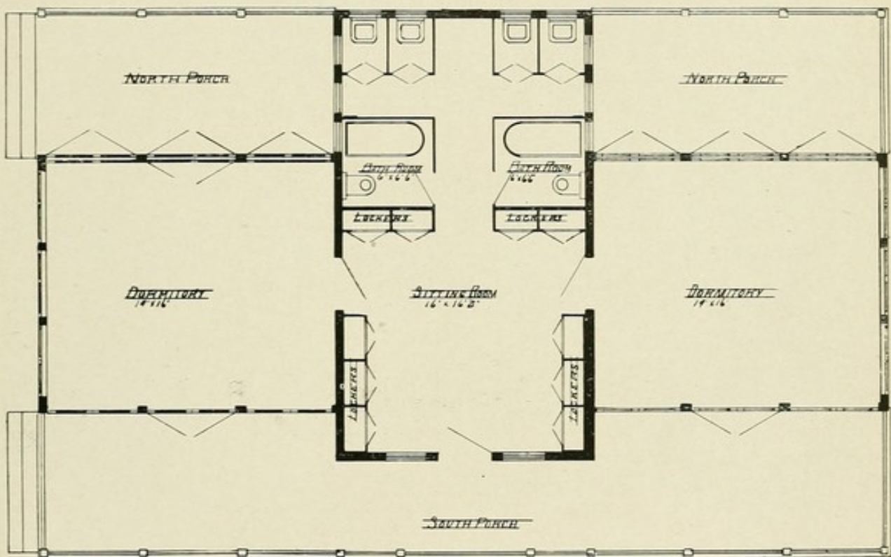
No. 86.—Association Sanatorium, Louisville, Ky. D. X. MURPHY & BROTHER, ARCHITECTS. LEAN-TO. VIEW OF FRONT ELEVATION AND FLOOR PLAN. CAPACITY, 12 PATIENTS. ESTIMATED COST, $2,750. (See illustration 99 for further description of this institution.)
