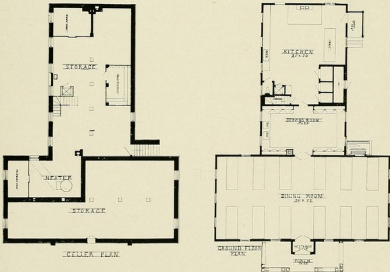
No. 31.—New Haven County State Tuberculosis Sanatorium, Meriden, Conn. FOOTE & TOWNSEND, ARCHITECTS. SERVICE BUILDING. VIEW OF FRONT ELEVATION AND FLOOR PLANS. SERVICE CAPACITY, 122 PATIENTS. ESTIMATED COST, $15,000. (See illustration 79 for further description of this institution.)
