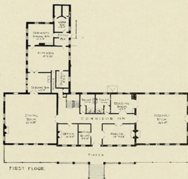
No. 23.—Maine State Sanatorium, Hebron, Me. T. C. STEVENS & J. H. STEVENS, ARCHITECTS. ADMINISTRATION BUILDING. VIEW OF FRONT ELEVATION AND FLOOR PLANS. ADMINISTRATIVE CAPACITY, 100 PATIENTS. ESTIMATED COST, $50,000. (See illustrations 11 and 58 for further description of this institution.)
