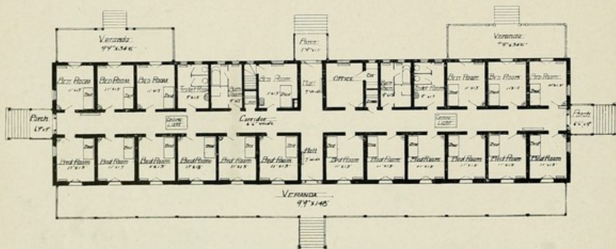
No. 53.—United States Army General Hospital, Fort Bayard, N. M. OFFICERS' QUARTERS. VIEW OF FRONT AND SIDE ELEVATION AND FLOOR PLAN. CAPACITY, 18 PATIENTS. COST, $18,534.
