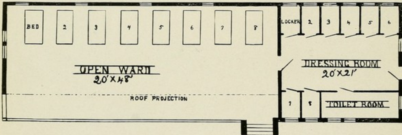
No. 91.—Loomis Sanatorium, Liberty, N. Y. DESIGNED BY DR. HERBERT MAXON KING. LEAN-TO. VIEW OF FRONT ELEVATION AND FLOOR PLAN. CAPACITY, 8 PATIENTS. ESTIMATED COST, $1,000. (See illustrations 1, 72, 73 and 108 for further description of this institution.)
