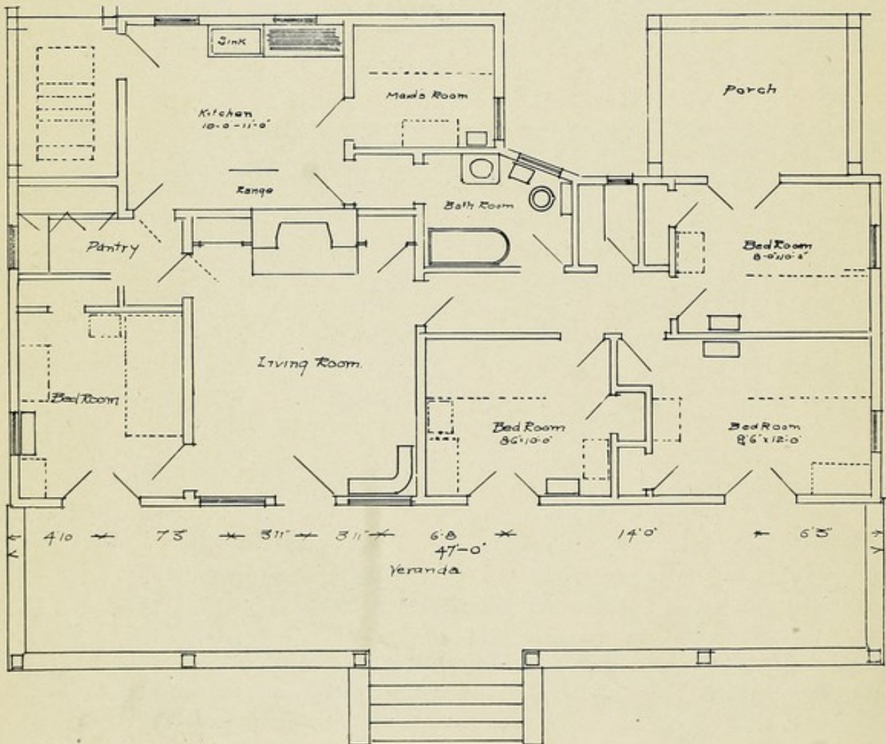
No. 108.—Loomis Sanatorium, Liberty, N. Y. SCOPES & FEUSTMANN, ARCHITECTS. ORCHARD COTTAGE. VIEW OF FRONT AND SIDE ELEVATIONS AND FLOOR PLAN. CAPACITY, 4 PATIENTS. ESTIMATED COST, $3,200. (See illustrations 1, 72, 73 and 91 for further description of this institution.)
