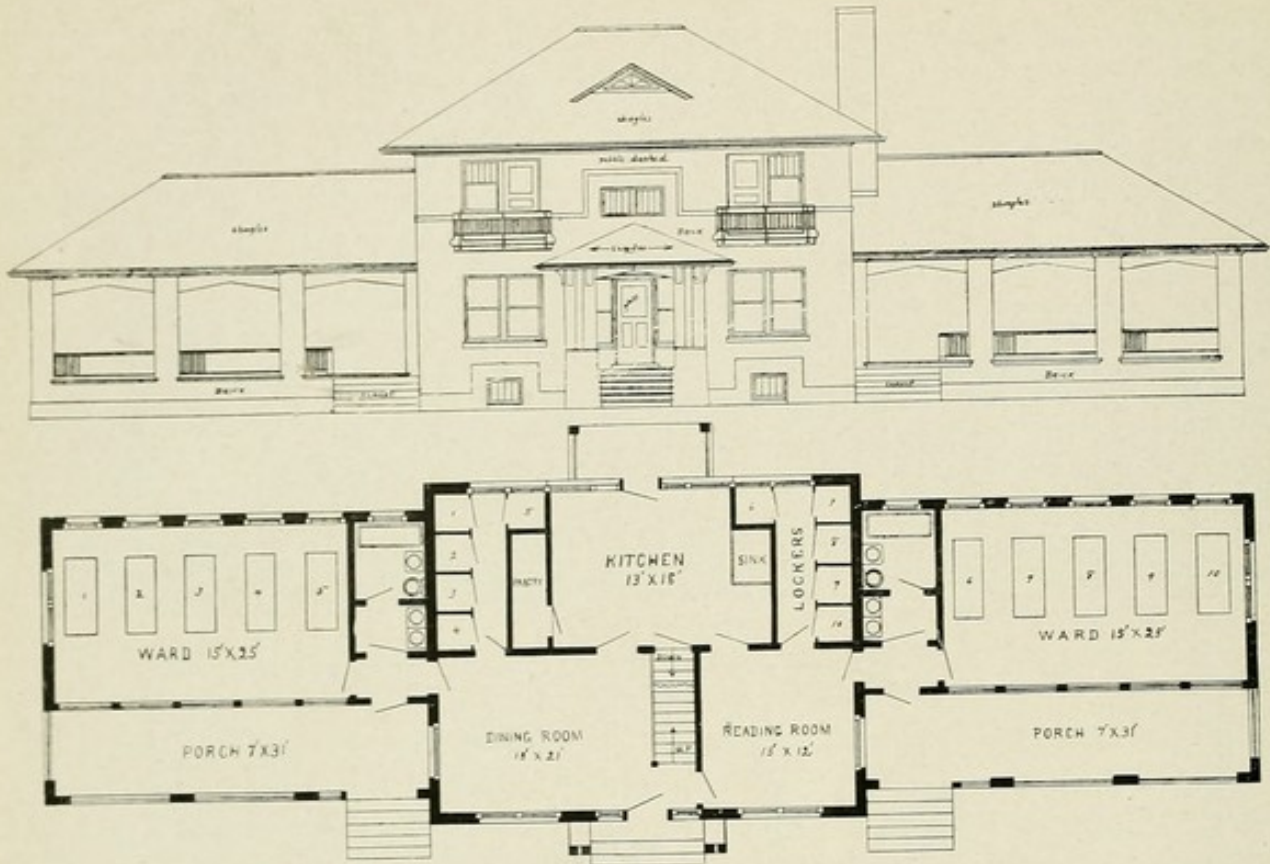
No. 44.—A Design for a Small Village or Town Hospital or Sanatorium. FRONT ELEVATION AND FLOOR PLAN. CAPACITY, 14 PATIENTS. ESTIMATED COST, $15,000.
