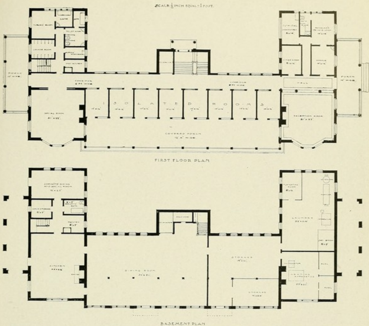
No. 50.—Jewish Hospital for Consumptives, Reisterstown, Md. PAVILION FOR ADVANCED CASES. FLOOR PLANS. CAPACITY, 24 PATIENTS. COST, $30,000.
