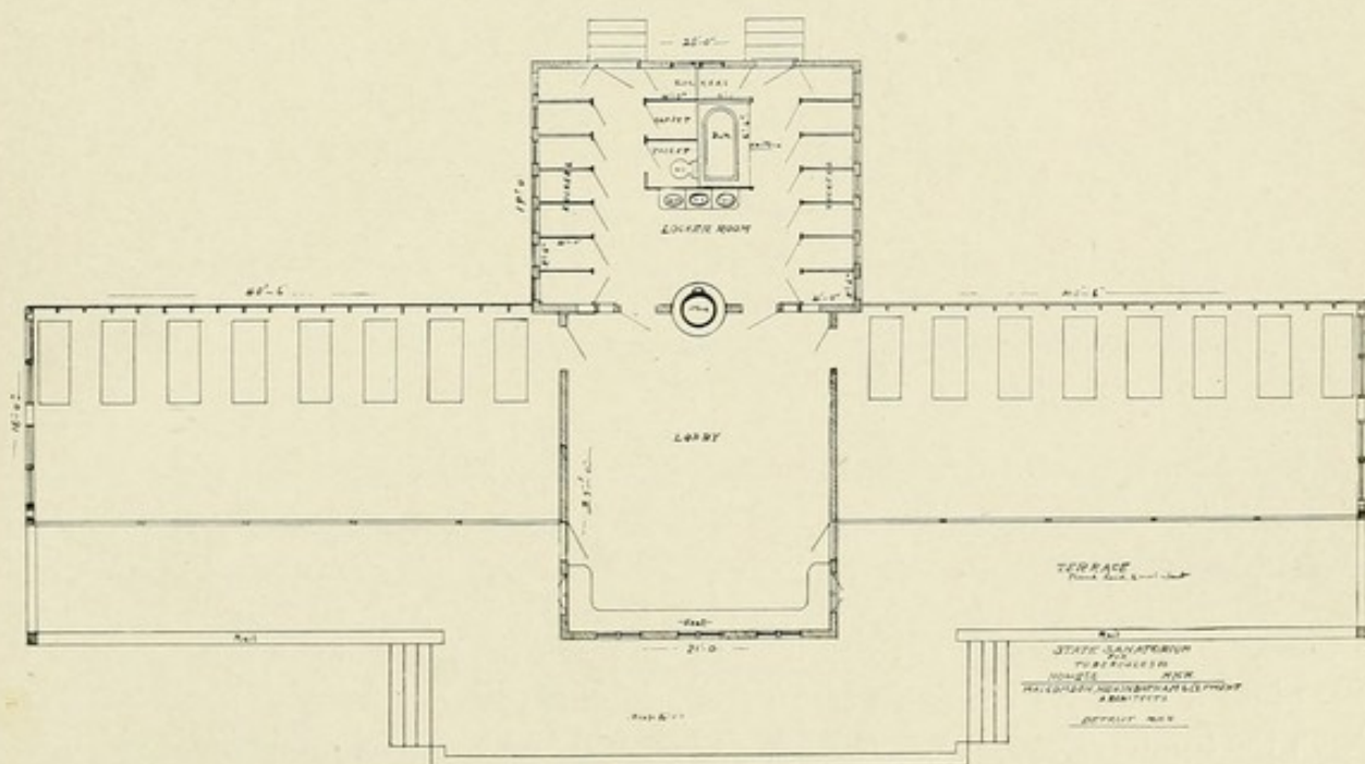
No. 74.—Michigan State Sanatorium, Howell, Mich. MALCOMSON, HIGINBOTHAM AND CLEMENT, ARCHITECTS. LEAN-TO. VIEW OF FRONT ELEVATION AND FLOOR PLAN. CAPACITY, 16 PATIENTS. COST, $4,500.
