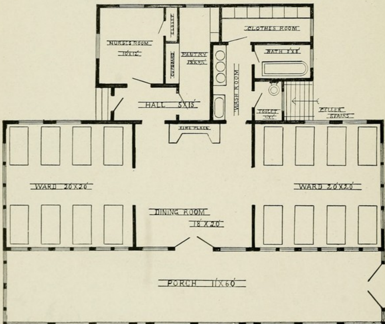
No. 66.—Danvers State Hospital, Hawthorne, Mass. DESIGNED BY DR. F. PAGE. PAVILION; VIEW OF FRONT AND SIDE ELEVATION AND FLOOR PLAN. CAPACITY, 16 PATIENTS. ESTIMATED COST, $6,000.
