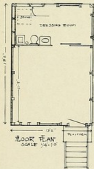
No. 96.—Millet Sanatorium, East Bridgewater, Mass. DESIGN BY DR. C. S. MILLET. COTTAGE. VIEW OF FRONT ELEVATION, FLOOR PLAN, SIDE AND END ELEVATION. CAPACITY, 1 PATIENT. ESTIMATED COST, $200.
