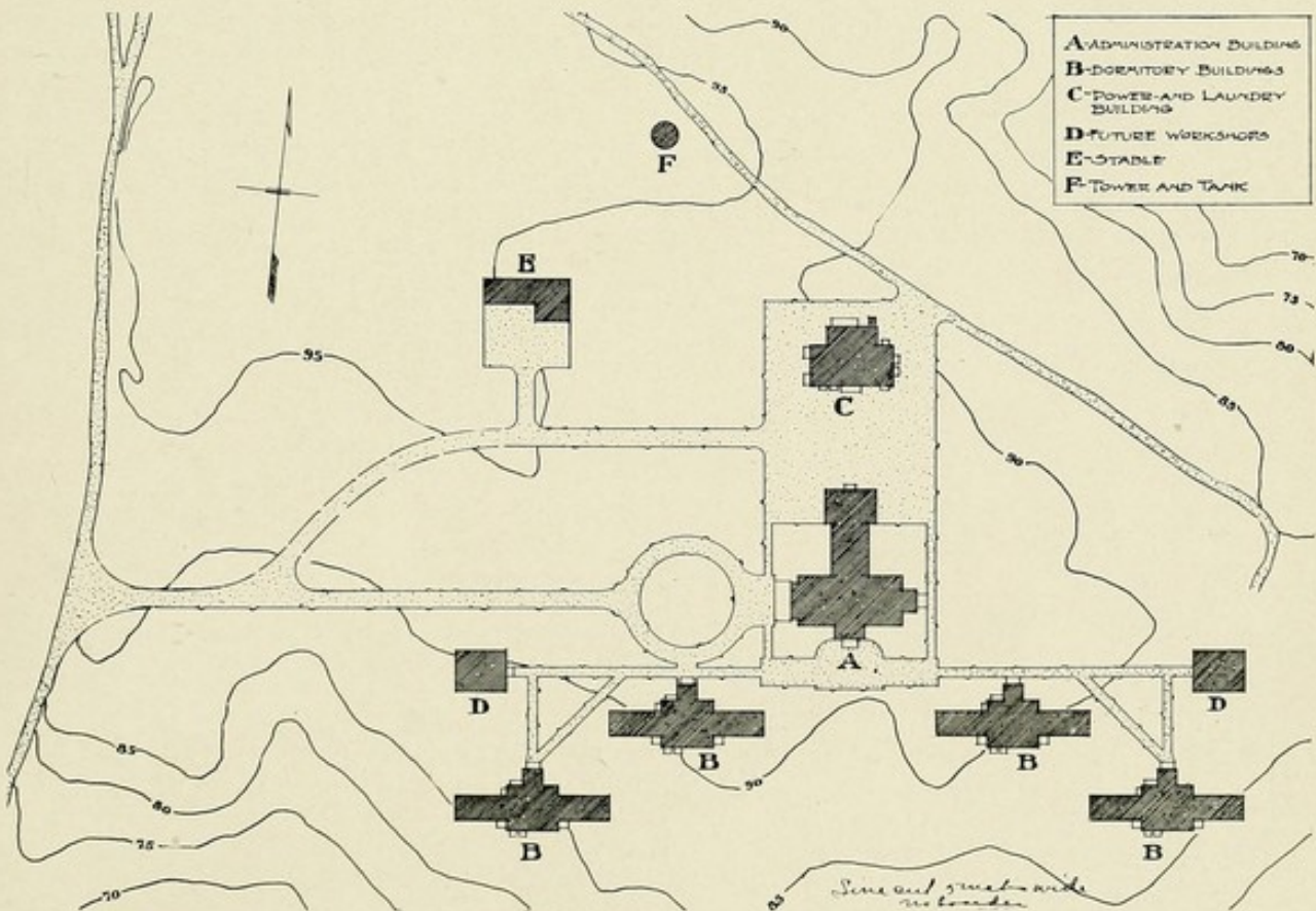
No. 12.—Preventorium for Children, Farmingdale, N. J. SCOPES & FEUSTMANN, AND WALTER W. JUDELL, ASSOCIATED ARCHITECTS. BIRD'S-EYE VIEW AND BLOCK PLAN SHOWING METHOD OF GROUPING THE BUILDINGS. (See illustrations 19, 27 and 95 for further description of this institution.)
