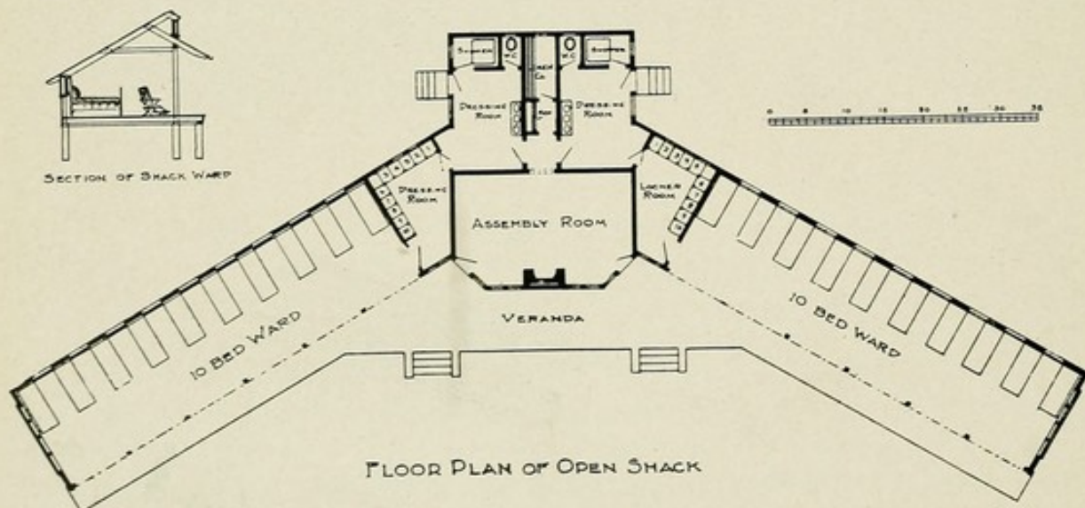
No. 87.—North Reading State Sanatorium, North Reading, Mass. JOHN A. FOX, ARCHITECT. LEAN-TO. VIEW OF FRONT ELEVATION, FLOOR PLAN AND CROSS-SECTION. CAPACITY, 20 PATIENTS. COST, $3,500.
