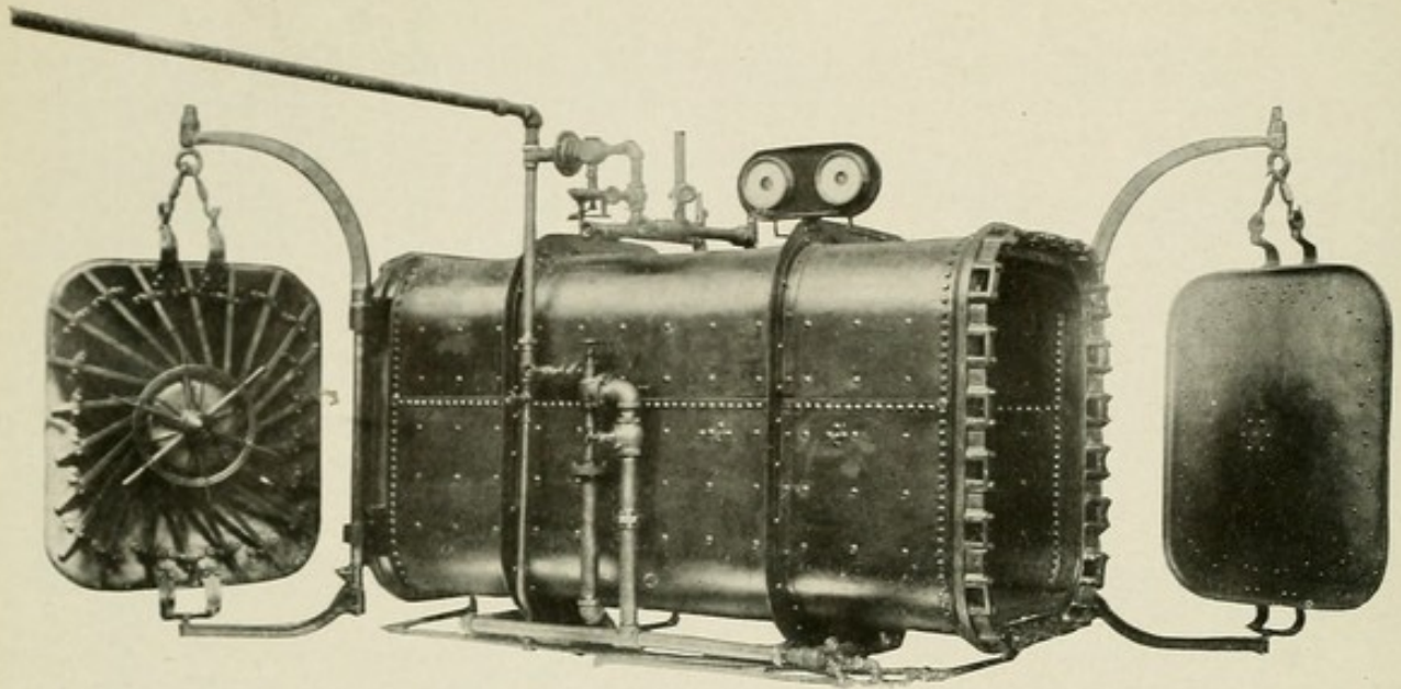
No. 21.—A Rectangular Steam Disinfecting Chamber, for Use in Connection with the Laundry. A CONVENIENT SHAPE FOR TUBERCULOSIS HOSPITAL AND SANATORIUM WORK. LOANED BY THE KNY-SHEERER COMPANY.
