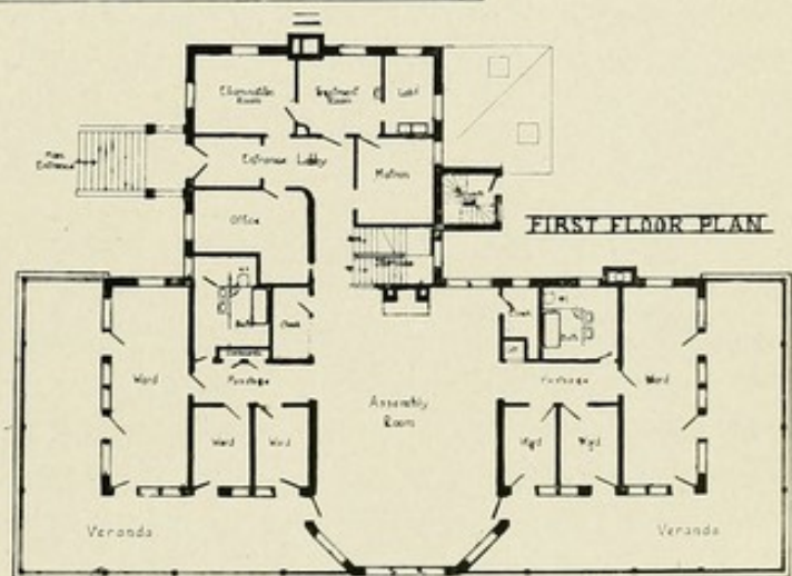
No. 25.—Manitoba Sanatorium, Ninette, Manitoba, Canada. DESIGNED BY DR. D. A. STEWART. ADMINISTRATION BUILDING. VIEW OF FRONT ELEVATION AND FLOOR PLANS. ADMINISTRATIVE CAPACITY, 100 PATIENTS. COST, $33,000. (See illustration 81 for further description of this institution.)
