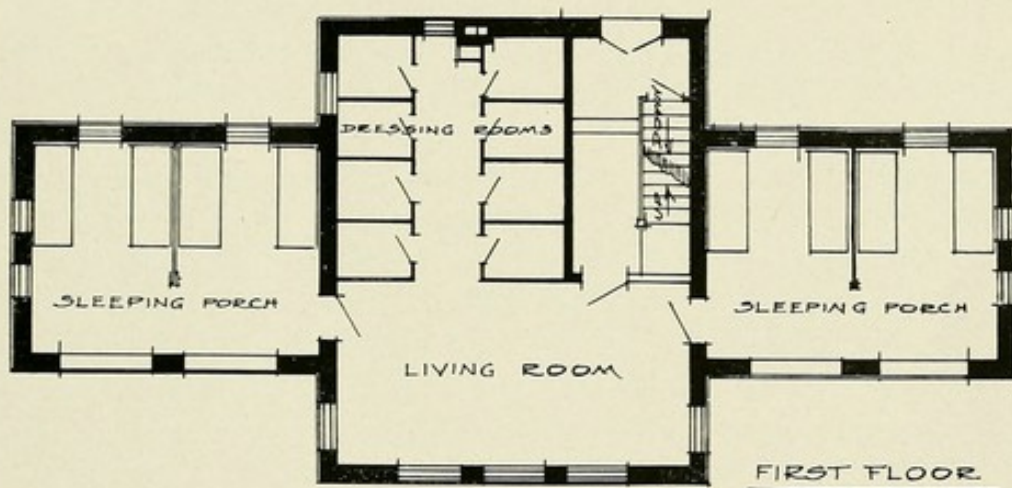
No. 14.—Municipal Sanatorium, Otisville, N. Y. DESIGNED BY DR. HERMANN M. BIGGS. JAMES D. BURT, ARCHITECT. SERVANTS' BUILDING No. 107. THIS STRUCTURE IS AN EXAMPLE OF A LEAN-TO CONSTRUCTED WITH FIRE-PROOF MATERIAL, DESIGNED TO SUPPLY OPEN-AIR SLEEPING QUARTERS FOR SERVANTS WHO WISH TO REMAIN AND SUPPORT THEMSELVES AT THE INSTITUTION AFTER COMPLETING THE TREATMENT. CAPACITY, 16 PERSONS; COST, $5,000.
