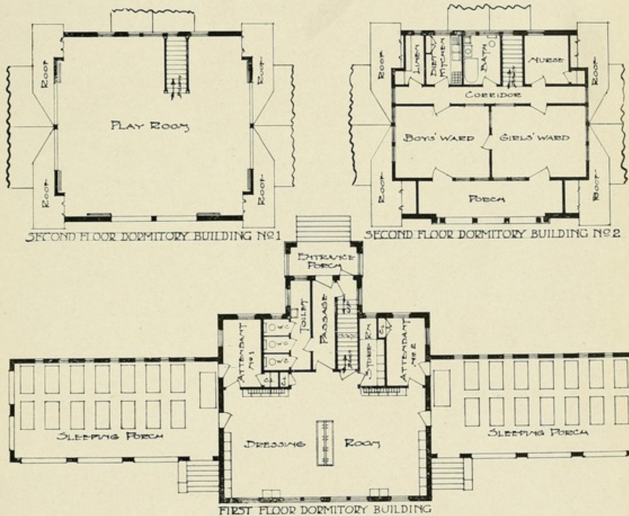
No. 95. —Preventorium for Children, Farmingdale, N. J. DESIGNED BY DR. HERMANN M. BIGGS, SCOPES & FEUSTMANN, AND WALTER W. JUDELL, ASSOCIATED ARCHITECTS. LEAN-TO. FRONT ELEVATION AND FLOOR PLANS. CAPACITY, 28 CHILDREN AND TWO ATTENDANTS. ESTIMATED COST, $7,700. (See illustrations 12, 19 and 27 for further description of this institution.)
