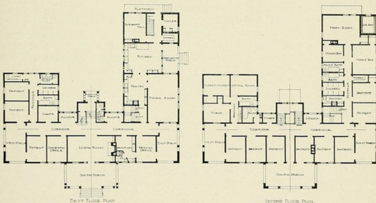
No. 38.—Lake Edward Sanatorium, Lake Edward, Province of Quebec, Canada. SCOPES & FEUSTMANN, ARCHITECTS. VIEW OF FRONT AND SIDE ELEVATION, FLOOR PLANS. CAPACITY, 26 PATIENTS. COST, $26,000.
