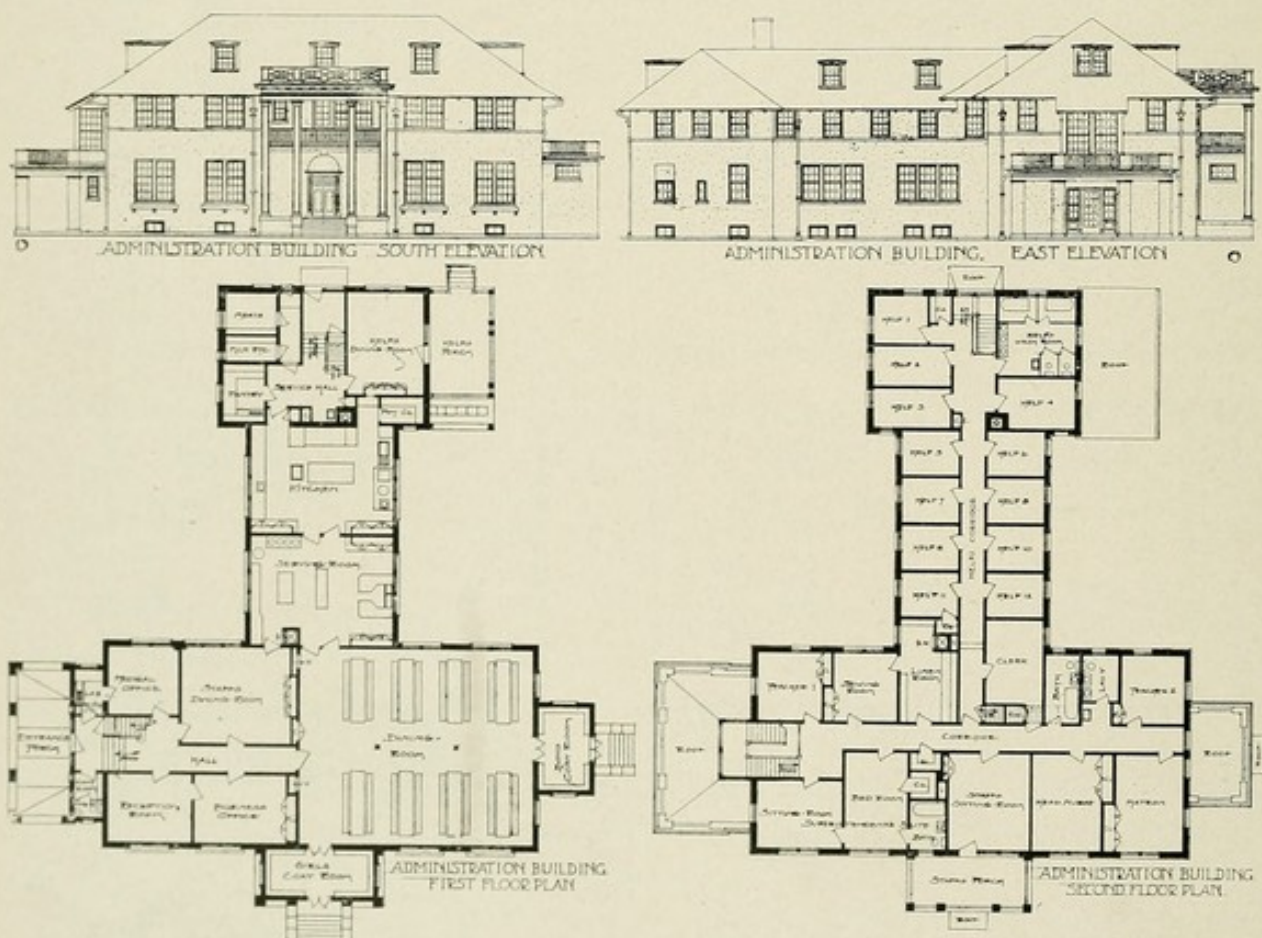
No. 27.—Preventorium for Children, Farmingdale, N. J. SCOPES & FEUSTMANN, AND WALTER W. JUDELL, ASSOCIATED ARCHITECTS. ADMINISTRATION BUILDING. FRONT AND SIDE ELEVATIONS AND FLOOR PLANS. ADMINISTRATION CAPACITY, 112 PATIENTS. COST, $35,000. (See illustrations 12, 19 and 95 for further description of this institution.)
