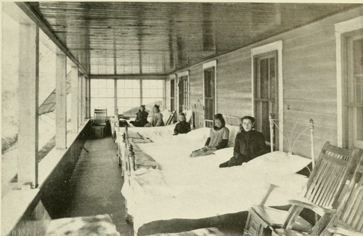
No. 72.—Loomis Sanatorium, Liberty, N. Y. VIEW OF CHAPMAN COTTAGE. SLEEPING PORCH; ILLUSTRATING METHOD OF CONSTRUCTION AND INTERIOR FINISH, USING NARROW FLOOR BOARDS FOR SEALING. (See illustrations 1, 73, 91 and 108 for further descriptions of this institution.)
