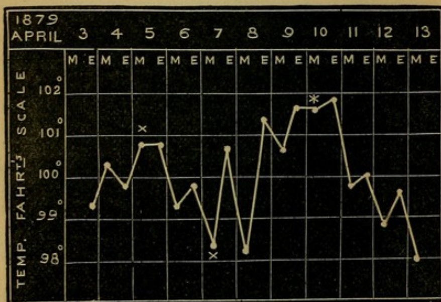
Thermometric Chart.
