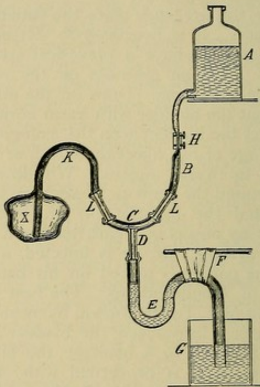
FIG. 292.—Keen's siphonage apparatus: X , cavity to be drained; A , reservoir; K , tube from cavity; B , tube from reservoir; H , clamp on tube from reservoir; L, L, D , glass tubes; C , rubber tube connecting cavity-drain with reservoir-drain; E , S-shaped rubber tube maintained in shape by hooking up at F ; G , vessel containing antiseptic fluid.
