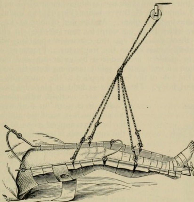
FIG. 91.—Hodgen's suspending apparatus.
