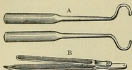
FIG. 242.—A, hernia-needles; B, hinged hernia-director.
