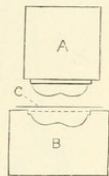
A, Fusible-metal die. B, Counter-die. C, Plate to form the cap.
