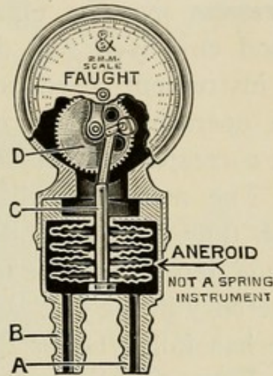
FIG. 17.—Diagram of internal mechanism, showing compression chambers.
