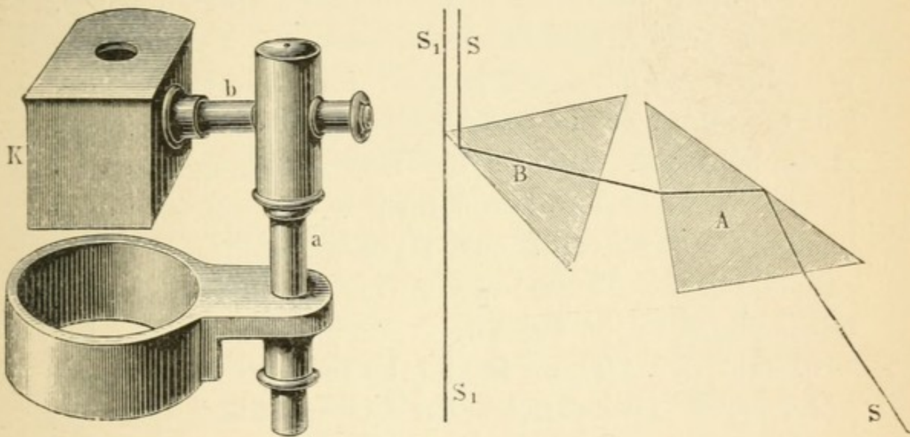
FIG. 23.—Zeiss's camera lucida.
