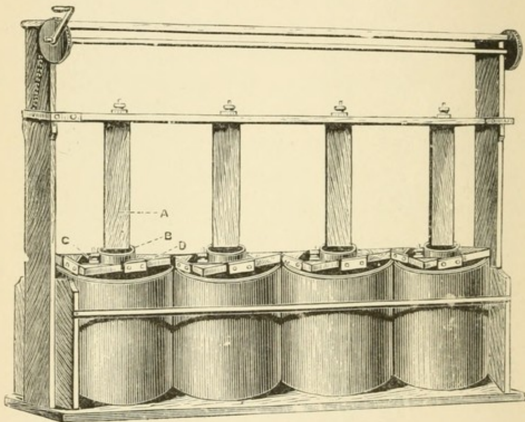
FIG. 25.—Improved constant battery.
