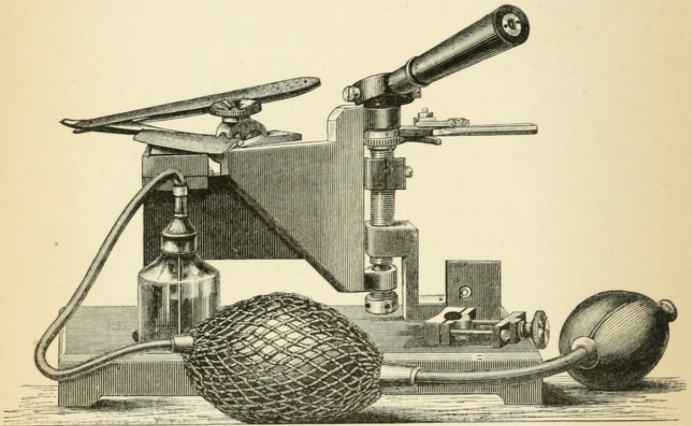
FIG. 43.—Roy's improved microtome.
