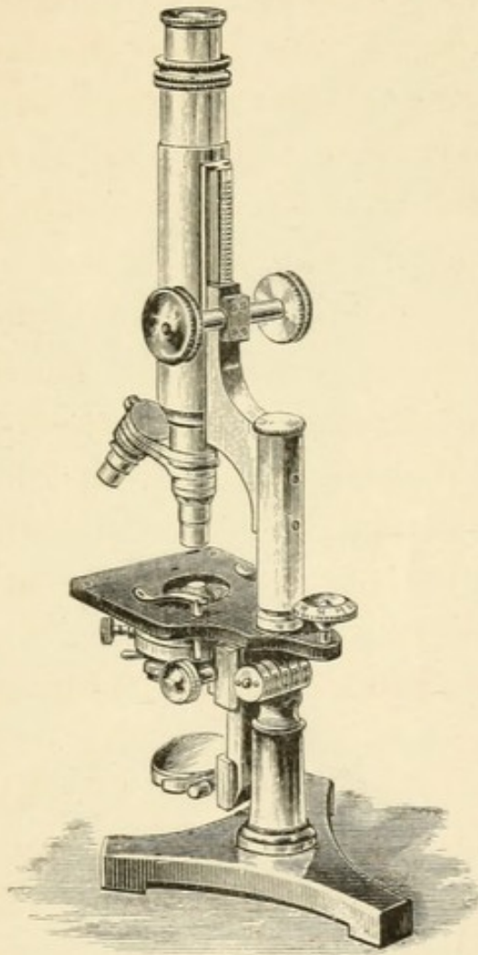
FIG. 20.—Beck's pathological stand.
