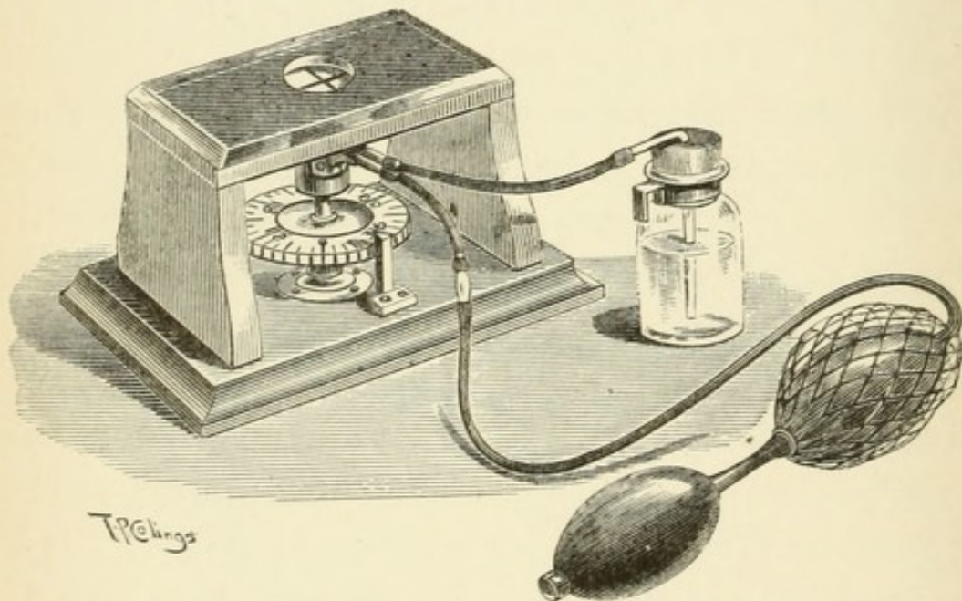
FIG. 42.—Author's pattern of Zeiss's microtome.
