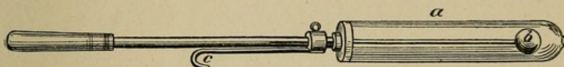
FIG. 68.—Internal Administration of Sparks. b , electrode; a , insulating tube, perforated for passage of spark and current.
