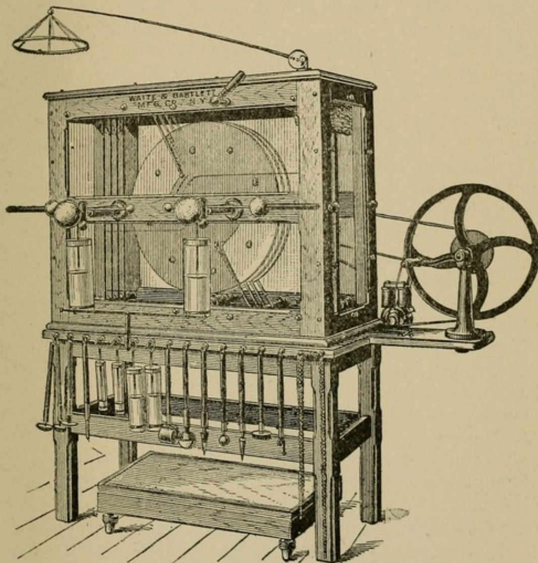
FIG. 61.—Static Machine.
