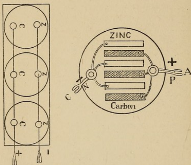
FIG. 3.—Quantity Currents.
