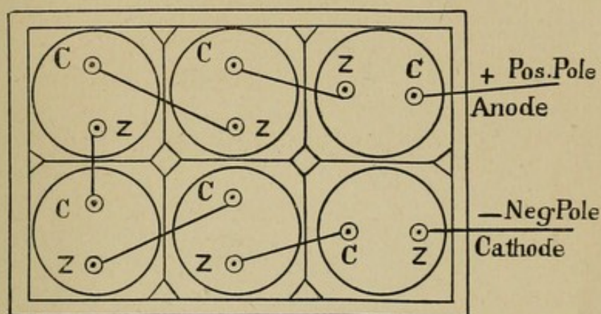
FIG. 4.—Arrangement for Intensity.
