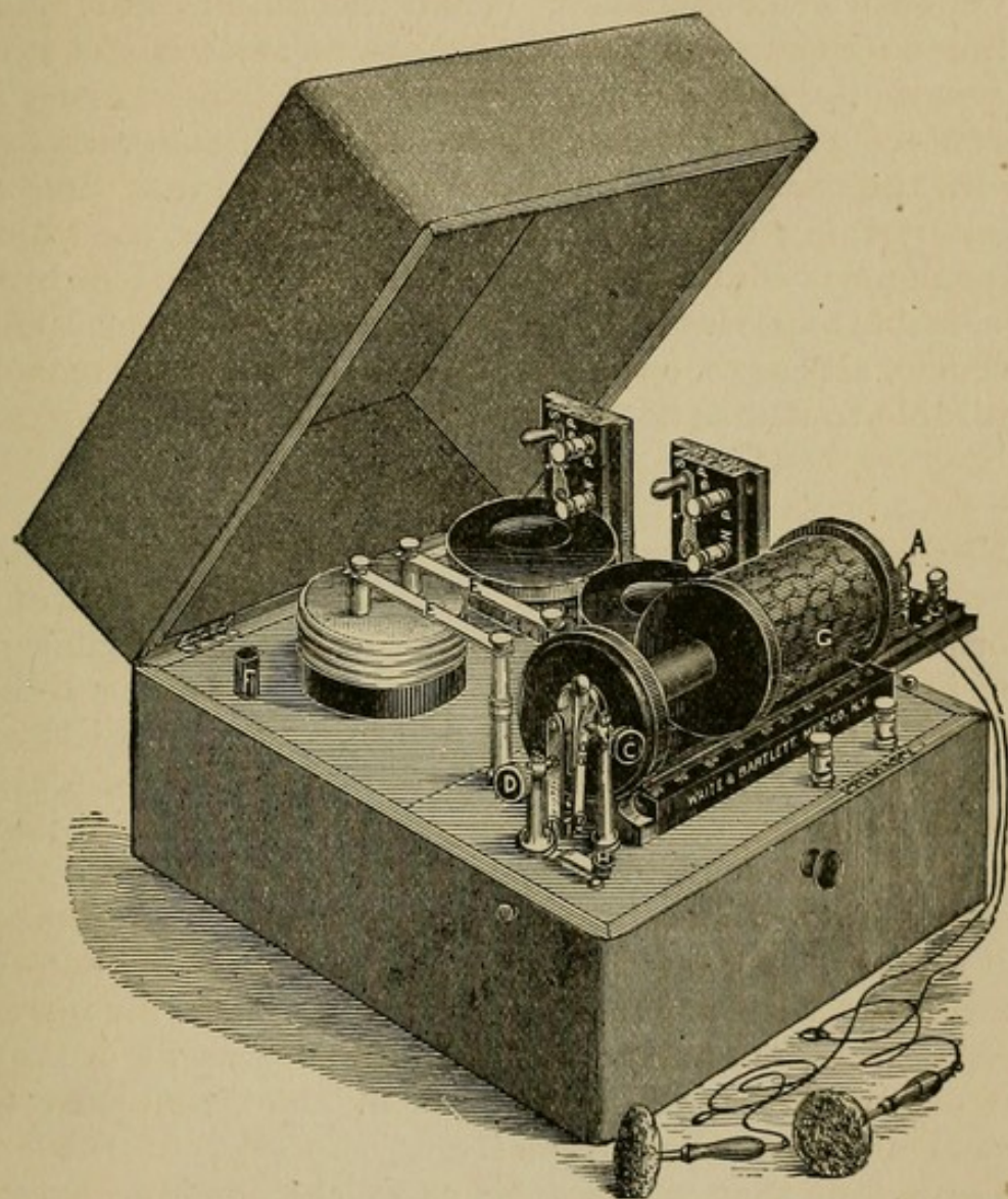
FIG. 16.—Engelmann Faradic Battery.
