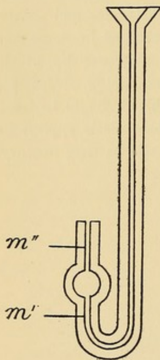
FIG. 13.—VISCOSIMETER OF DENNING AND WATSON.
