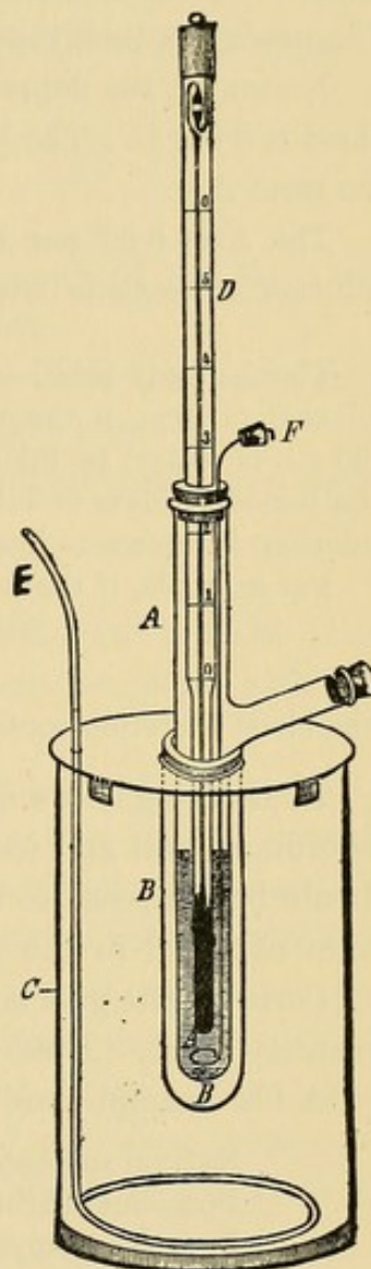
FIG. 14.—BECKMANN'S CRYOSCOPE.
