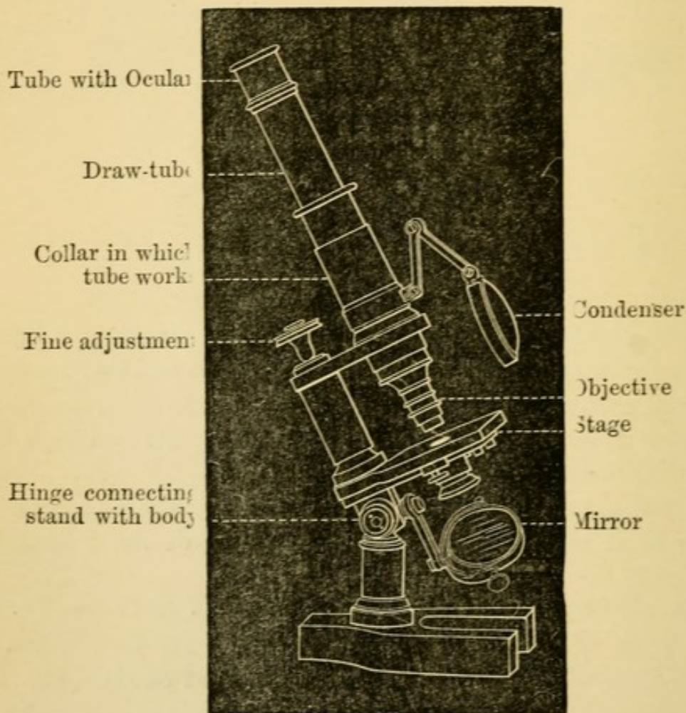
Fig. 1.—Continental Model Microscope.
