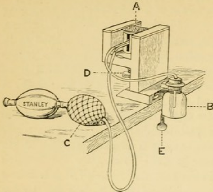
Fig. 14.—Cathcart's Microtome.
