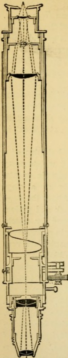
Fig. 3.—Diagram of the Method in which a Compound Microscope magnifies.
