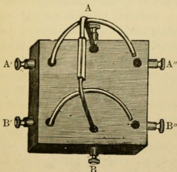
Fig. 34. Reverser. Brass wires (not shown in fig.) connect mercury cups corresponding to A' and B'', and A'' and B'.
