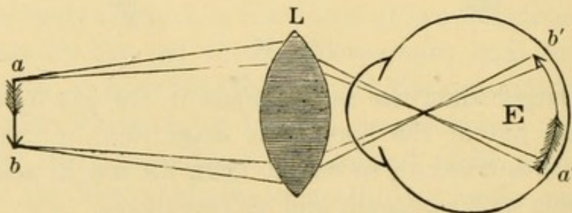
FIG. 77. — SIMPLE MICROSCOPE
