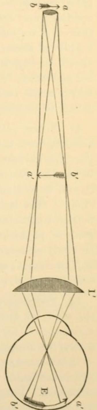
FIG. 78. — COMPOUND MICROSCOPE
