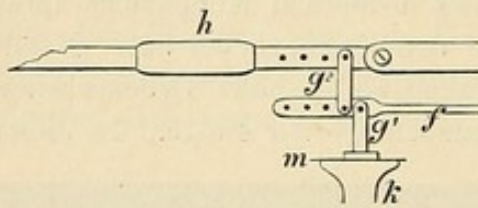
Fig. 179. Hürthle's Federmanometer.
