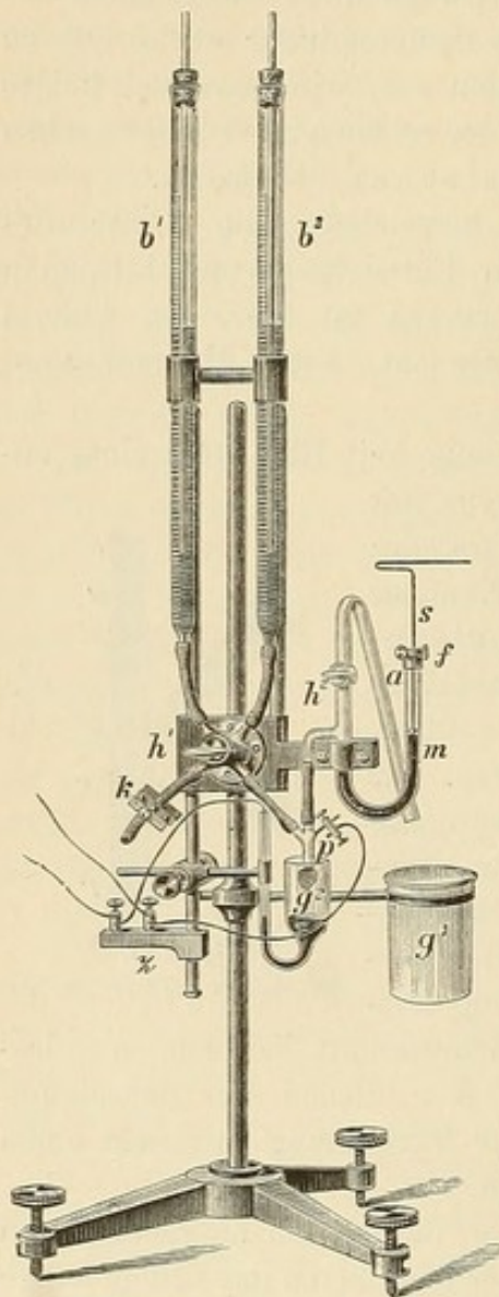
Fig. 141. Kronecker's Froschherzmanometer. ( \frac{1}{5} nat. Gr.).
