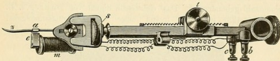
Fig 110. Marey's Chronograph. ( \frac{2}{3} nat. Gr.)
