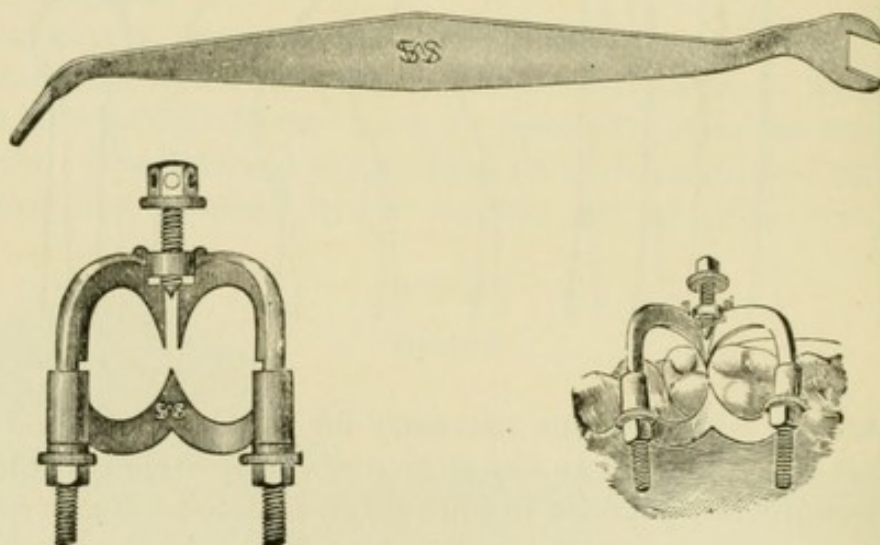
Parr's universal separator.
