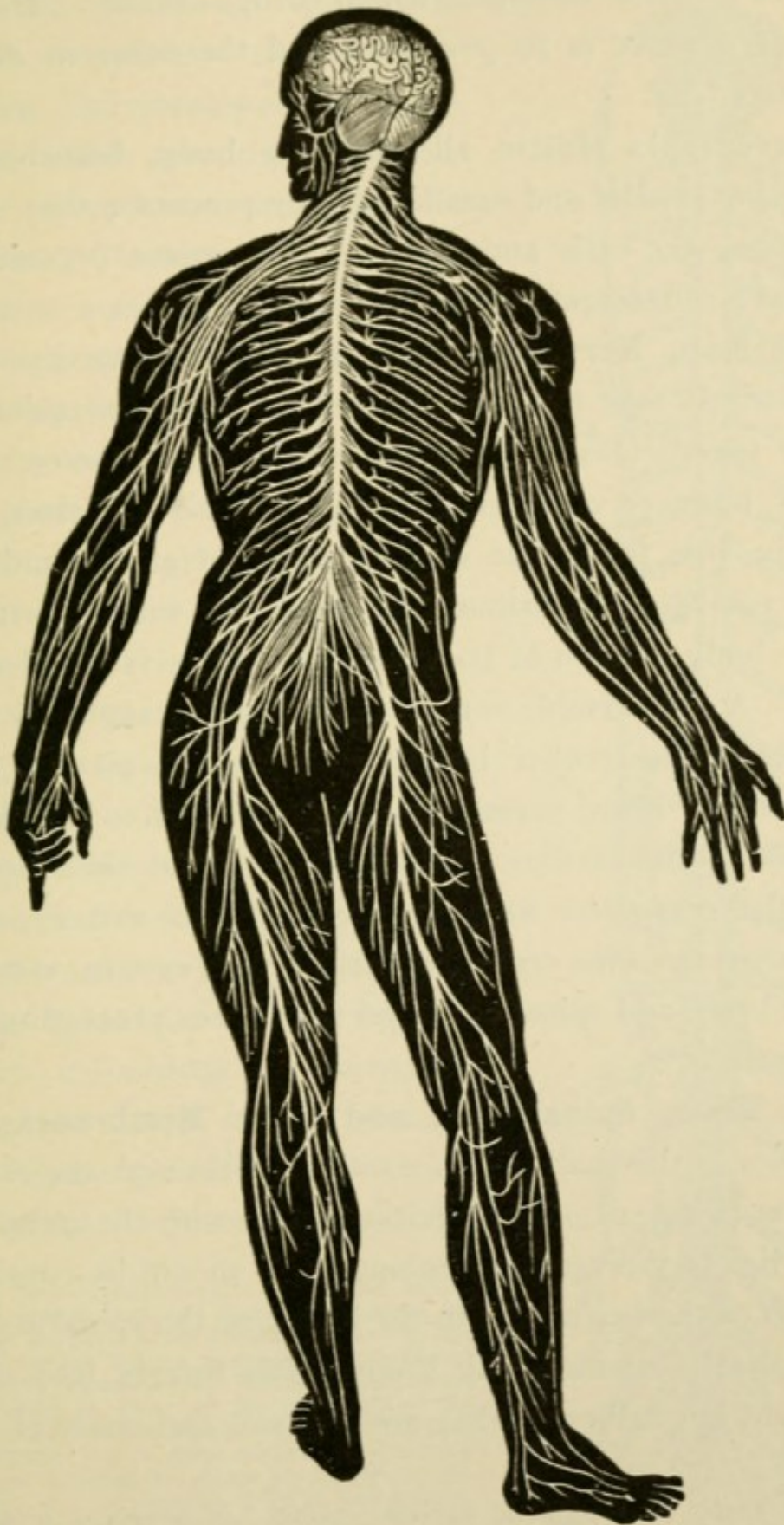
FIG. 112.—Diagram illustrating the general arrangement of the nervous system.
