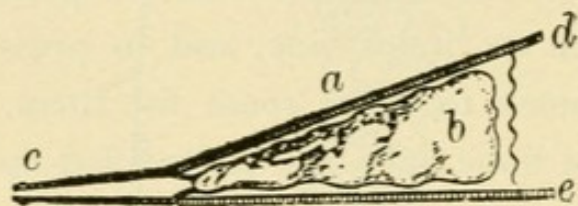
FIG. 100.—Diagram to illustrate the entry of air to the lungs when the thoracic cavity enlarges,
