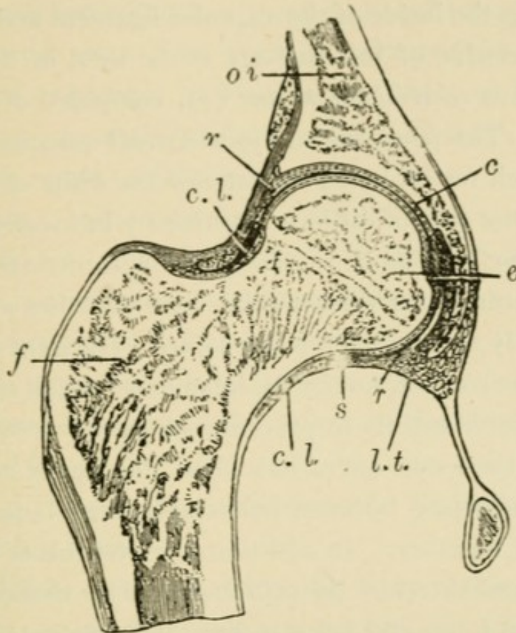
FIG. 26.—Section through the hip joint.
