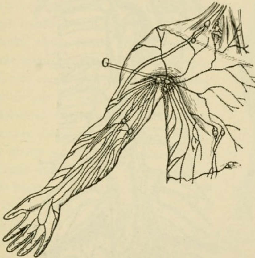
FIG. 71.—Superficial lymphatics and glands. G. Axillary glands.
