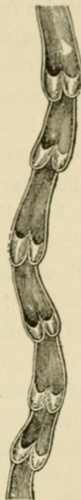
FIG. 73.—Valves of lymphatics. (Sap- pey.)
