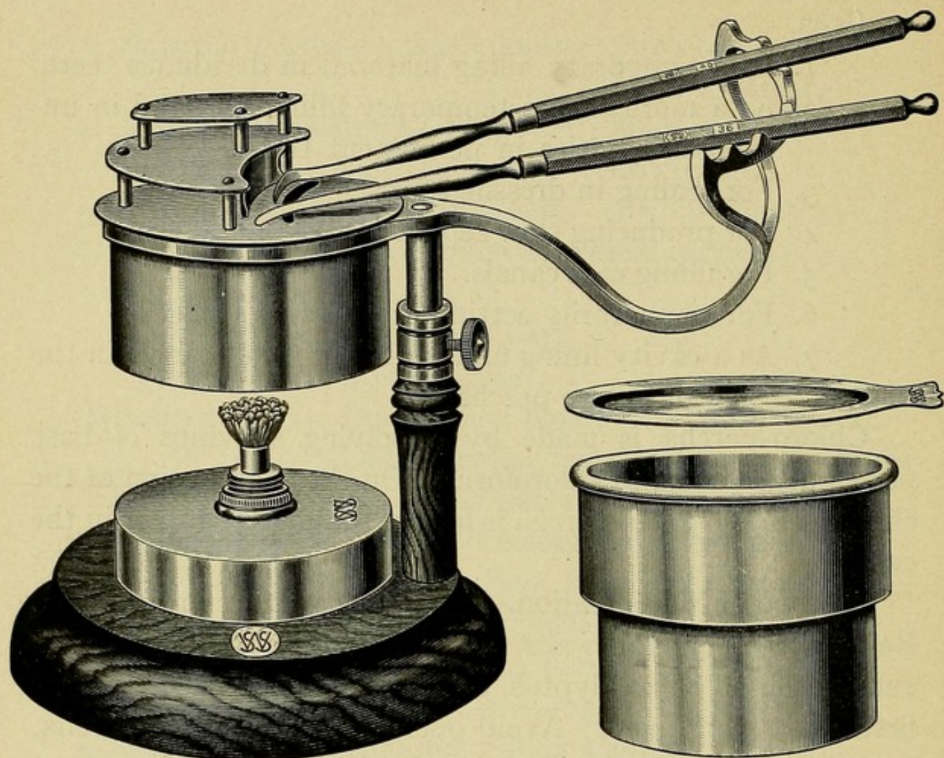
FIG. 172.—Flagg's gutta-percha and tool heater.
