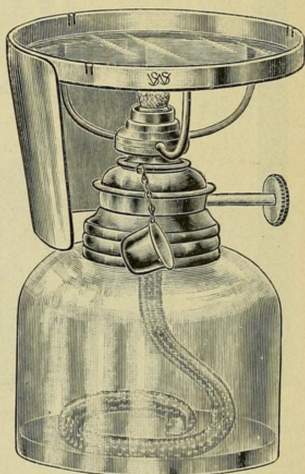
FIG. 121.—Alcohol lamp, flame shield and gold annealer.
