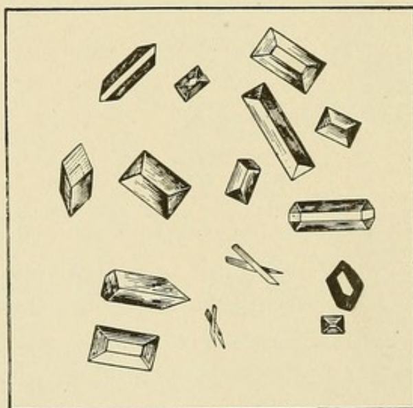
Ammonium phosphates.
