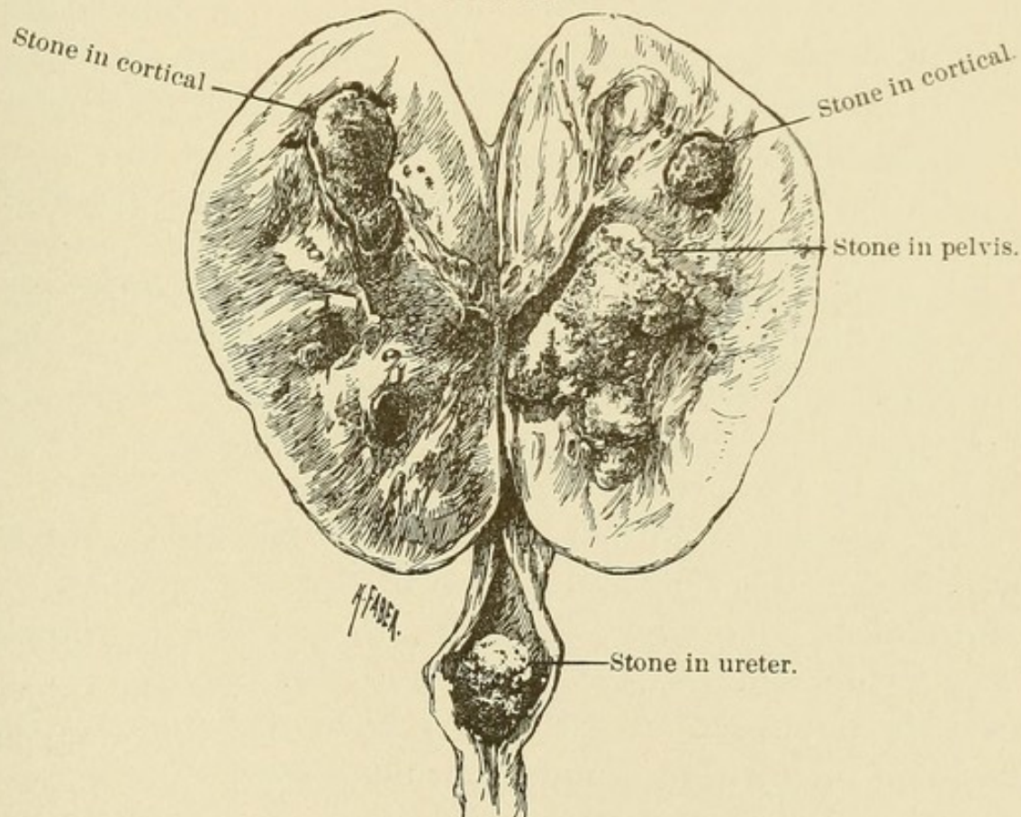
Nephro-lithiasis.
