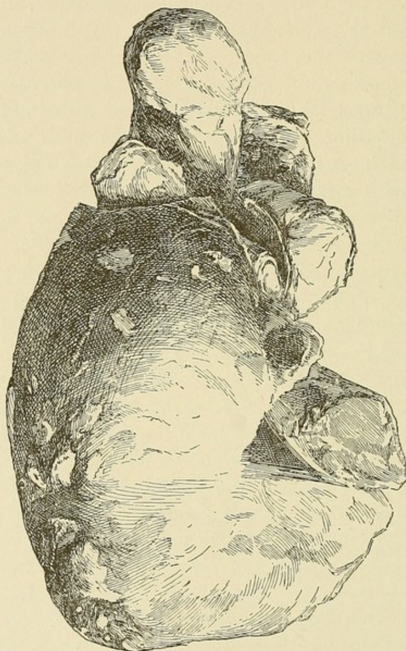
Renal calculus.
