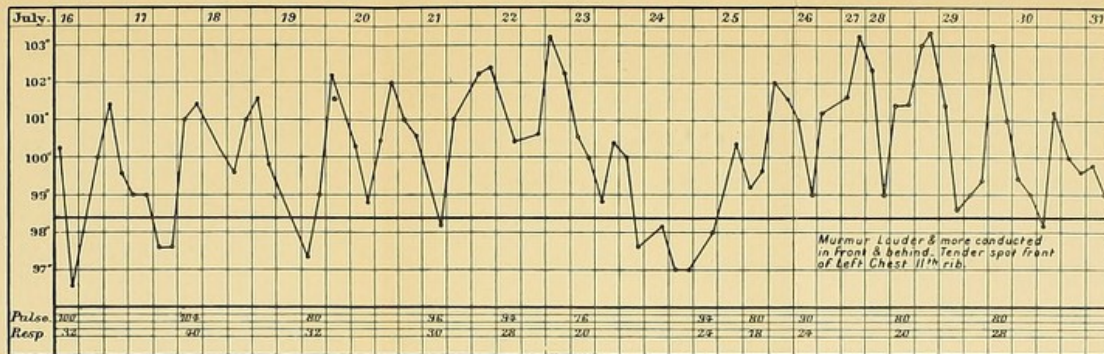
Chart illustrating the temperature of a case of ulcerative endocarditis. Between the dates July 26th and July 30th is a well-marked embolic rise of temperature.
