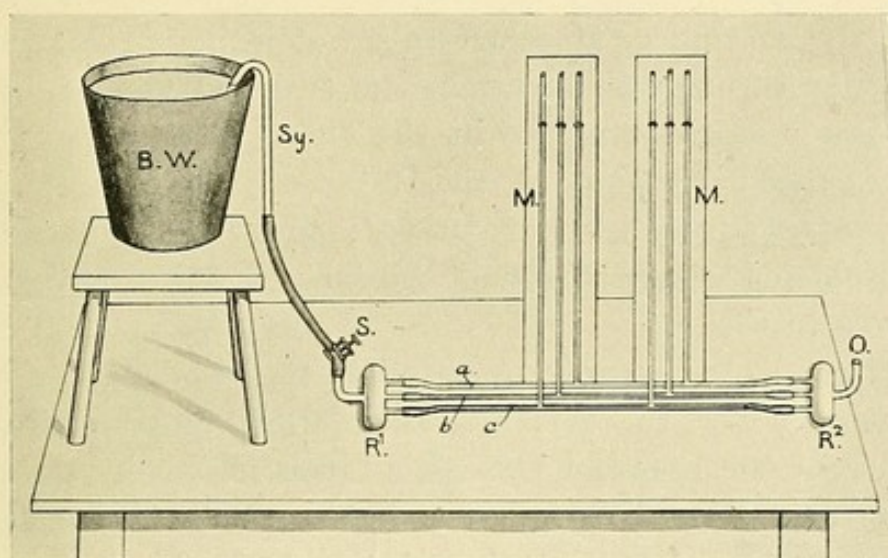
FIG. 19.—Schema of the circulation devised by Dr. Cargill Knott and the author; description in text. The thick tubes between tubes a , b , c and R¹ and R² are omitted from the figure.
