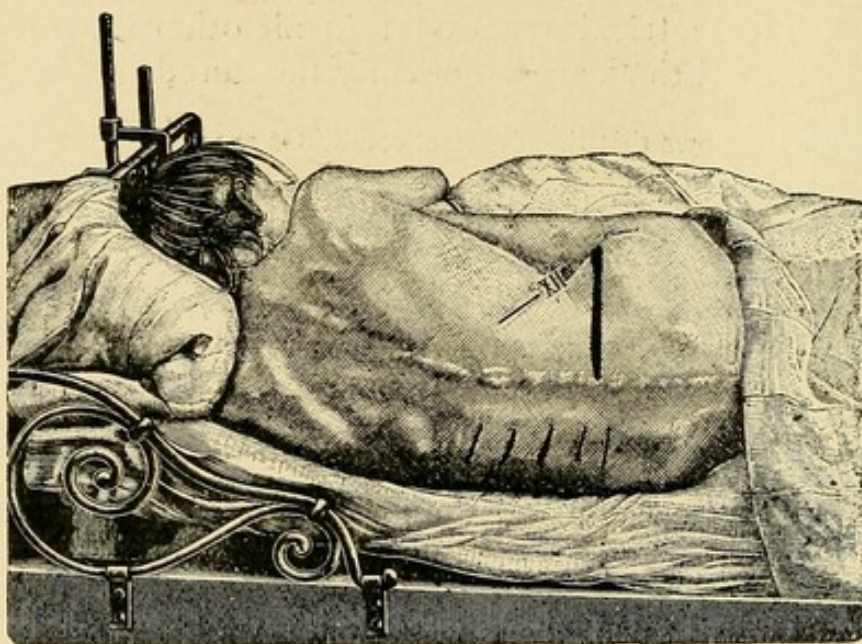
FIG. 38. (After Quincke.)
