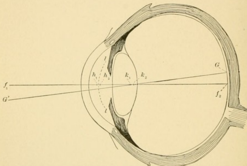
FIG. 28.—CARDINAL POINTS OF THE EYE (see text).
