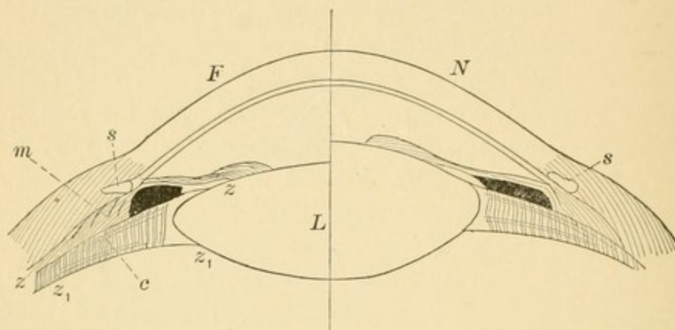
FIG. 30.—CHANGES IN THE LENS DURING ACCOMMODATION. (After Helmholtz.)
