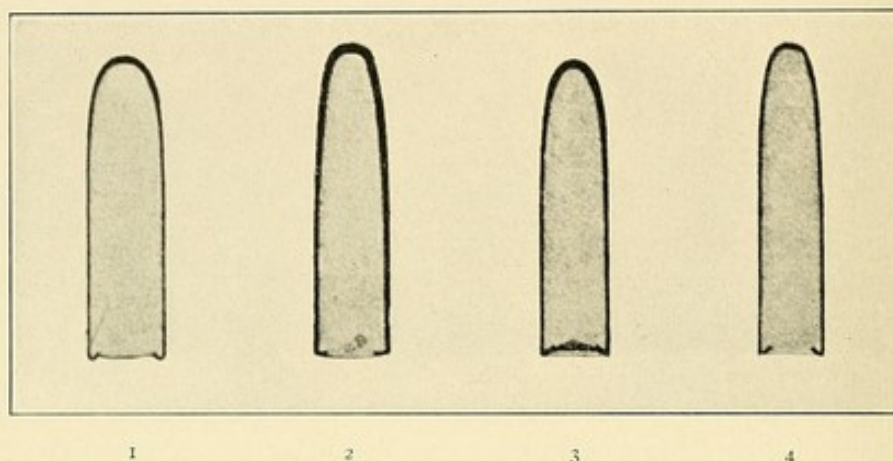
Fig. 590.—Sections of bullets to show relative shape and thickness of mantles: 1, Geudes: regular dome-shaped tip; mild steel mantle; thickness at tip, 0.8 mm.; at sides of body, 0.3 mm.; 2, Lee- Metford : ogival tip; cupro-nickel mantle; thickness at tip, 0.8 mm.; gradual decrease at sides to 0.4 mm.; 3, Mausers : pointed dome tip; steel mantle plated with copper alloy; thickness at tip, 0.8 mm.; gradual decrease at sides to 0.4 mm.; 4, Krag-Jørgensen : ogival tip as in Lee- Metford ; steel mantle plated with cupro-nickel; thickness at tip, 0.6 mm.; gradual decrease at sides to 0.4 mm. Note the more gradual thinning in the Lee- Metford (from Makins ' "Surgical Experiences," etc.).
