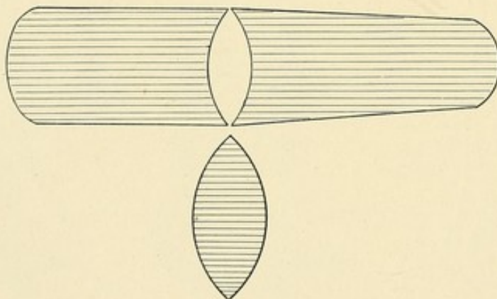
Fig. 232.—Patterns of pieces used in making the usual (soldered) internal right-angle splint, seen applied in figure 242.
