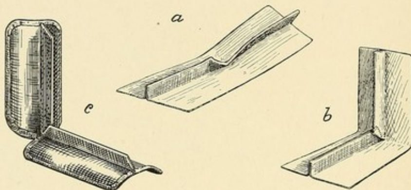
Fig. 231.—Method of manufacture of tin internal right-angle splint: a , Form into which piece of tin is folded (with vise and hammer); b shows the bend in the back ridge completed (bent with pliers, hammered close in the vise); c , the completed splint with edges shaped and covered with adhesive plaster, and with the surfaces of the splint properly concaved.
