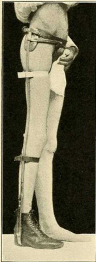
Fig. 435.—Fracture of the thigh. Convalescent ambulatory splint without traction.
