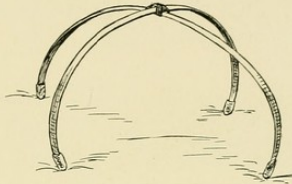
Fig. 405.—Cradle to keep clothes from leg. Made from two barrel-hoops.
