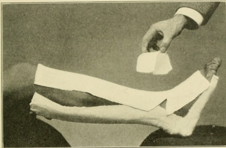
Fig. 630.—Anterior and posterior leg splints applied. Note application of the half cuff of plaster to reinforce the ankle.
