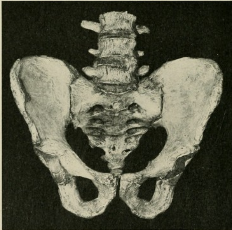
Fig. 106.—Normal pelvis. Note relations of pelvic ring.
