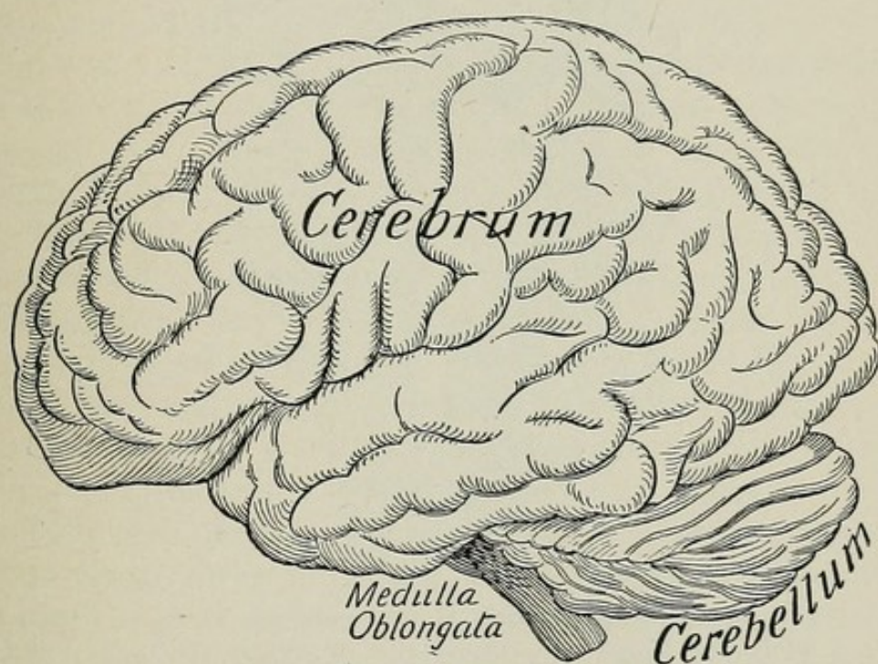
Fig. 13.—The human brain, from the left (Morrow).
