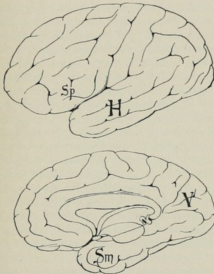
Fig. 23.—The upper figure represents the left hemisphere from outside, that is, from the left. The lower figure shows the internal or mesial aspect of the right hemisphere, that is, the right hemisphere from the left side. Areas usually claimed to possess special relations are marked as follows: H , hearing; V , vision; Sm , smell; Sp , speech.
