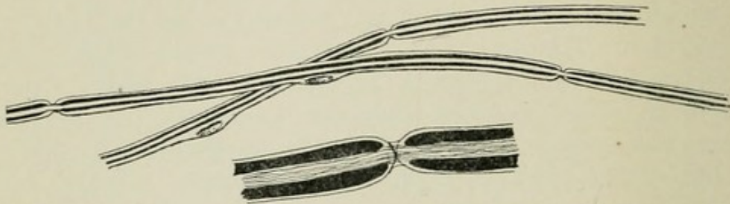
Fig. 3.—Two nerve-fibers shown diagrammatically especially to emphasize the continuity of the axon. A detail, further enlarged, to suggest fibrils in the axon.
