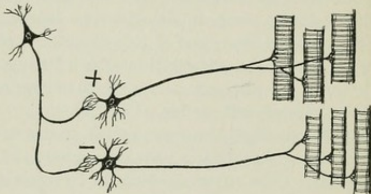
Fig. 18.—The principle of reciprocal innervation. The cortical neuron is represented as exciting the upper of the two subordinate neurons, causing the contraction of one group of muscle-fibers, while it inhibits the second neuron, allowing the associated muscle-fibers to relax. The + sign suggests stimulation; the — sign, inhibition. Doubtless the actual arrangement is less simple than this.
