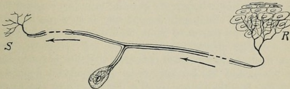
Fig. 6.—To show how in an afferent neuron the transmission is from the endings subject to stimulation ( R ) to a synapse ( S ) in the central nervous system. The perikaryon has an intermediate position and its functions other than that of maintenance are problematic.
