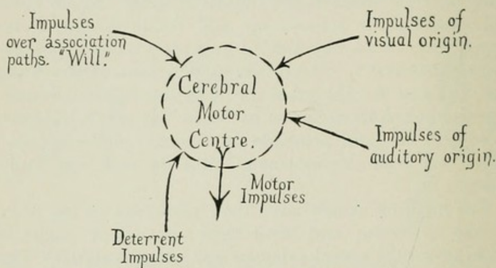
Fig. 20.—To suggest, though incompletely, the concentration of certain streams of impulses upon the motor cortex in one tired by prolonged exertion. To bring in play a fresh path of approach is to secure some renewal of activity. To abate the deterrent impulses has a like effect.
