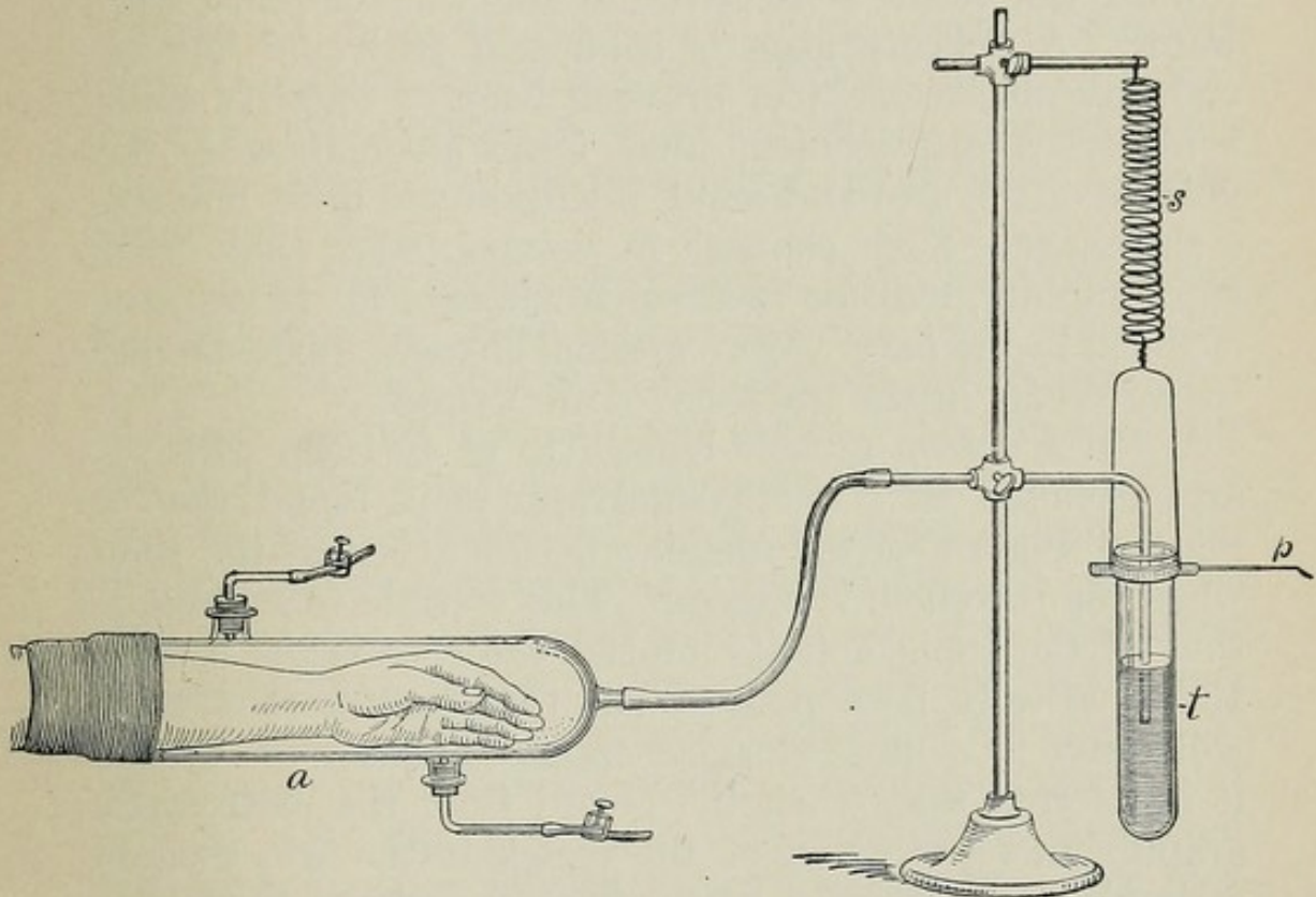
Fig. 24.—A schematic diagram of Mosso's plethysmograph for the arms: a , The glass cylinder for the arm, with rubber sleeve and two tubulatures for filling with warm water; s , the spiral spring swinging the test-tube, t . The spring is so calibrated that the level of the liquid in the test-tube above the arm remains unchanged as the tube is filled and emptied. The movements of the tube are recorded on a drum by the writing point, p . (Howell.)
