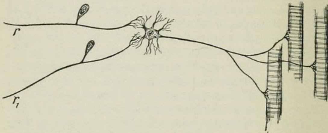
Fig. 19.—The principle of fatigue in reflex action—Forbes' conception. When the reflex obtained through r fails, the action can be renewed by shifting stimulation to r 1 . The motor parts are the same in both cases, hence the fatigue is in a route of approach to the center. One must, in imagination, multiply all the elements illustrated.
