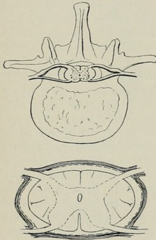
Fig. 10.—The upper figure shows the spinal cord within the arch of a vertebra. A pair of spinal nerves is shown, each nerve having a dorsal and a ventral root.
