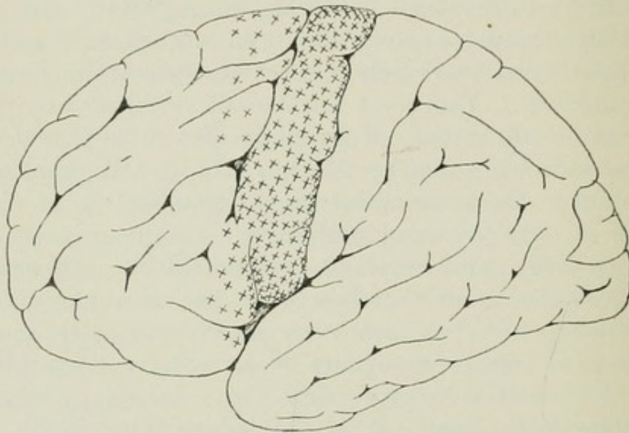
Fig. 22.—The human cerebrum is sketched from the left side. The crosses are sprinkled on the area from which the muscles of the right half of the body appear to be governed. This area extends out of sight over the top of the brain and dips into the fissure between the two hemispheres.
