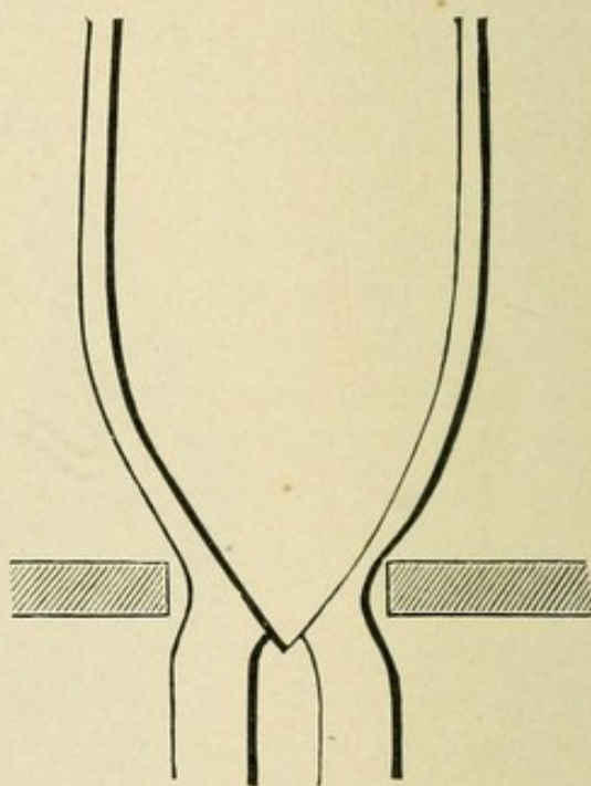
Fig. 28 (b).—Injection under greater pressure; the passage is free.
