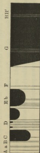
Spectrum of five-banded hematine.
