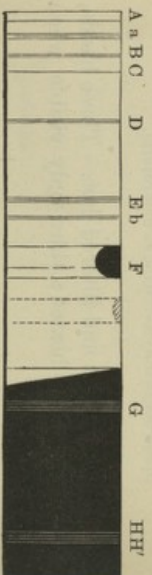
Spectrum of sero-luteine.
