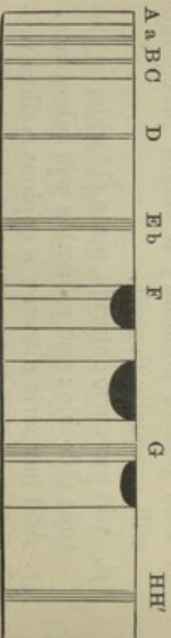
Spectrum of ether solution of corpus luteum.
