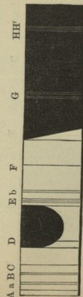
Spectrum of reduced HematocrySTALLINE.
