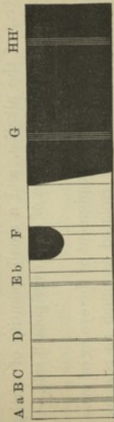
Spectrum of intestino-luteine.
