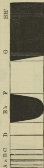
Spectrum of juice of corpora lutea treated with sulphuric acid.
