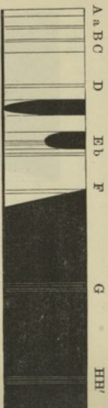
Spectrum of reduced hematine.
