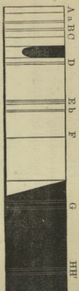
Spectrum of Chologyanine.
