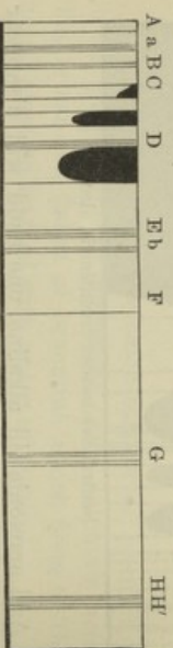
Hydrochloric product of fluorescent creuntine.
