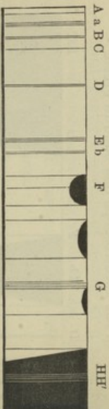
Spectrum of ovario-luteine in alcohol.
