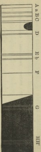
Spectrum of Chologyanine dissolved in water.
