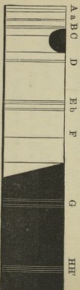
Spectrum of choleraic urobiline.
