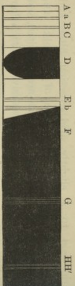
Spectrum of pure alkaline hematine.
