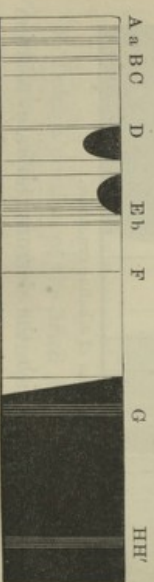
Spectrum of creuntine hydrochlorate.
