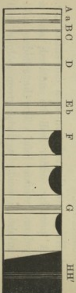
Spectrum of egg luteine in ether.
