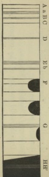
Spectrum of egg luteine in alcohol, cold.
