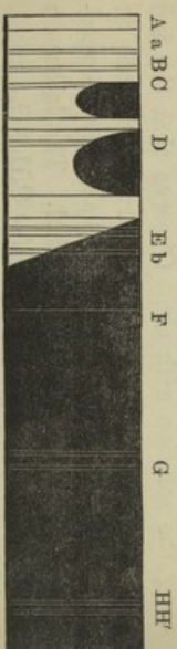
Spectrum of soluble Cholothalline.
