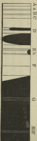
Spectrum of sulphate of creuntine.
