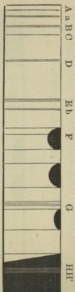
Spectrum of egg luteine in alcohol, hot.
