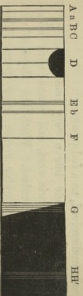
Spectrum of Pettenkofer's test.
