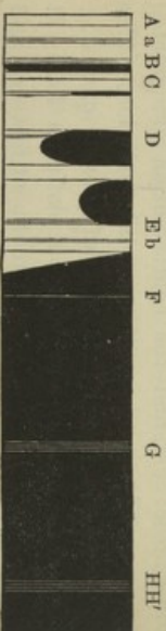
Spectrum of fluopitine.
