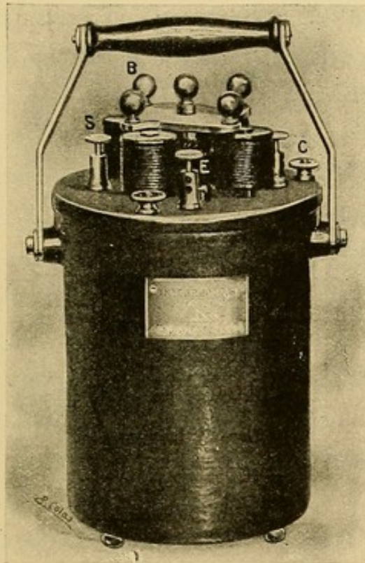
FIG. 12.—AUTOME INTERRUPTER.
