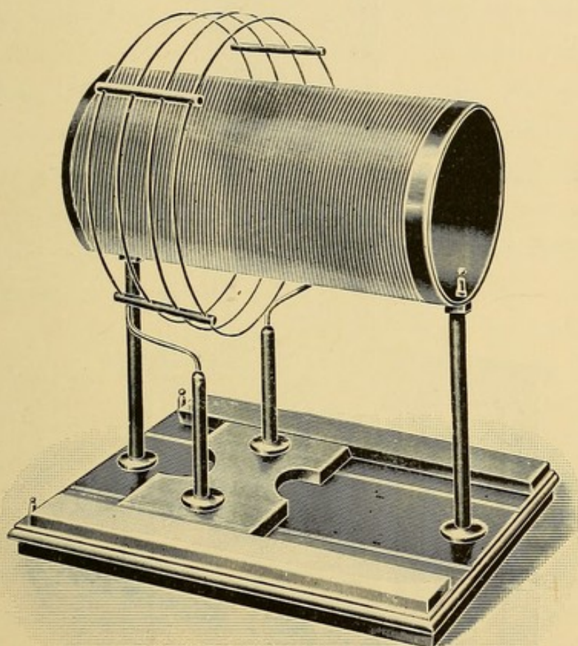
FIG. 29.—D'ARSONVAL RESONATOR.
