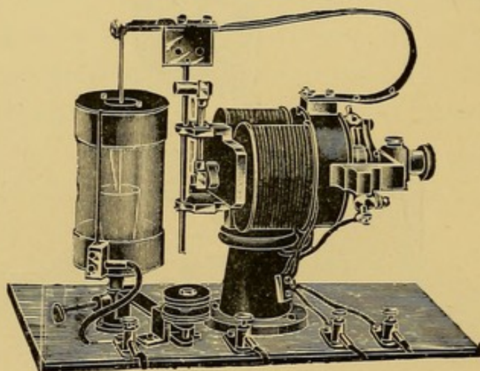
FIG. 15.—DIPPER INTERRUPTER.
