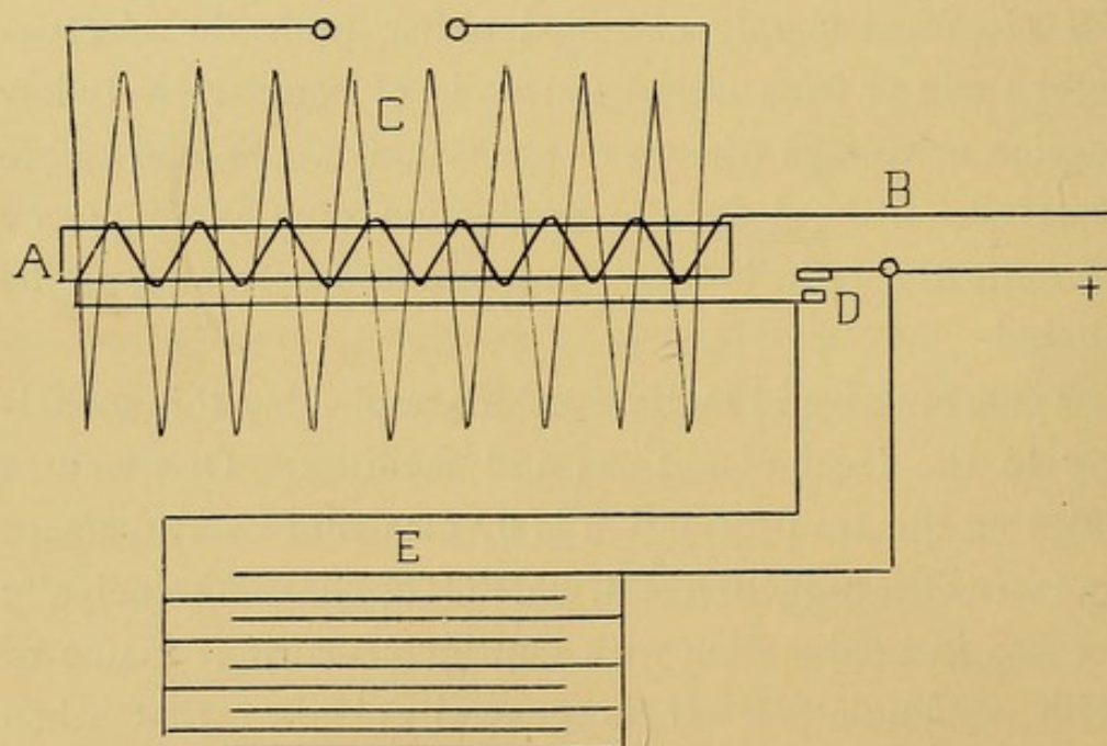
FIG. 5.—DIAGRAM OF AN INDUCTION COIL.
