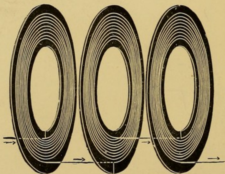
FIG. 8.—DIAGRAM OF JOINTLESS SECTION-WINDING.
