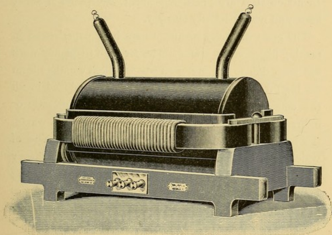
FIG. 20.—HIGH-TENSION TRANSFORMER.
