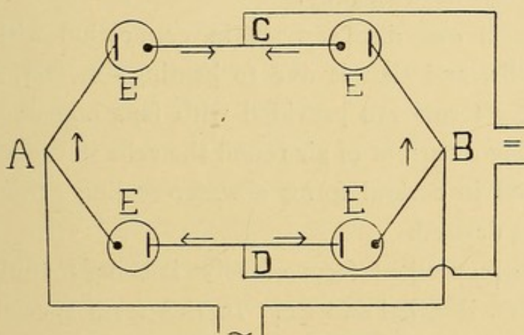
FIG. 23.—DIAGRAM OF NODON VALVE.
