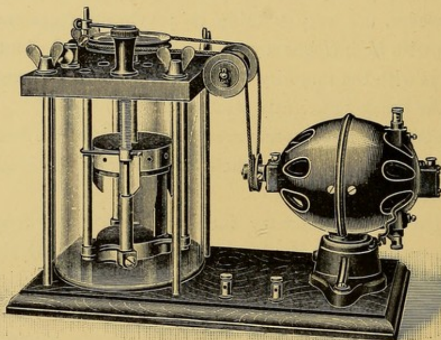
FIG. 11.—TURBINIA JET INTERRUPTER.
