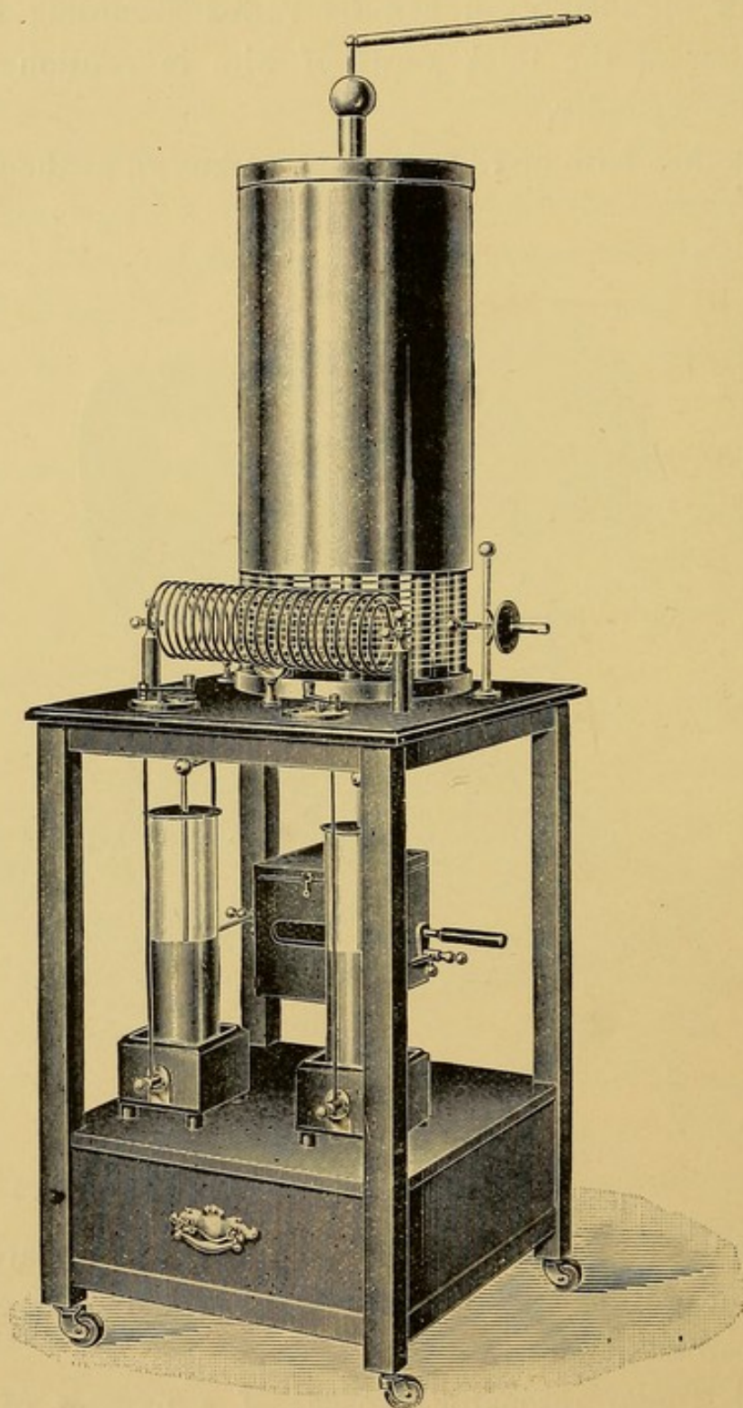
FIG 30.—COMPLETE HIGH FREQUENCY APPARATUS.
