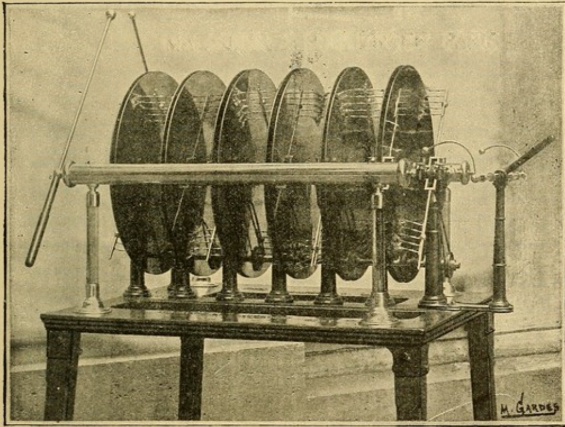
FIG. 25 —EBONITE PLATE WIMSHURST MACHINE.
