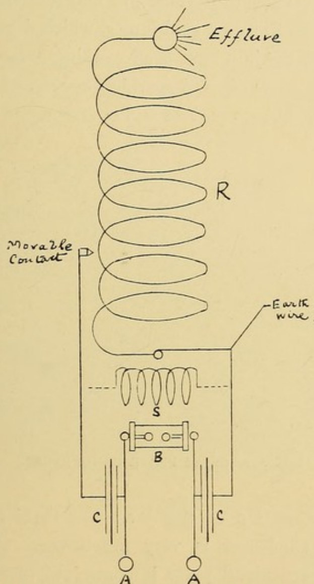
FIG. 26.—DIAGRAM OF HIGH FREQUENCY APPARATUS.
