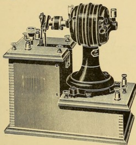
FIG. 16.—DOUBLE-DIPPER INTERRUPTER.
