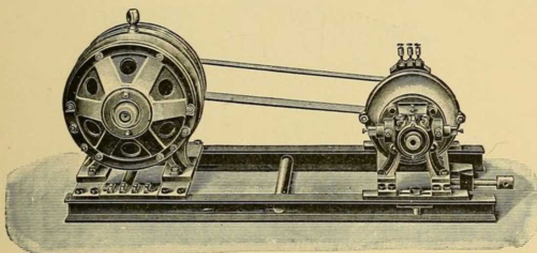
FIG. 21.—ALTERNATING CONTINUOUS MOTOR CONVERTER.
