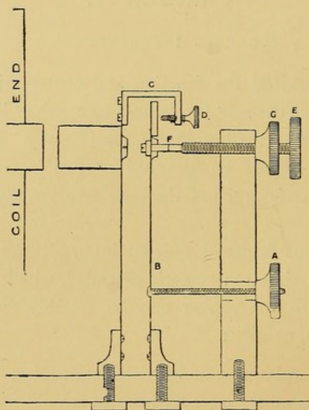
FIG. 10.—PLATINUM INTERRUPTER.
