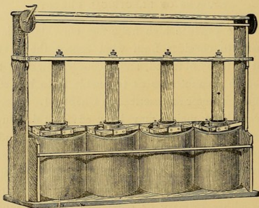
FIG. 2.—PRIMARY BATTERY.
