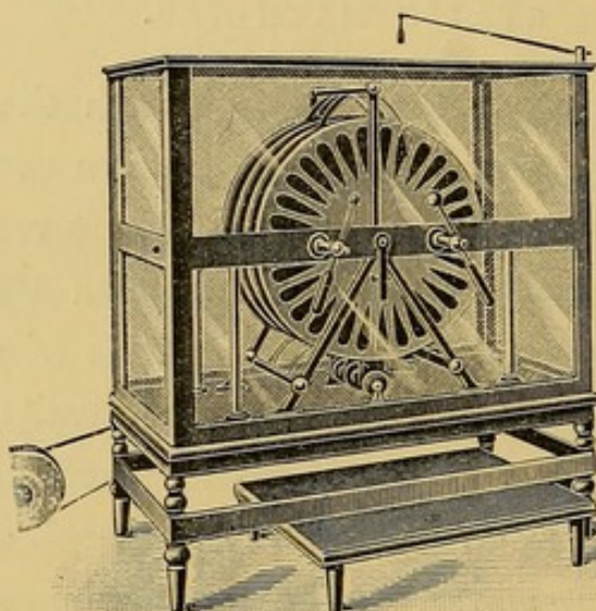
FIG. 24.—GLASS PLATE WIMSHURST MACHINE.
