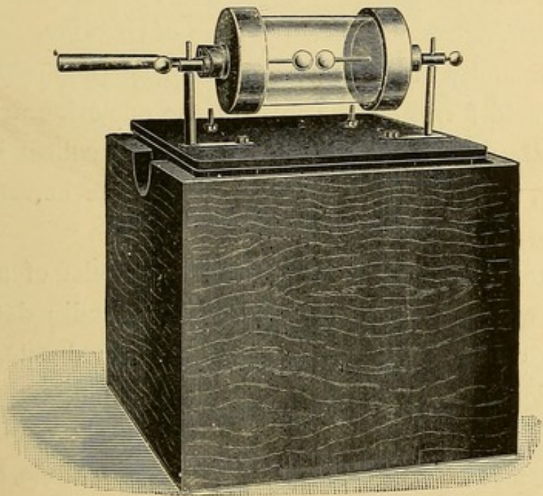
FIG. 28.—HIGH FREQUENCY OIL CONDENSER.
