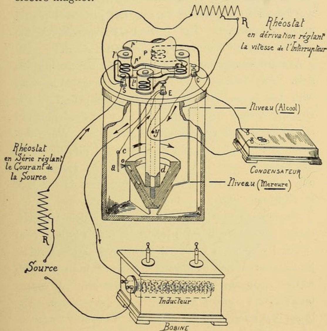
FIG. 13.—DIAGRAM OF AUTONOME INTERRUPTER.
