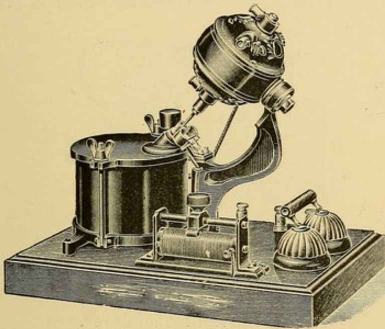
FIG. 14.—MACKENZIE DAVIDSON INTERRUPTER.
