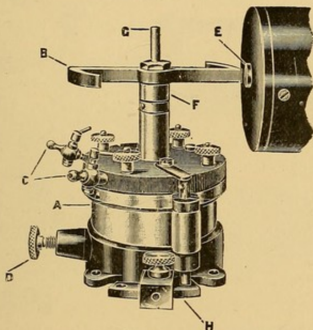
FIG. 9.—MOTO-MAGNETIC INTERRUPTER.
