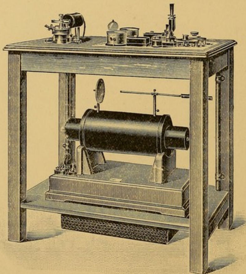
FIG. 18.—SWITCH-TABLE, WITH INTERRUPTER, COIL, AND RESISTANCE.
