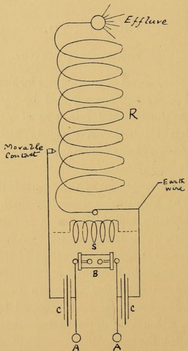
FIG. 30.—DIAGRAM OF HIGH FREQUENCY APPARATUS.
