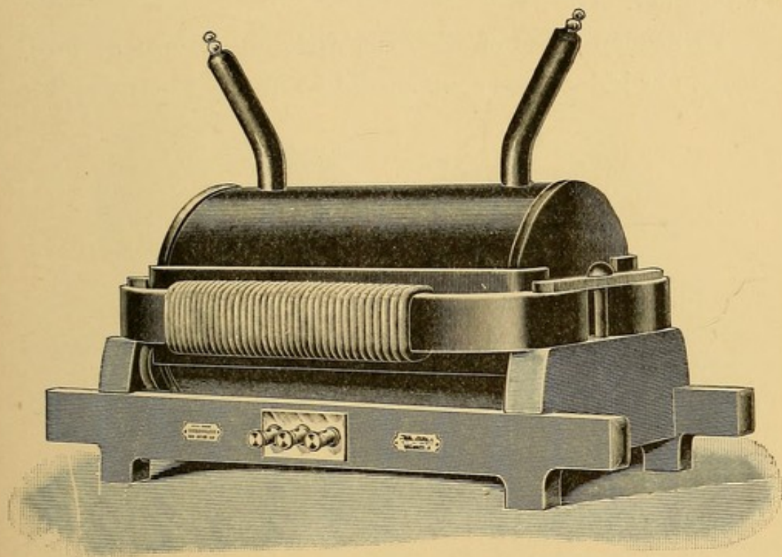
FIG. 20.—HIGH-TENSION TRANSFORMER.
