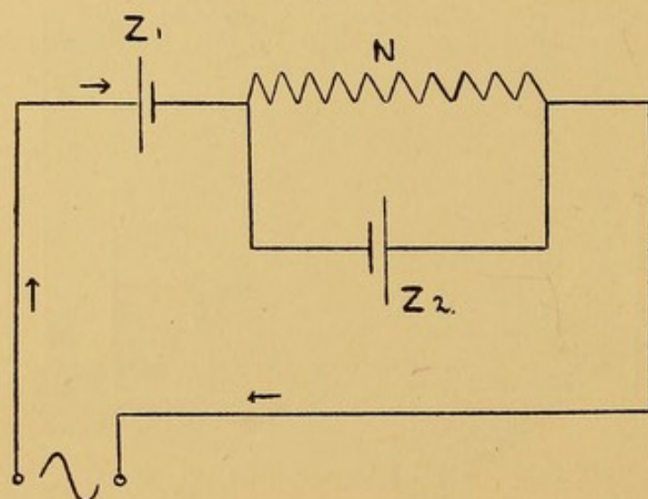
FIG. 25.—DIAGRAM OF SIEMENS' VALVE.
