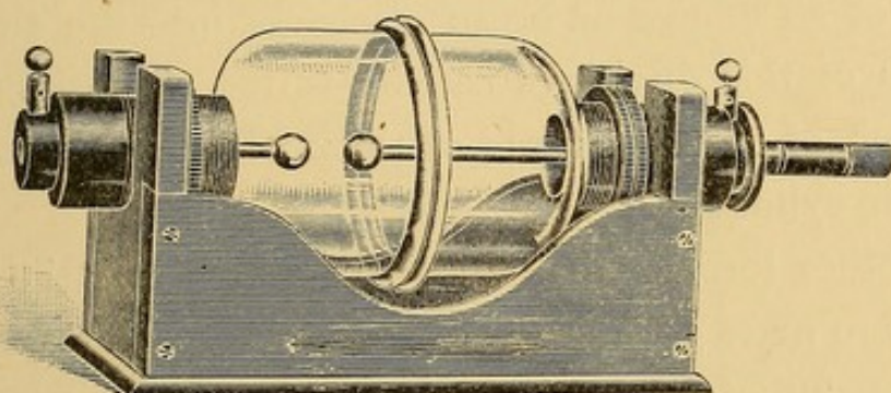
FIG. 33.—HIGH FREQUENCY SPARK-GAP.
