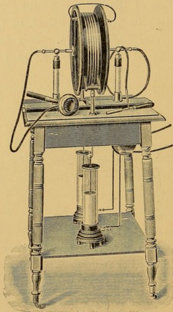
FIG. 36.—ROYCOURT HIGH FREQUENCY APPARATUS.
