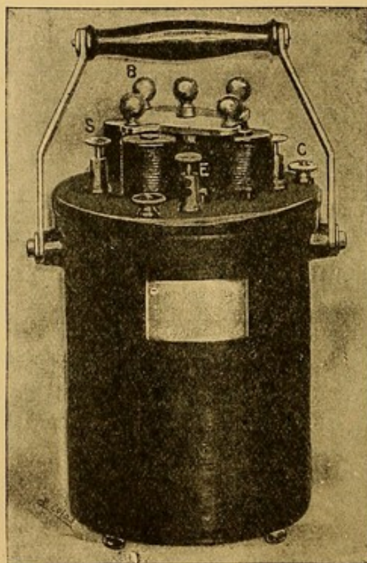
FIG. 11.—AUTONOME INTERRUPTER.
