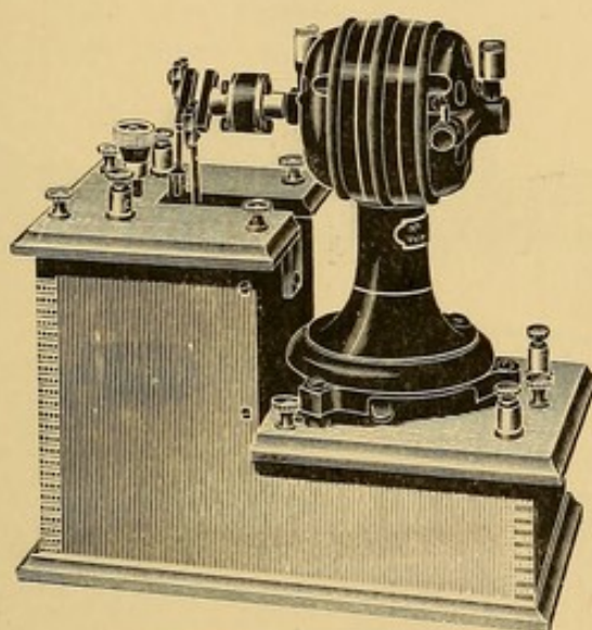
FIG. 13.—DOUBLE-DIPPER INTERRUPTER.
