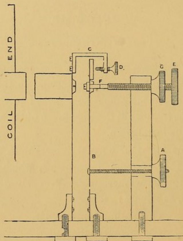
FIG. 8.—PLATINUM INTERRUPTER.
