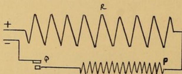
FIG. 15.—SERIES RESISTANCE.
