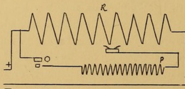
FIG. 16.—SHUNT RESISTANCE.
