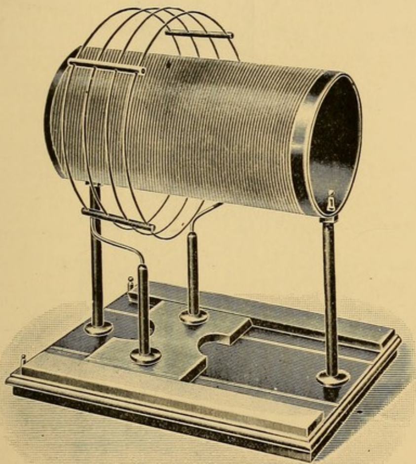
FIG. 34.—D'ARSONVAL RESONATOR.
