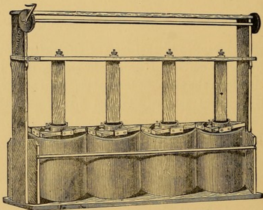
FIG. I.—PRIMARY BATTERY.
