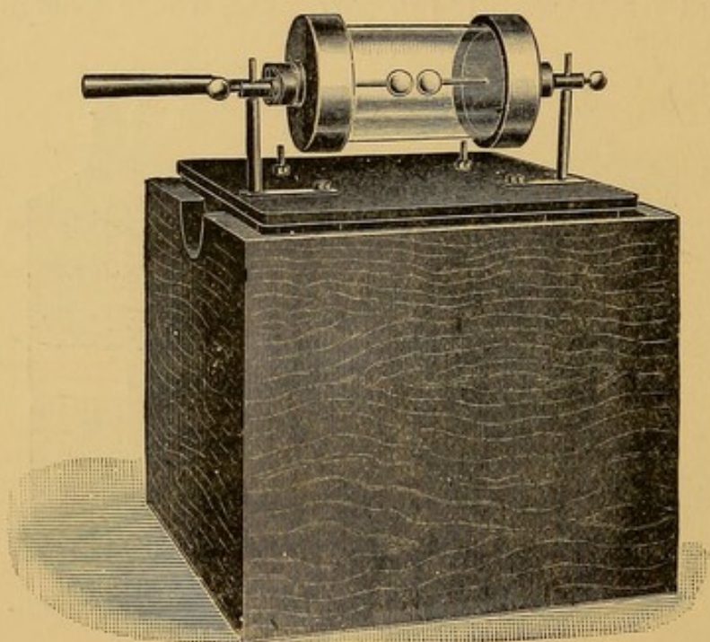
FIG. 32.—HIGH FREQUENCY OIL CONDENSER.
