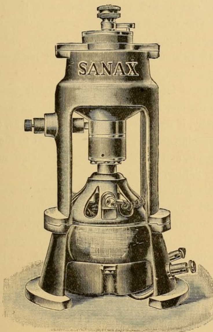
FIG. 12.—SANAX INTERRUPTER.
