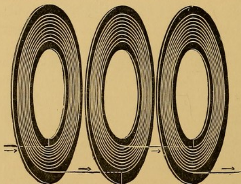
FIG. 7.—DIAGRAM OF JOINTLESS SECTION-WINDING.
