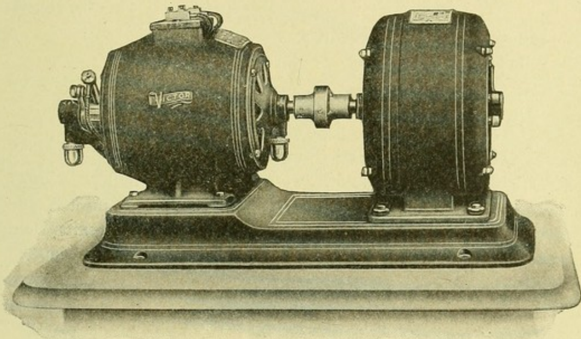
Fig. 8.—Transformer, alternating to direct current. (Victor.)
