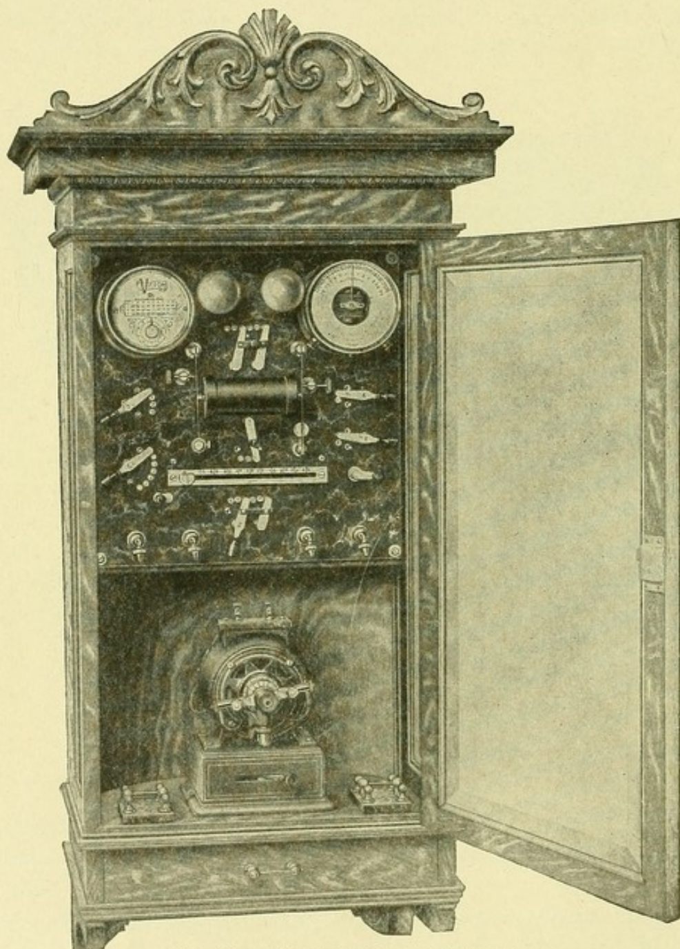
Fig. 7.—Wall cabinet. (Victor.)
