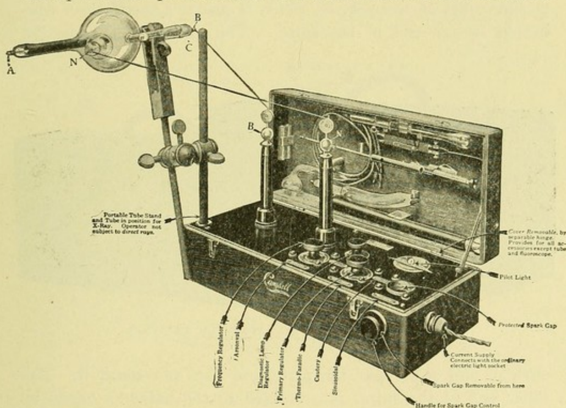
Fig. 74.—Campbell model "E" X-ray and coil.
