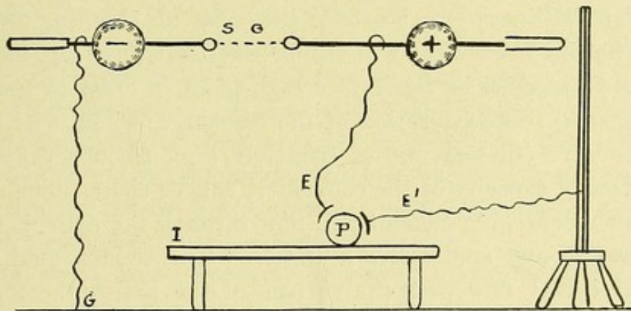
Fig. 42.—The wave-current intensified. (Morton.)
