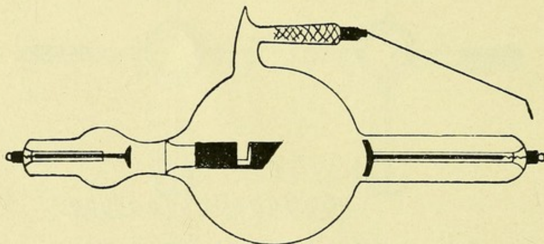
Fig. 66.—Campbell X-ray tube.
