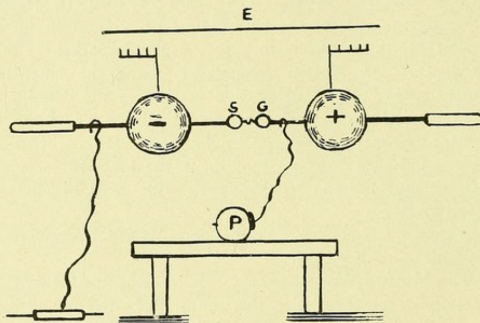
Fig. 41.—Wave-current. (Morton.)
