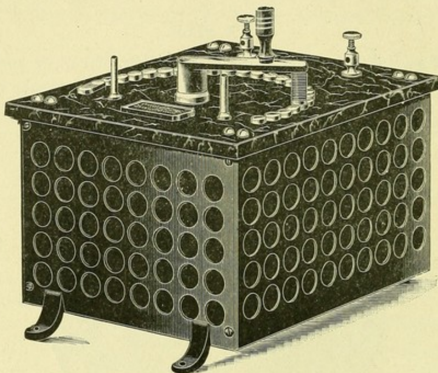
Fig. 11.—Twenty-five point rheostat. (Victor.)
