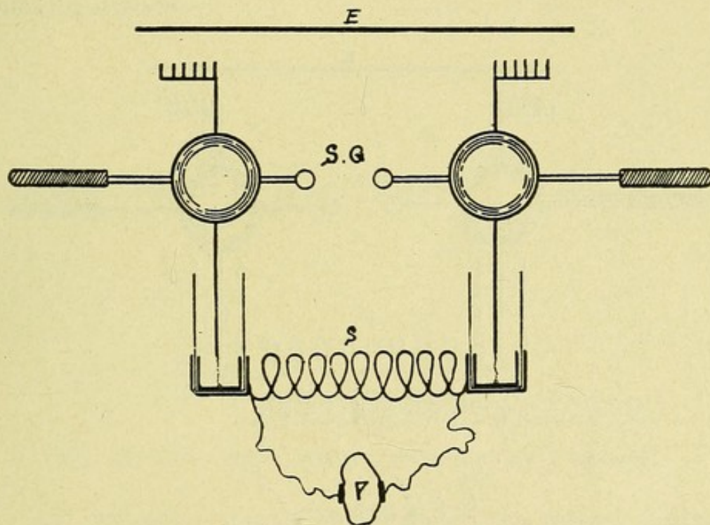
Fig. 63.—Drawing of d'Arsonval apparatus.
