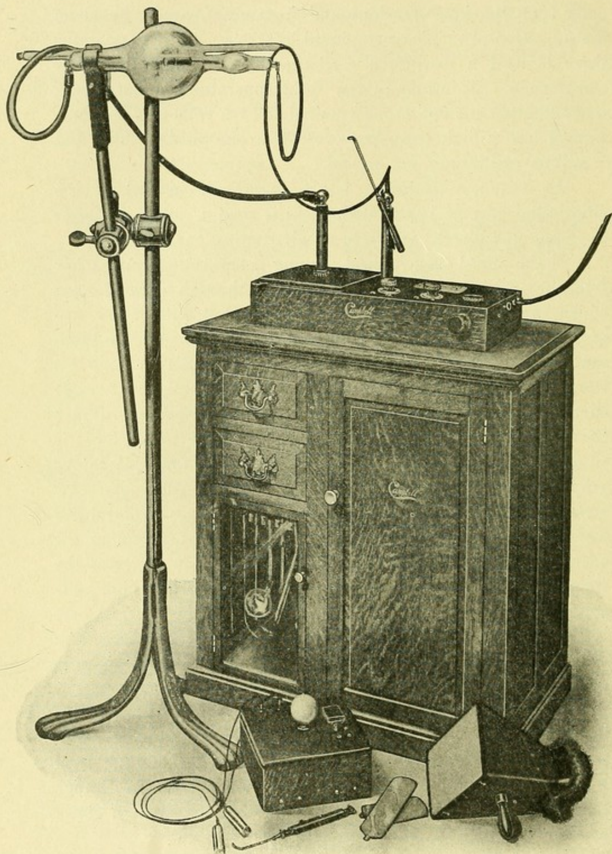
Fig. 71.—Campbell model "D" coil, cabinet and X-ray.
