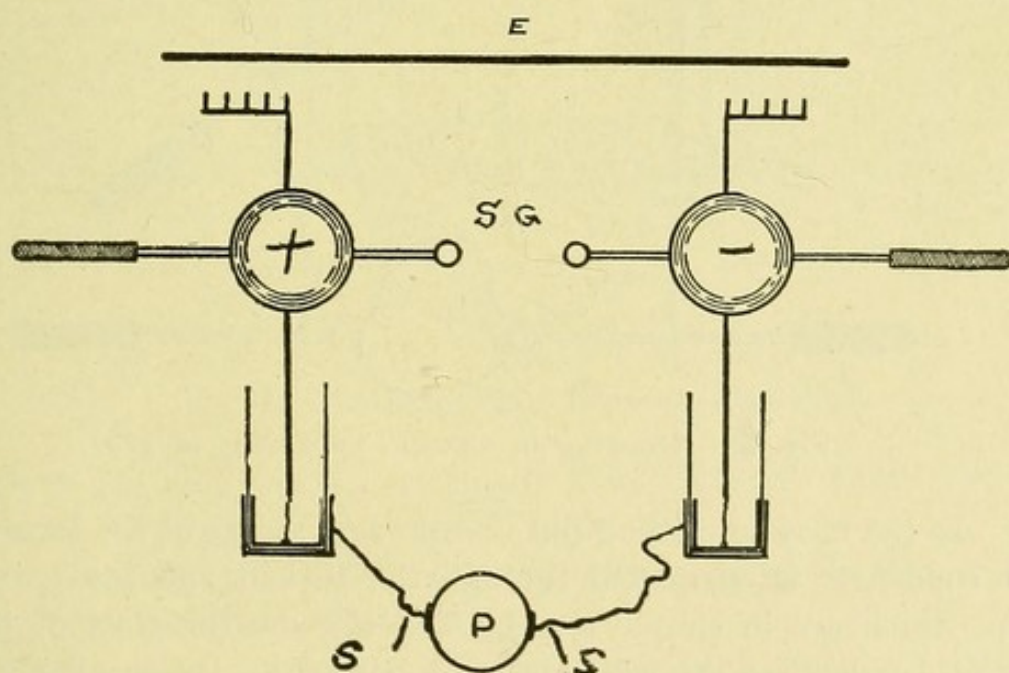
Fig. 61.—Drawing of Morton's static induced current of 1881.
