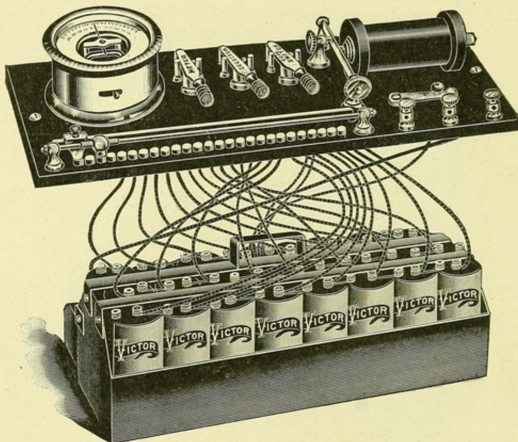
Fig. 5.—Removable tray. (Victor.)
