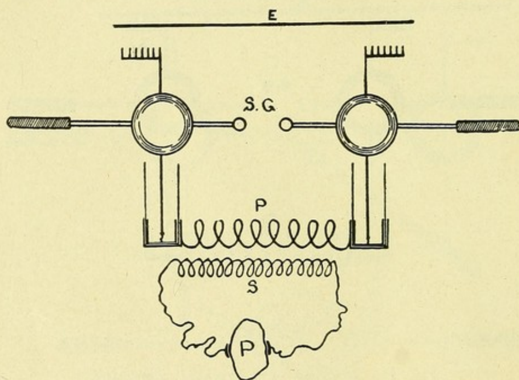
Fig. 64.—Drawing of Tesla apparatus.
