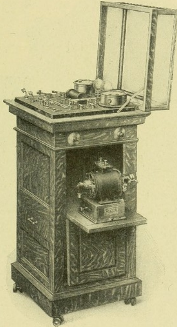
Fig. 6.—Floor cabinet. (Victor.)
