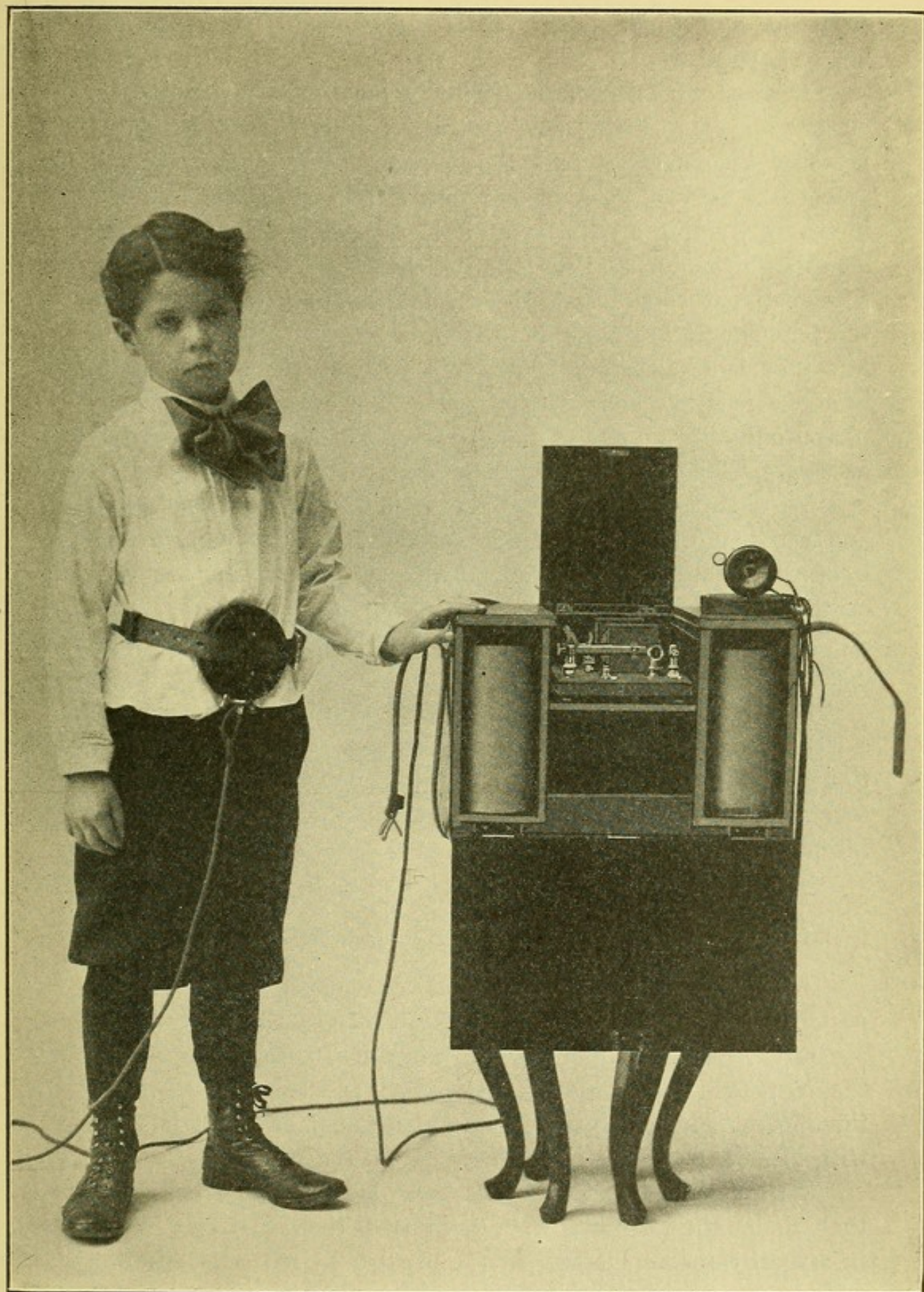
Fig. 81.—Bachelet dry-cell generators.
