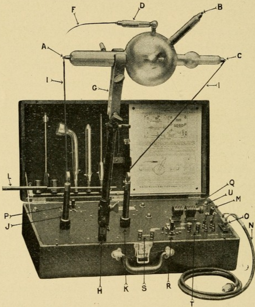
Fig. 39—Portable Coil.
