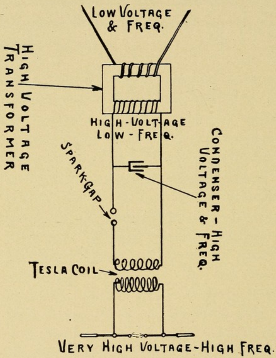
Fig. 14—Diagram of Tesla Type.
