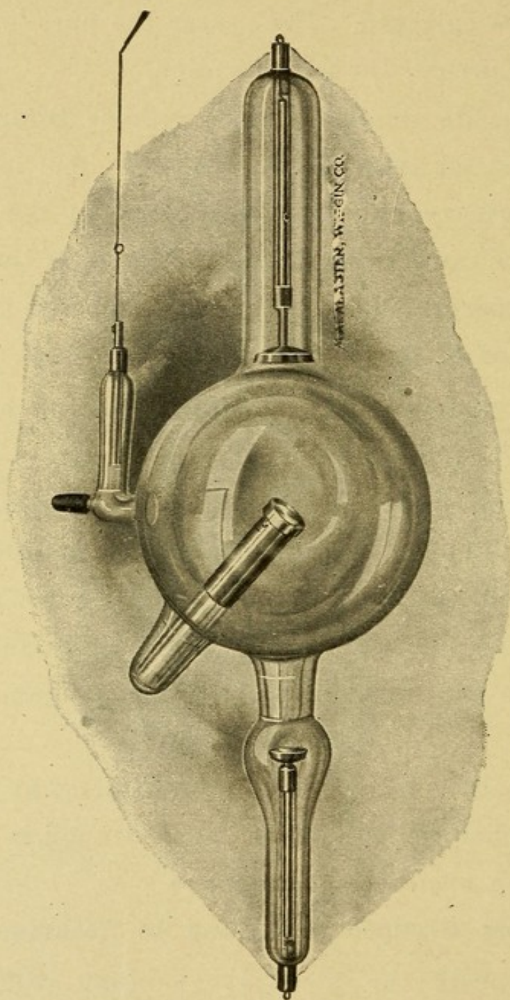
Fig. 62—High Frequency X-ray Tube.
