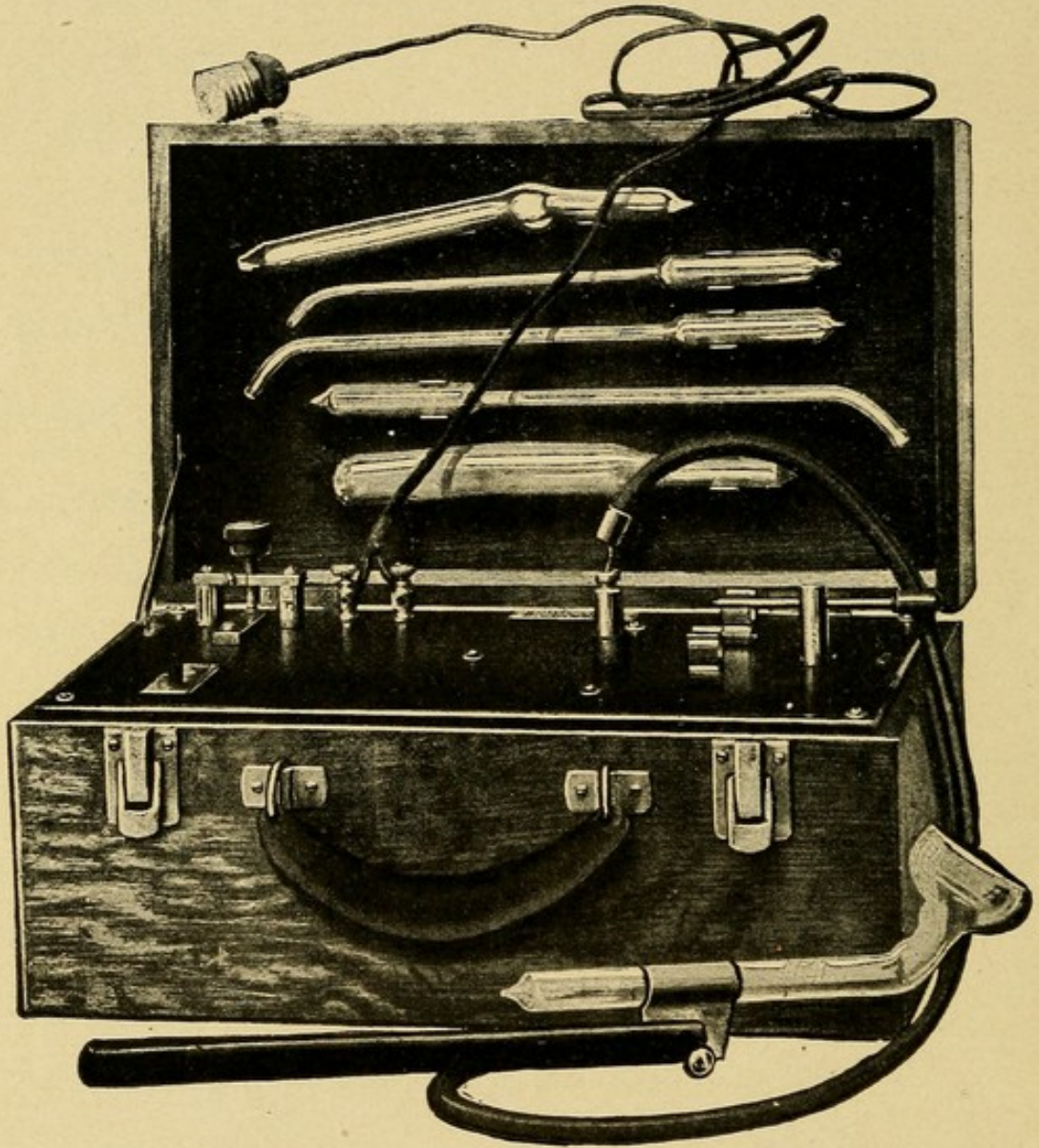
Fig. 2—Portable High Frequency Coil.
