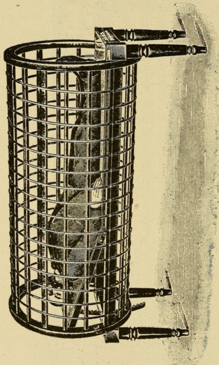
Fig. 35. Horizontal Auto-Conduction Cage.
