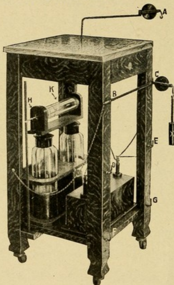
Fig. 25—Resonator for X-ray Coil.
