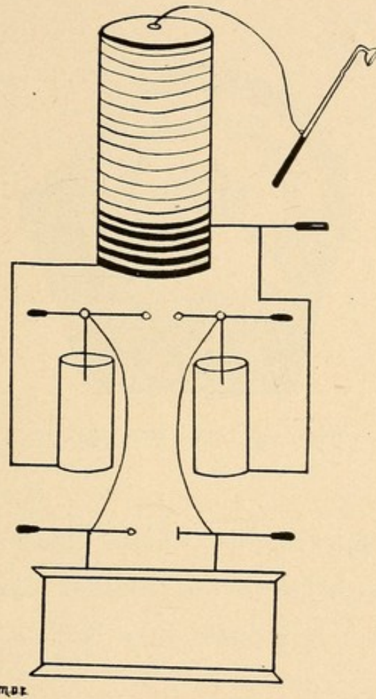
Fig. 15—Diagram of Oudin Resonator.
