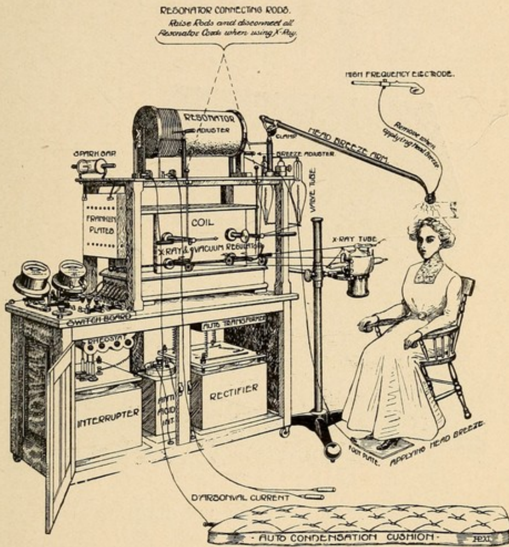
Fig. 18—Illustrating the Various Methods of Administering High Frequency Currents.
