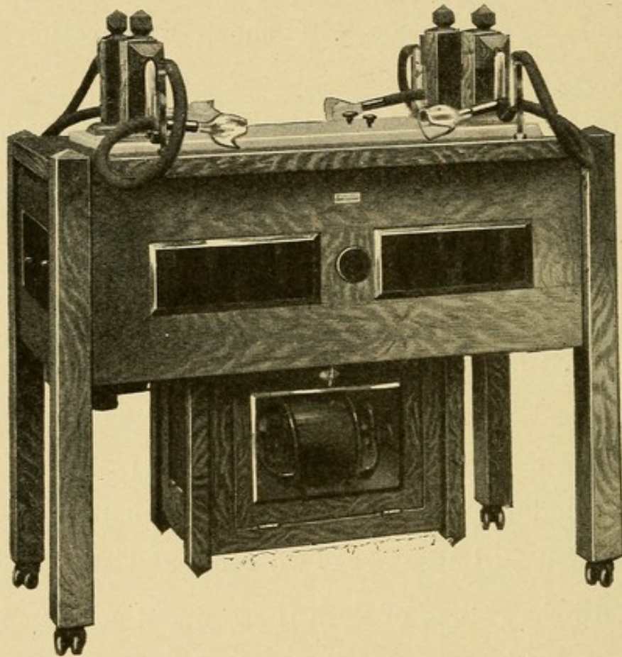
Fig. 57—Ozone Generator for Office Use.
