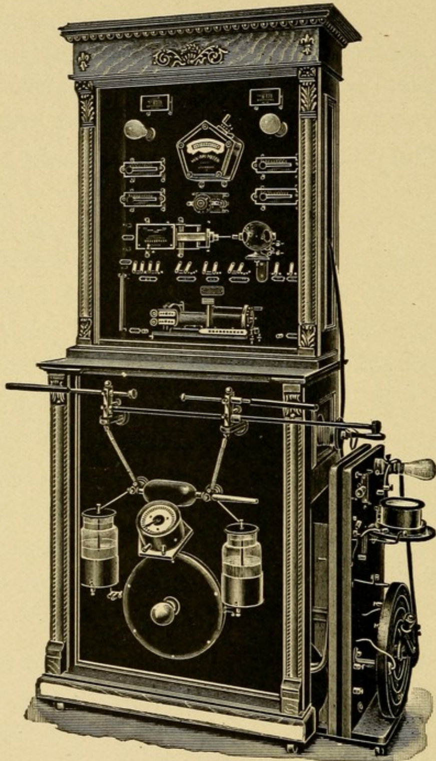
Fig. 10—Large High Frequency Outfit.
