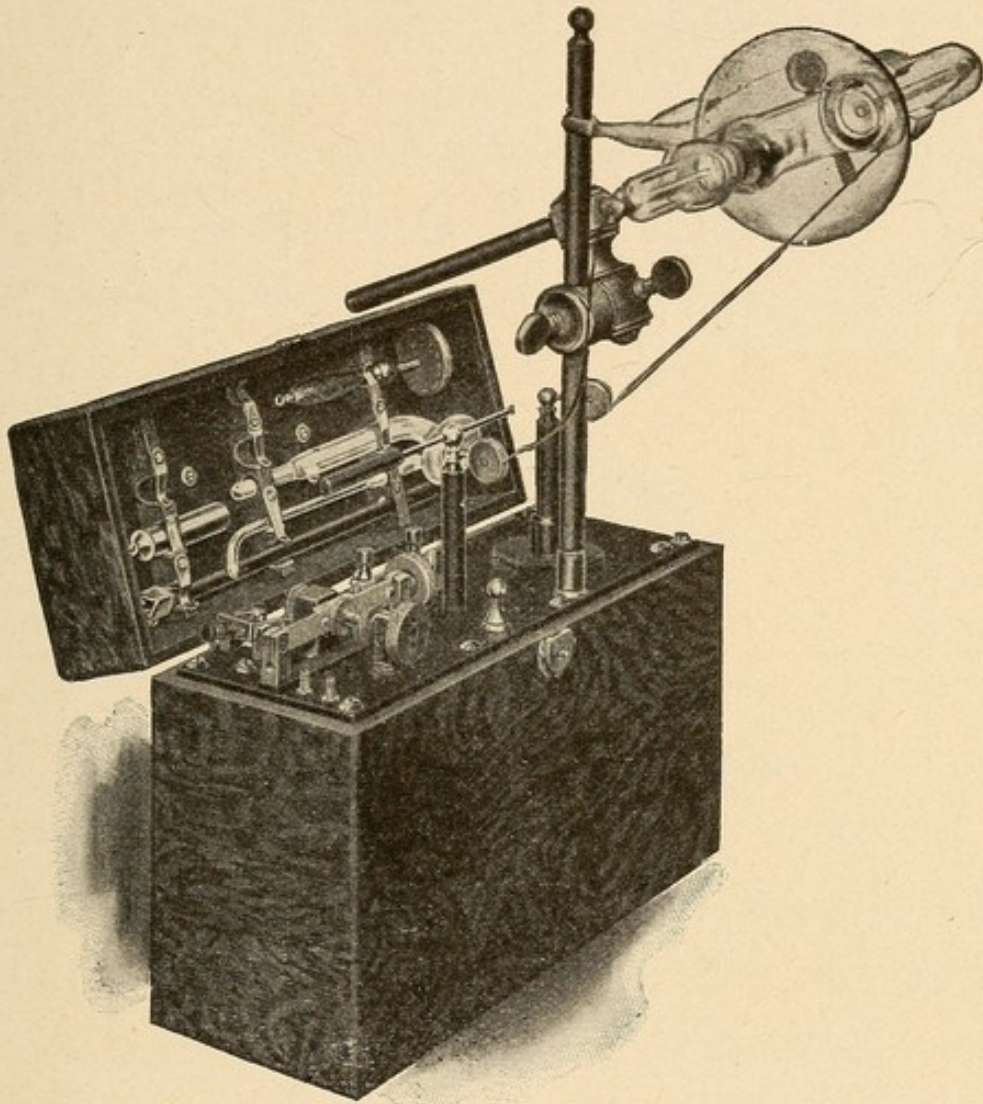
Fig. 40—Portable Coil.
