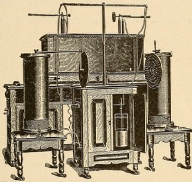
Fig. 30—Double Resonator with Diaphragms.
