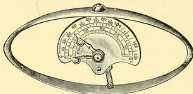
FIG. 31.—Mathieu's Dynamometer.
