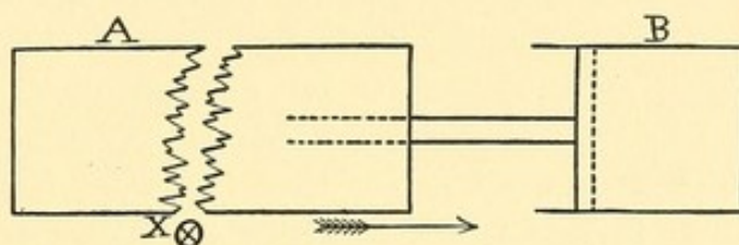
FIG. 22.—A, Hydraulic Cylinder; B, Powder Compressing Chamber.
