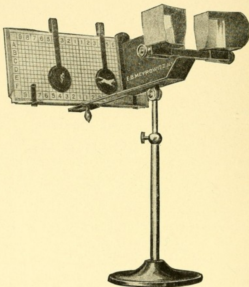
FIG. 35.—Derby's Stereoscope.
